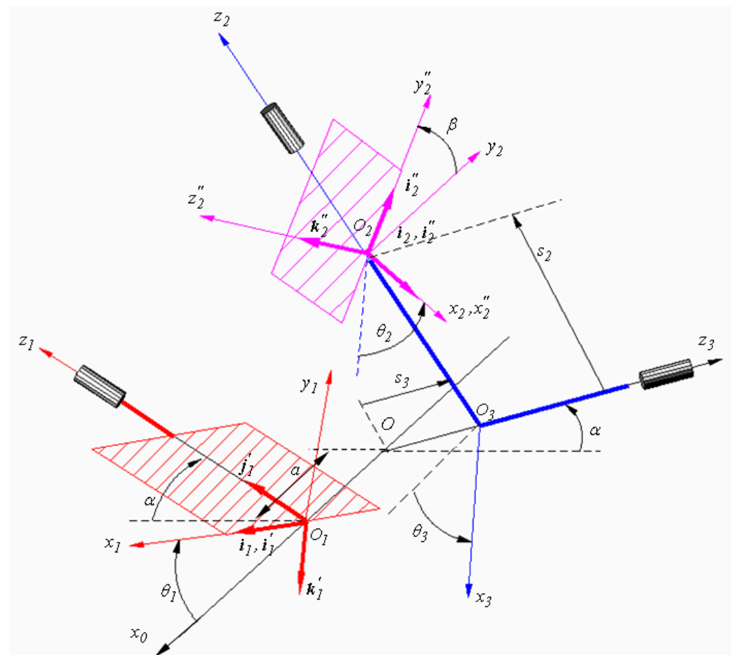
Figure 4. Cartesian reference systems: x_1'y_1'z_1' attached to the driving element, x_2'y_2'z_2' attached to the intermediate element, and x_3'y_3'z_3' attached to the driven element.
