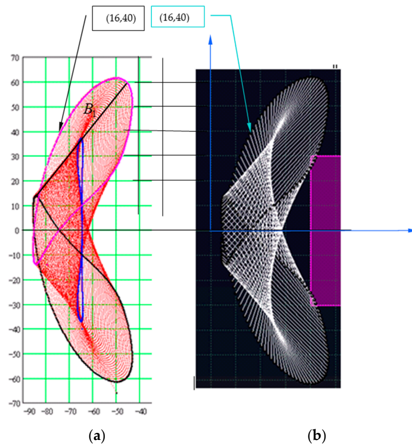
Figure 9. The geometrical loci of a straight line ( B_1 ) attached to element 1, with respect to element 2: (a) analytical and (b) numerical results.
