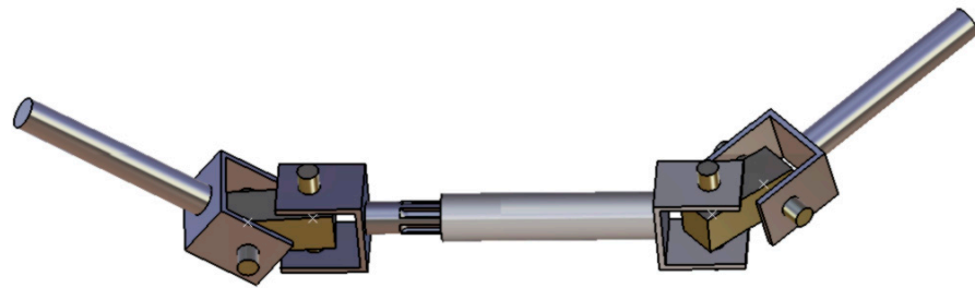
Figure 2. Double Cardan joint.
