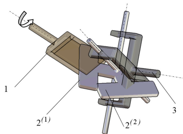
Figure 5. The assemblage possibilities of the mechanism.
