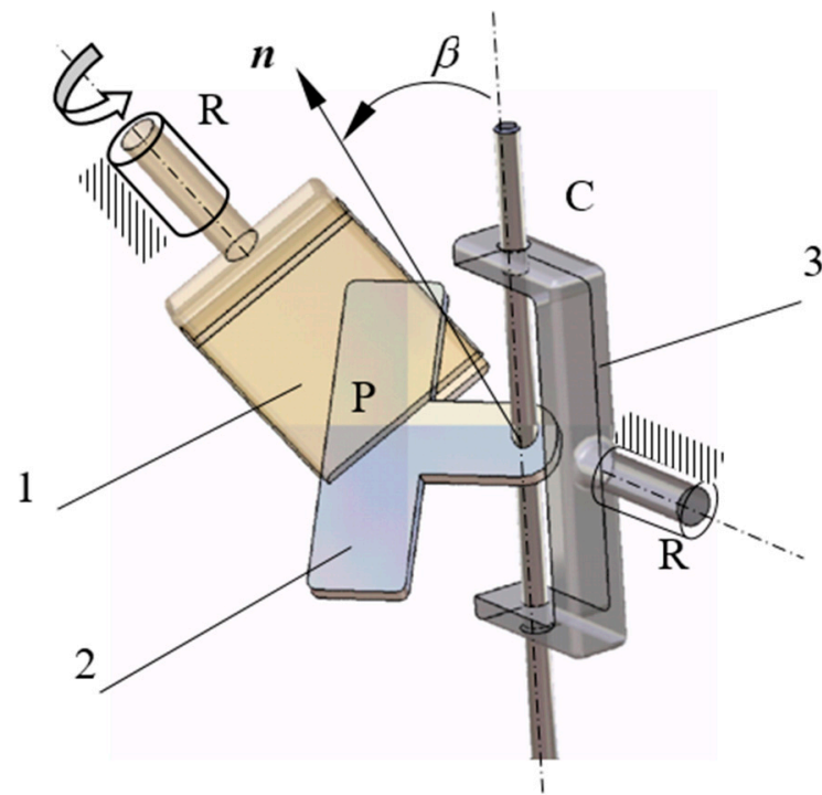
Figure 3. The spatial RPCR mechanism.
