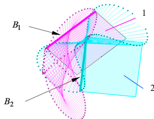
Figure 7. The positions of a line segment attached to a plate with respect to the other one.
