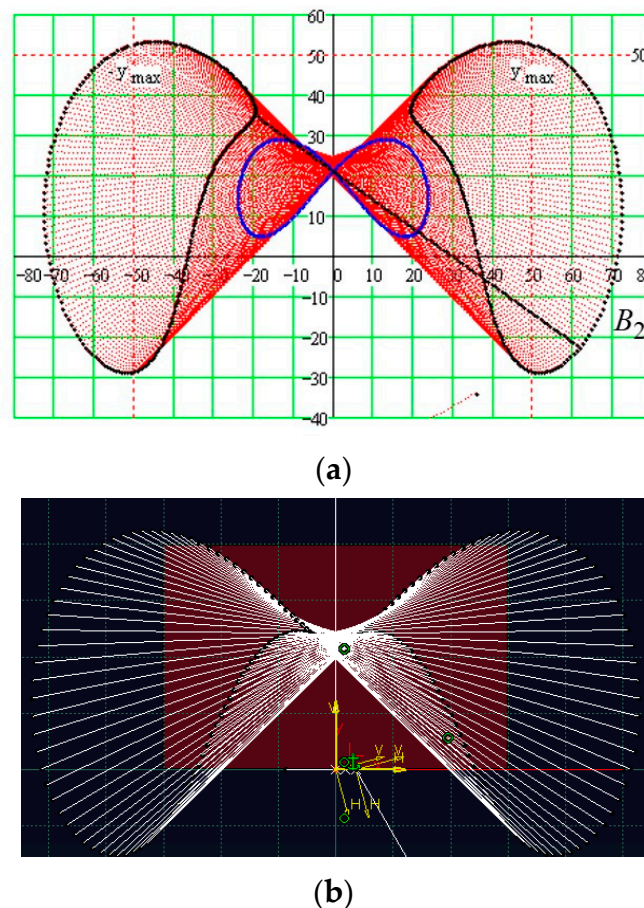
Figure 8. The geometrical loci of a straight line ( B_2 ) attached to element 2 with respect to element 1: (a) analytical and (b) numerical results.
