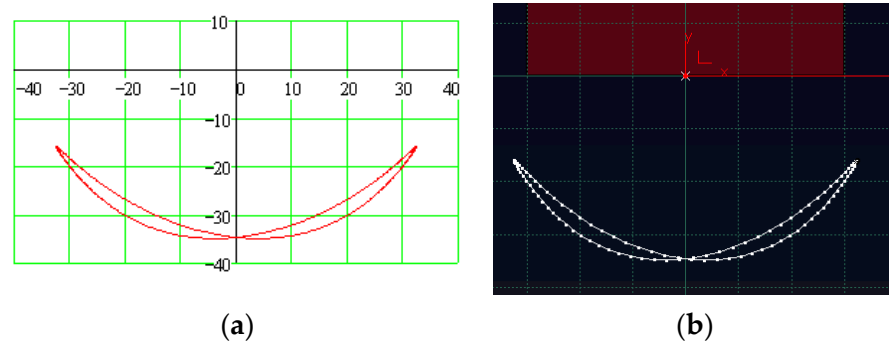
Figure 6. The trajectory of the point O_2 in the frame attached to the driving element: (a) analytical solution and (b) numerical simulation.
