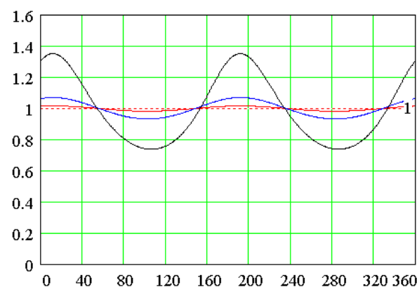
Figure 10. The plots of the transmission ratio \omega_3/\omega_1 for different values of the angle between axes: \pi/36 (red); \pi/18 (blue); and \pi/9 (black).
