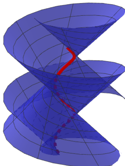
Figure 2. The ruled surface (blue) with the base curve (red).
