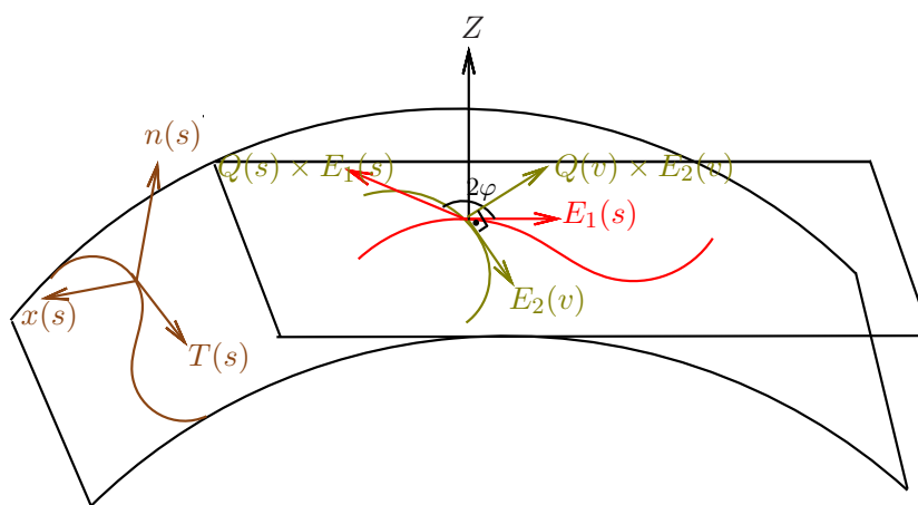
Figure 1. Ruled surface and quaternion shape operators.
