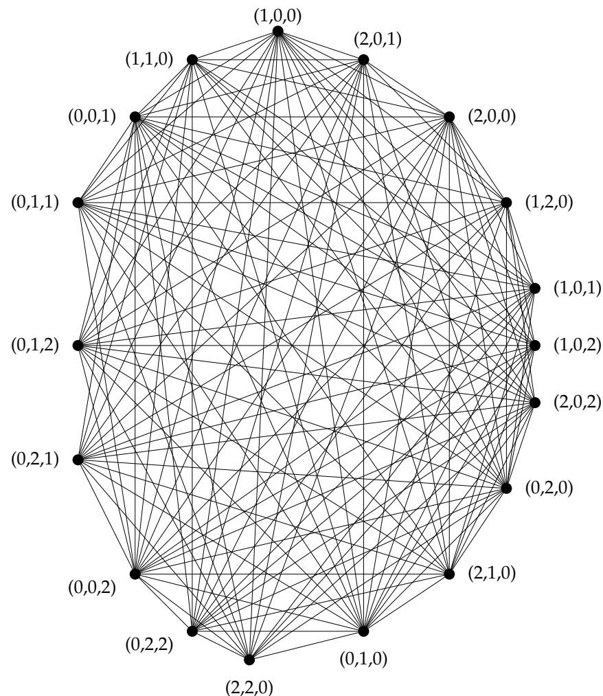
Figure 1. WT(\mathbb{Z}_3 \times \mathbb{Z}_3 \times \mathbb{Z}_3) .
