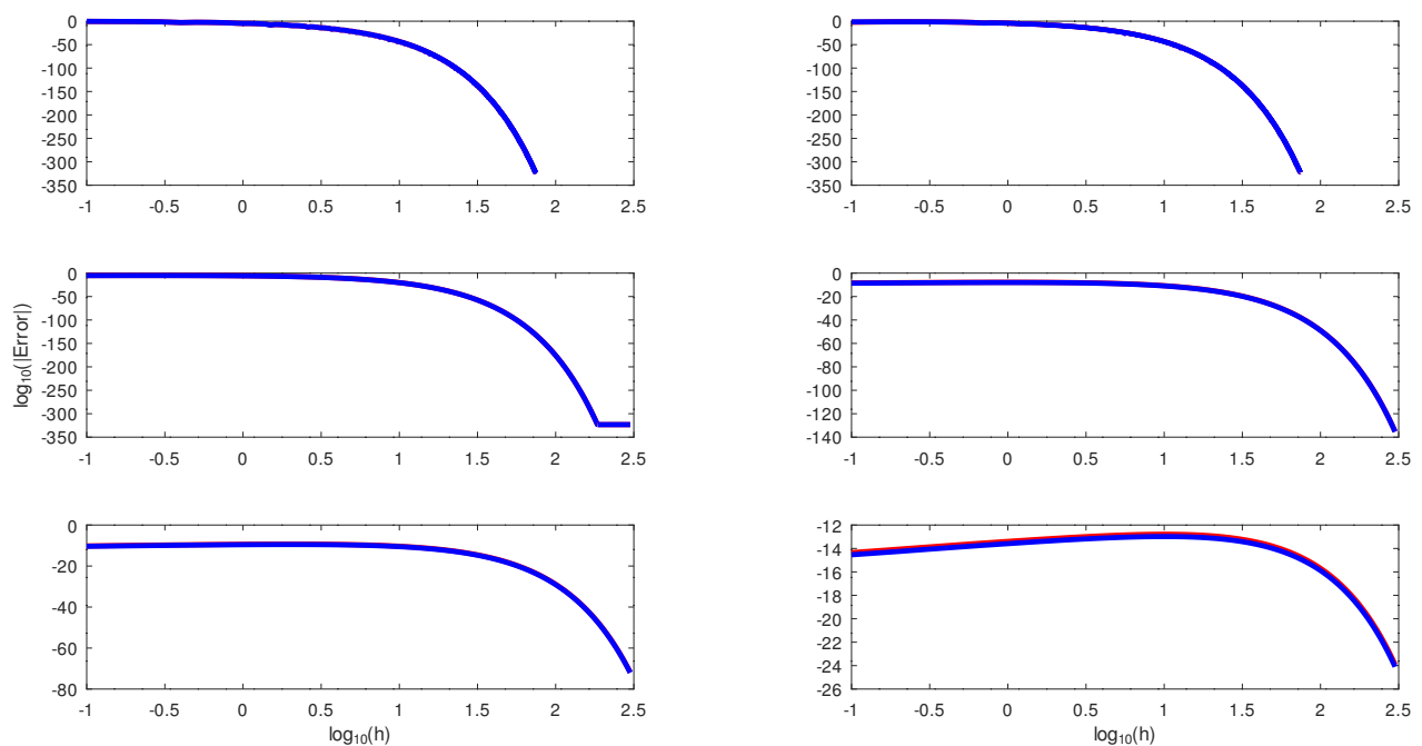
Figure 6. The log–log plots of the errors and the step size on Example 4. The red and blue lines represents y_{n+\frac{5}{2}} and y_{n+\frac{7}{4}} , respectively.
