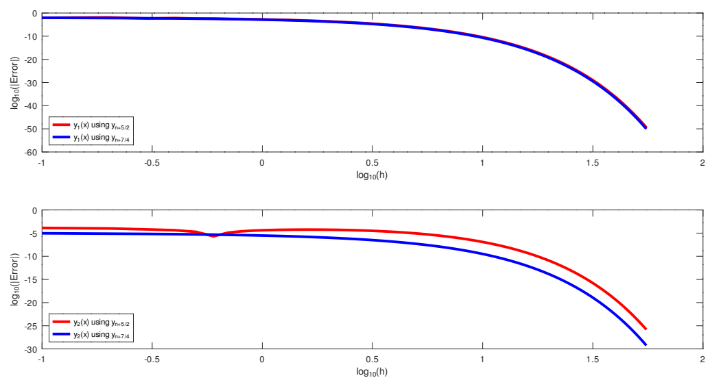
Figure 3. The log–log plots of the errors and the step size on Example 1.
