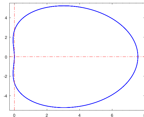
Figure 1. Region of absolute stability of the block hybrid method y_{n+\frac{7}{4}} .
