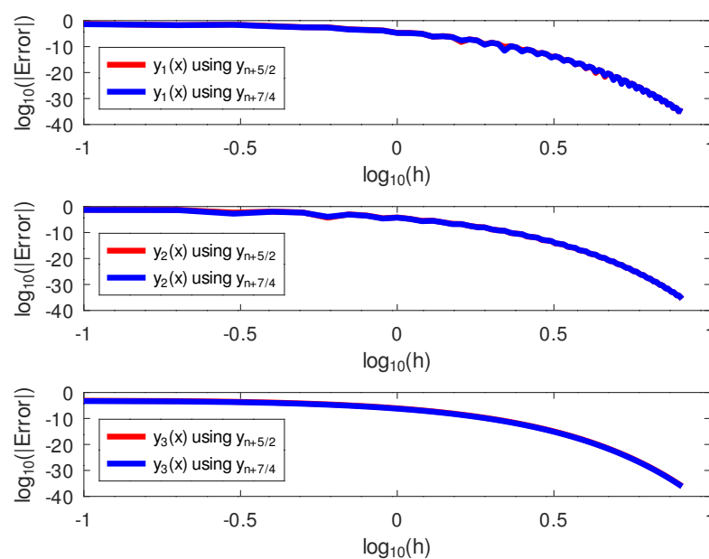
Figure 5. The log–log plots of the errors and the step size on Example 3.
