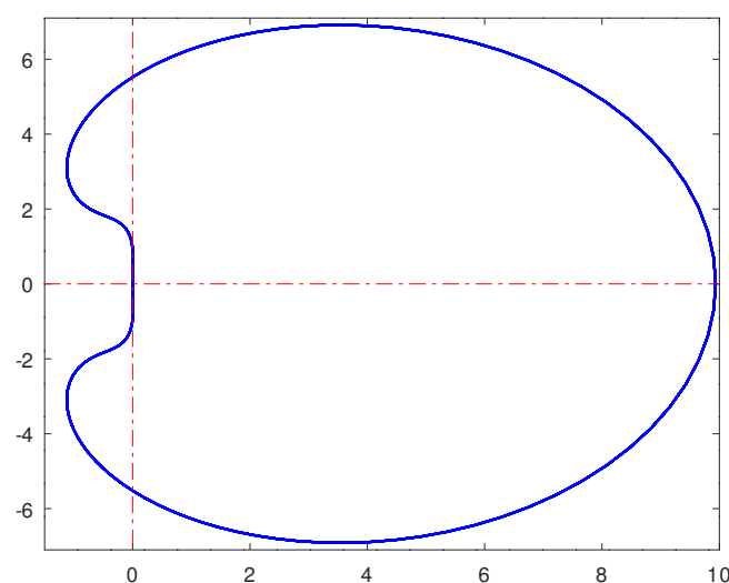
Figure 2. Region of absolute stability of the block hybrid method y_{n+\frac{5}{2}} .
