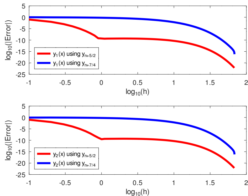
Figure 4. The log–log plots of the errors and the step size on Example 2.
