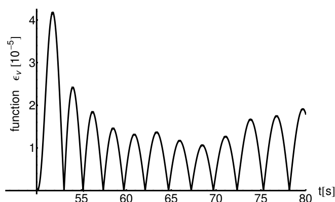
Figure 4. The residual function \varepsilon_v(t) = |v_{\text{numerical}} - \bar{v}_{\text{MOHPM}}| on interval I_3 = [50, 80] for x_{i0} = 0.25 , y_{i0} = 0.5 , z_{i0} = 1.5 , physical parameters a = 2.096 , b = 0.84 , c = 0.275 , d = 1.65 , e = 0.23 , f = 1.24 .
