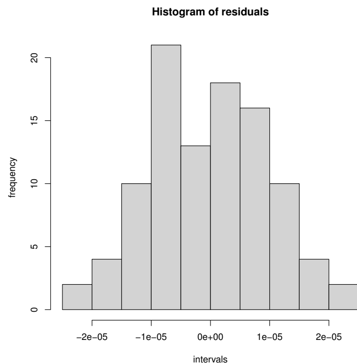
Figure 15. Histogram for the residuals.
