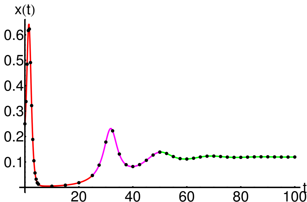
Figure 5. The MOHPM solution \bar{x}_{\text{MOHPM}} (dotted curves) versus numerical ones (color) for the original state x(t) when: x_{i0} = 0.25 , y_{i0} = 0.5 , z_{i0} = 1.5 , physical parameters: a = 2.096 , b = 0.84 , c = 0.275 , d = 1.65 , e = 0.23 , f = 1.24 . The red color curve corresponds to the subinterval I_1 ; the magenta color curve corresponds to the subinterval I_2 ; the green color curve corresponds to the subinterval I_3 .
