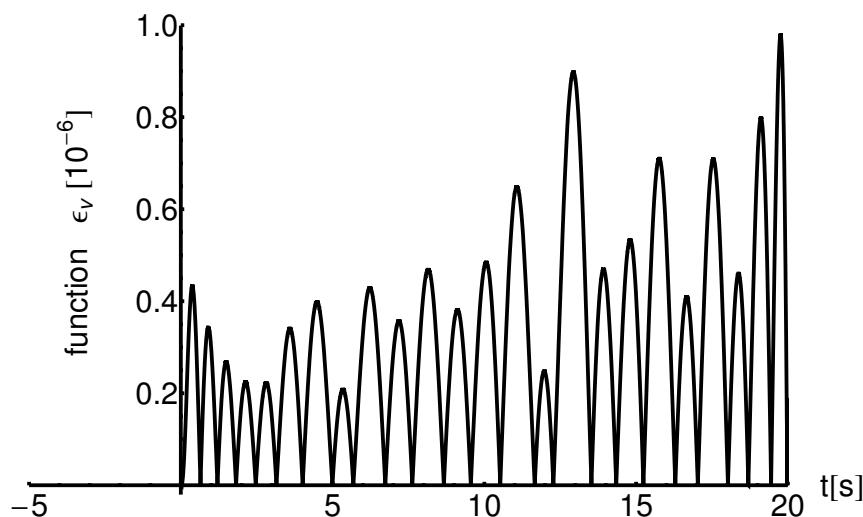
Figure 7. The residual function \varepsilon_v(t) = |v_{numerical} - \bar{v}_{MOHPM}| on interval I_1 = [0, 20] for x_{i0} = 0.125 , y_{i0} = 0.69 , z_{i0} = 0.34 , physical parameters a = 2.0 , b = 1.05 , c = \frac{bf}{3ae} \frac{-a^2+4ae-e^2}{a-e} = 0.22 , d = 2.65 , e = 0.6 , f = 2.4 .
