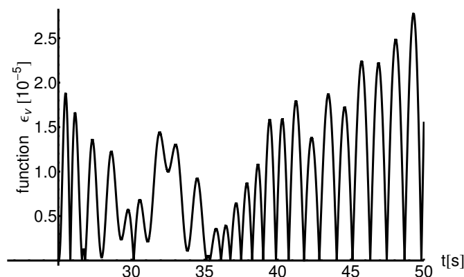
Figure 3. The residual function \varepsilon_v(t) = |v_{\text{numerical}} - \bar{v}_{\text{MOHPM}}| on interval I_2 = [25, 50] for x_{i0} = 0.25 , y_{i0} = 0.5 , z_{i0} = 1.5 , physical parameters a = 2.096 , b = 0.84 , c = 0.275 , d = 1.65 , e = 0.23 , f = 1.24 .
