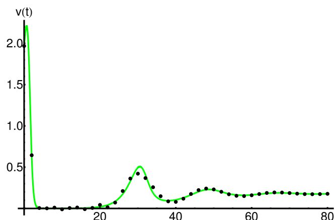
Figure 12. Comparative profiles between OHPM solution ( \bar{v}_{OHPM} ) using Equations (42) and (A7) for a small index number N_{max} = 5 ; numerical ones (color) for: x_{i0} = 0.25 , y_{i0} = 0.5 , z_{i0} = 1.5 , physical parameters: a = 2.096 , b = 0.84 , c = 0.275 , d = 1.65 , e = 0.23 , f = 1.24 .
