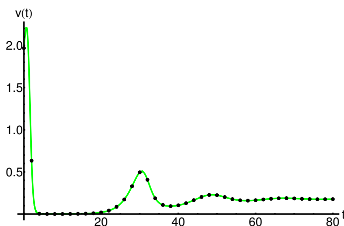
Figure 10. Comparative profiles between OHPM solution \bar{v}_{OHPM} using Equations (42) and (A7); numerical ones (color) for: x_{i0} = 0.25 , y_{i0} = 0.5 , z_{i0} = 1.5 , physical parameters: a = 2.096 , b = 0.84 , c = 0.275 , d = 1.65 , e = 0.23 , f = 1.24 .
