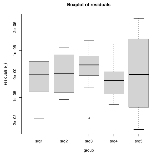
Figure 16. Box-plot for residuals. The White circle represents one singular point belongs to subgroup sgr3.
