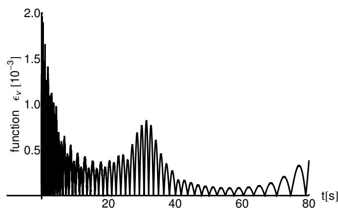
Figure 11. The residual function \varepsilon_v(t) = |v_{numerical} - \bar{v}_{OHPM}| when N_{max} = 20 , N_1 = 10 (the optimal parameters computed using extended interval [0, 80] ) for x_{i0} = 0.25 , y_{i0} = 0.5 , z_{i0} = 1.5 , physical parameters a = 2.096 , b = 0.84 , c = 0.275 , d = 1.65 , e = 0.23 , f = 1.24 .
