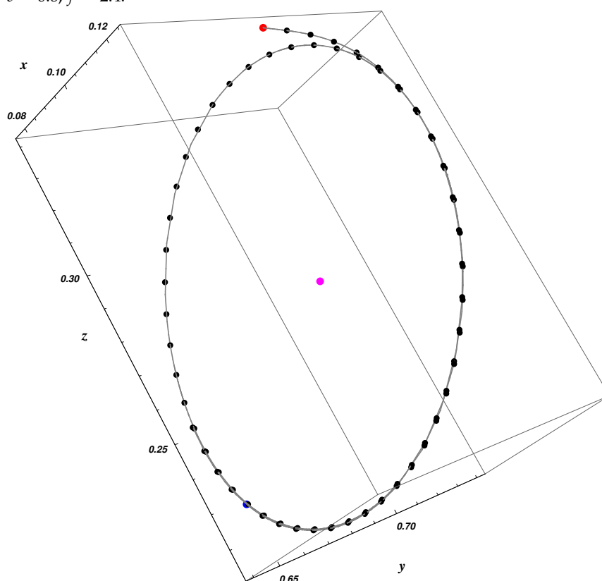
Figure 9. Almost periodical orbit (x(t), y(t), z(t)) (gray curve for numerical results) versus (\bar{x}_{\text{MOHPM}}(t), \bar{y}_{\text{MOHPM}}(t), \bar{z}_{\text{MOHPM}}(t)) (dotted black curve for MOHPM results), for initial conditions x_{i0} = 0.125 , y_{i0} = 0.69 , z_{i0} = 0.34 (red point), physical parameters a = 2.0 , b = 1.05 , c = \frac{bf}{3ae} \frac{-a^2 + 4ae - e^2}{a - e} = 0.22 , d = 2.65 , e = 0.6 , f = 2.4 ; equilibrium point \left(\frac{e}{f} \sqrt{\frac{ac}{bd}}, \sqrt{\frac{ae}{bf}}, \frac{a}{b} \sqrt{\frac{ec}{fd}}\right) (magenta point) and the point (x(19), y(19), z(19)) (blue point), respectively.
