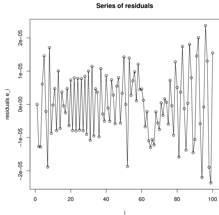
Figure 14. Series of residuals.
