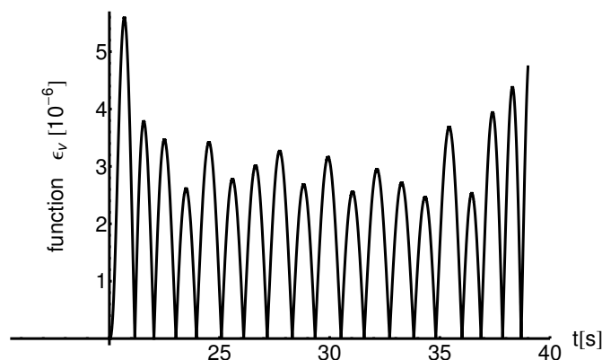
Figure 8. The residual function \varepsilon_v(t) = |v_{\text{numerical}} - \bar{v}_{\text{MOHPM}}| on interval I_2 = [20, 40] for x_{i0} = 0.125 , y_{i0} = 0.69 , z_{i0} = 0.34 , physical parameters a = 2.0 , b = 1.05 , c = \frac{bf}{3ae} \frac{-a^2 + 4ae - e^2}{a - e} = 0.22 , d = 2.65 , e = 0.6 , f = 2.4 .
