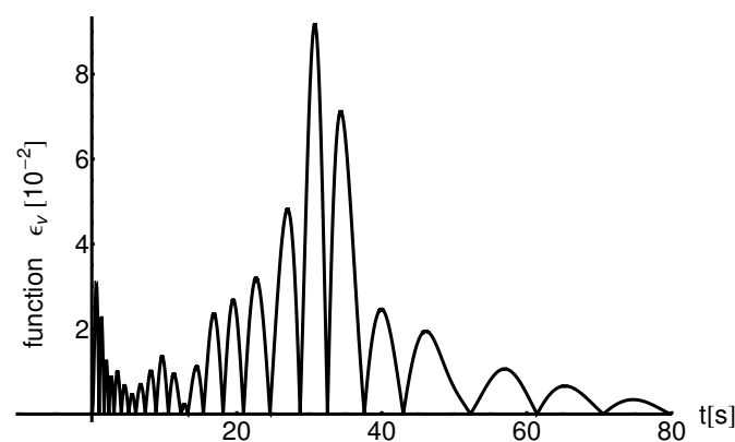
Figure 13. The residual function \varepsilon_v(t) = |v_{numerical} - \bar{v}_{OHPM}| when N_{max} = 5 , N_1 = 2 (the optimal parameters computed using extended interval [0, 80] ) for x_{i0} = 0.25 , y_{i0} = 0.5 , z_{i0} = 1.5 , physical parameters a = 2.096 , b = 0.84 , c = 0.275 , d = 1.65 , e = 0.23 , f = 1.24 .
