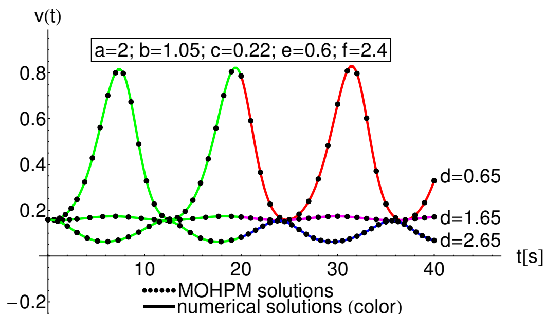
Figure 6. Effects of parameter d on MOHPM solution \bar{v}_{MOHPM} (dotted curves) versus numerical ones (color) for: x_{i0} = 0.125 , y_{i0} = 0.69 , z_{i0} = 0.34 , physical parameters: d \in \{0.65, 1.65, 2.65\} , a = 2.0 , b = 1.05 , c = \frac{bf}{3ae} \frac{-a^2 + 4ae - e^2}{a - e} = 0.22 , e = 0.6 , f = 2.4 . The green color curve corresponds to the subinterval I_1 ; the red color curve corresponds to the subinterval I_2 for d = 0.65 ; the magenta color curve corresponds to the subinterval I_2 for d = 1.65 ; the blue color curve corresponds to the subinterval I_2 for d = 2.65 .
