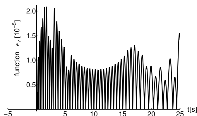
Figure 2. The residual function \varepsilon_v(t) = |v_{numerical} - \bar{v}_{MOHPM}| on interval I_1 = [0, 25] for x_{i0} = 0.25 , y_{i0} = 0.5 , z_{i0} = 1.5 , physical parameters a = 2.096 , b = 0.84 , c = 0.275 , d = 1.65 , e = 0.23 , f = 1.24 .
