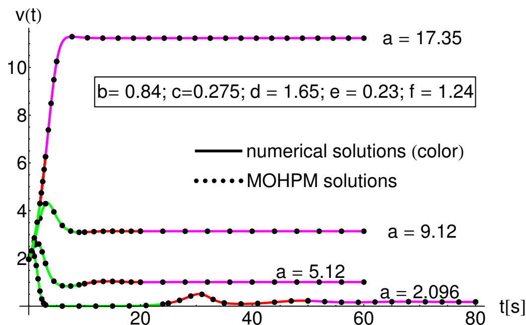
Figure 1. Effects of parameter a on MOHPM solution \bar{v}_{\text{MOHPM}} (dotted curves) versus numerical ones (color) for: x_{i0} = 0.25 , y_{i0} = 0.5 , z_{i0} = 1.5 , physical parameters: a \in \{2.096, 5.12, 9.12, 17.35\} , b = 0.84 , c = 0.275 , d = 1.65 , e = 0.23 , f = 1.24 . The green color curve corresponds to the subinterval I_1 ; the red color curve corresponds to the subinterval I_2 ; the magenta color curve corresponds to the subinterval I_3 .
