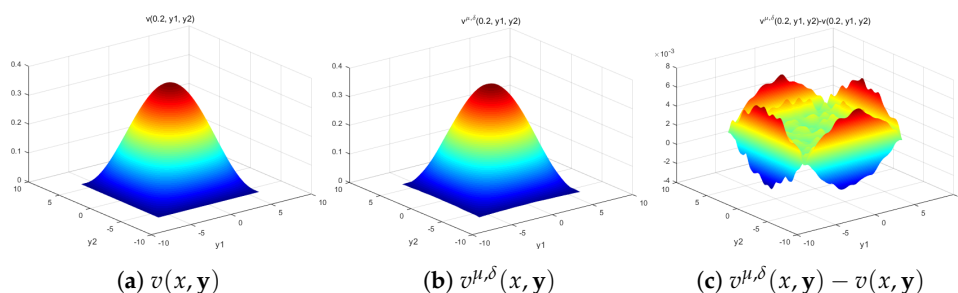
Figure 5. The exact solution v(x, y) , the regularized solution v^{\mu,\delta}(x, y) with the Poussin kernel, and the error v^{\mu,\delta}(x, y) - v(x, y) at x = 0.2 when \epsilon = 0.01 , q = \frac{1}{4} , and k = 10 .
