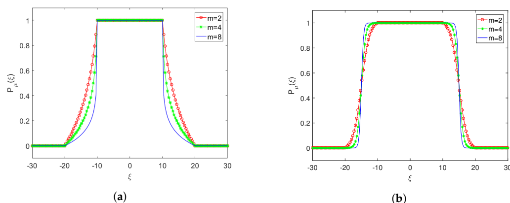
Figure 1. The logarithmic-type kernel (a) and the hyperbolic tangent-type kernel (b) for different values of m with n = 1 and \mu = 0.1 .
