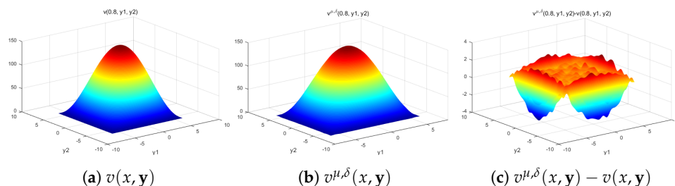
Figure 7. The exact solution v(x, y) , the regularized solution v^{\mu,\delta}(x, y) with the Poussin kernel, and the error v^{\mu,\delta}(x, y) - v(x, y) at x = 0.8 when \epsilon = 0.01 , q = \frac{1}{4} , and k = 10 .
