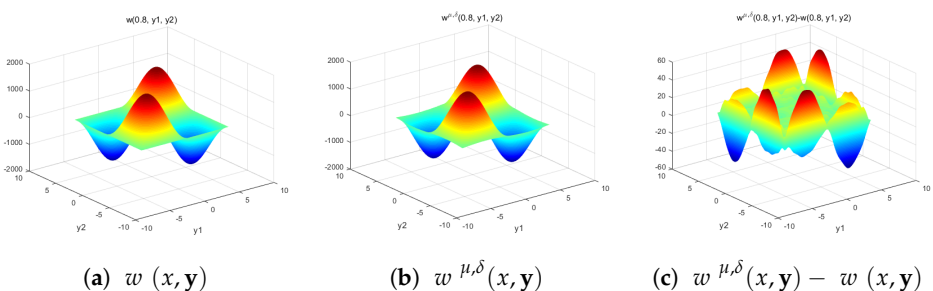
Figure 10. The exact solution w(x, y) , the regularized solution w^{\mu,\delta}(x, y) with the Poussin kernel, and the error w^{\mu,\delta}(x, y) - w(x, y) at x = 0.8 when \epsilon = 0.01 and k = 10 .
