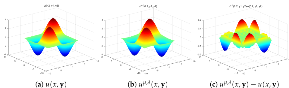
Figure 2. The exact solution u(x, y) , the regularized solution u^{\mu, \delta}(x, y) with the Poussin kernel, and the error u^{\mu, \delta}(x, y) - u(x, y) at x = 0.2 when \epsilon = 0.01 , q = \frac{1}{2} , and k = 10 .
