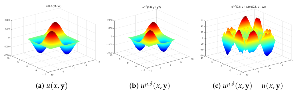
Figure 4. The exact solution u(x, y) , the regularized solution u^{\mu, \delta}(x, y) with the Poussin kernel, and the error u^{\mu, \delta}(x, y) - u(x, y) at x = 0.8 when \epsilon = 0.01 , q = \frac{1}{2} , and k = 10 .
