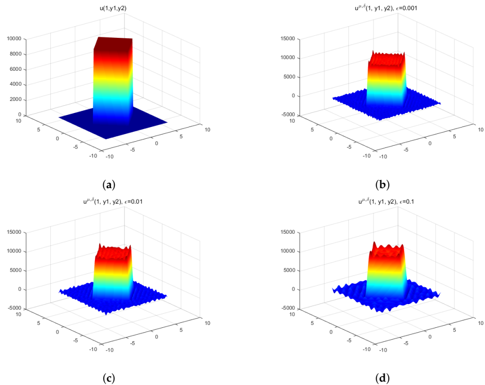
Figure 13. The exact solution u(1, \mathbf{y}) (a) and the regularized solutions u^{\mu,\delta}(1, \mathbf{y}) with the Poussin kernel when k = 10 , for noise levels \epsilon = 0.001 (b), 0.01 (c), and 0.1 (d).
