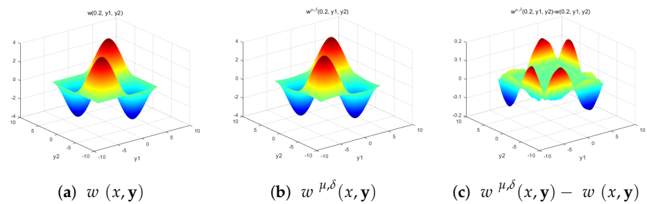
Figure 8. The exact solution w(x, y) , the regularized solution w^{\mu,\delta}(x, y) with the Poussin kernel, and the error w^{\mu,\delta}(x, y) - w(x, y) at x = 0.2 when \epsilon = 0.01 and k = 10 .
