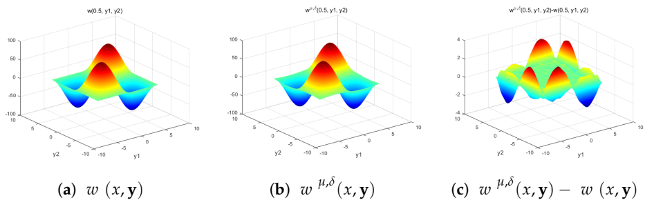
Figure 9. The exact solution w(x, y) , the regularized solution w^{\mu,\delta}(x, y) with the Poussin kernel, and the error w^{\mu,\delta}(x, y) - w(x, y) at x = 0.5 when \epsilon = 0.01 and k = 10 .
