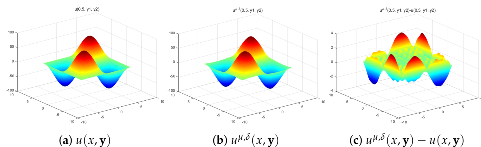
Figure 3. The exact solution u(x, y) , the regularized solution u^{\mu, \delta}(x, y) with the Poussin kernel, and the error u^{\mu, \delta}(x, y) - u(x, y) at x = 0.5 when \epsilon = 0.01 , q = \frac{1}{2} , and k = 10 .
