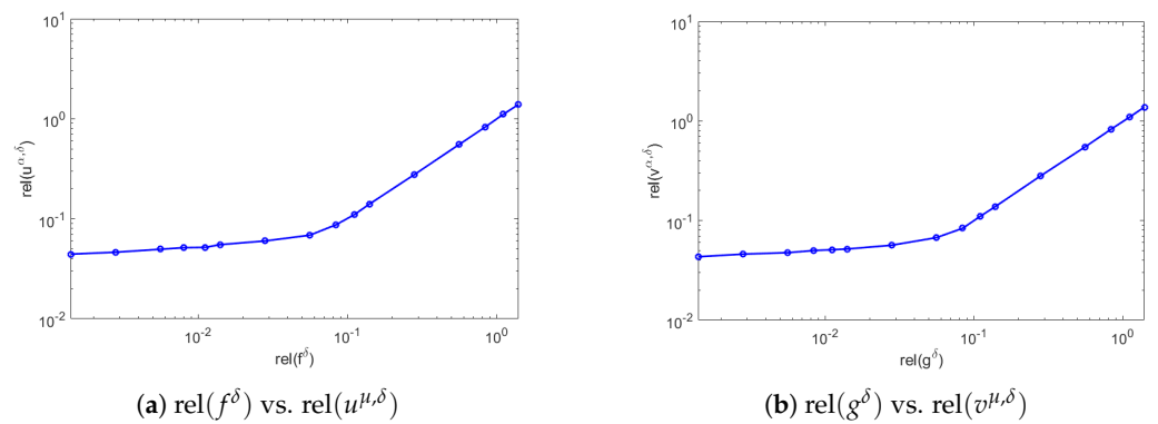
Figure 12. Log-log plots of relative errors for k = 10 and x = 1 : (a) \text{rel}(f^\delta) vs. \text{rel}(u^{\mu,\delta}) and (b) \text{rel}(g^\delta) vs. \text{rel}(v^{\mu,\delta}) .
