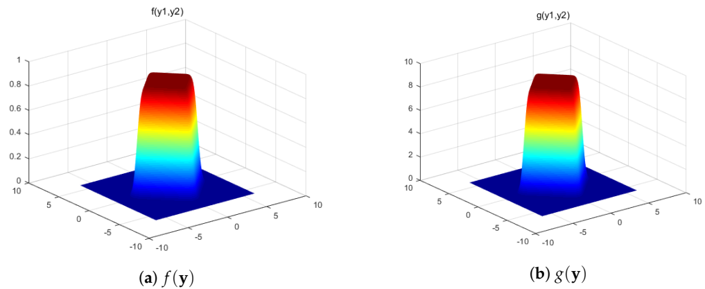
Figure 11. The exact data f(\mathbf{y}) and g(\mathbf{y}) in Example 4 for k = 10 .
