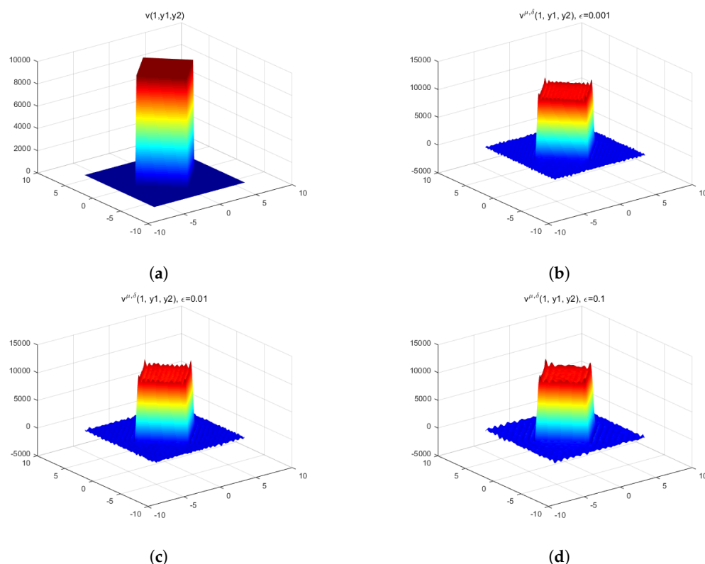
Figure 14. The exact solution v(1, \mathbf{y}) (a) and the regularized solutions v^{\mu, \delta}(1, \mathbf{y}) with the Poussin kernel when k = 10 , for noise levels \epsilon = 0.001 (b), 0.01 (c), and 0.1 (d).
