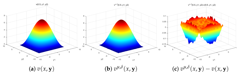
Figure 6. The exact solution v(x, y) , the regularized solution v^{\mu,\delta}(x, y) with the Poussin kernel, and the error v^{\mu,\delta}(x, y) - v(x, y) at x = 0.5 when \epsilon = 0.01 , q = \frac{1}{4} , and k = 10 .
