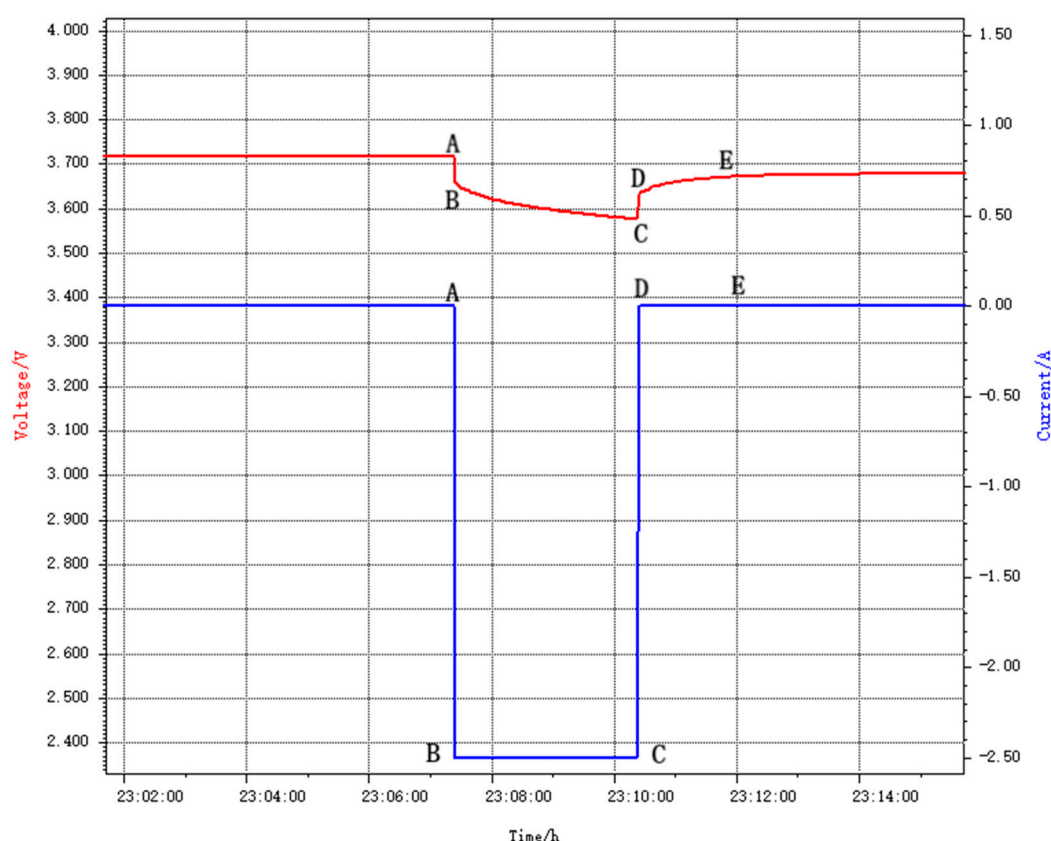
Figure 2. Magnified View of a Single Cycle from the HPPC Test Profile.
