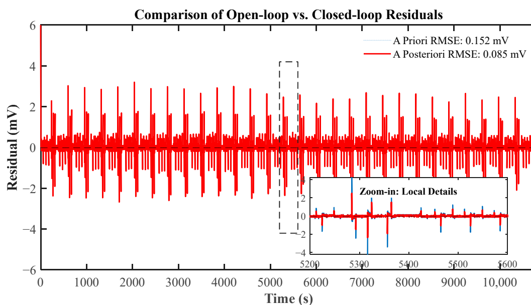
Figure 11. Decoupled analysis of terminal voltage residuals.
