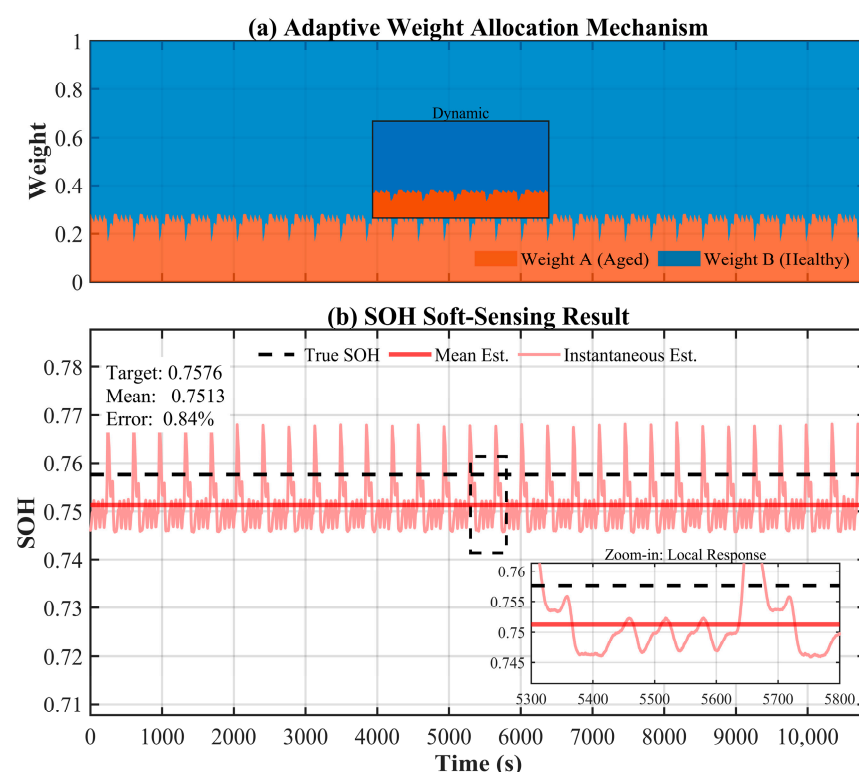
Figure 13. Mechanism and validation of real-time SOH Soft-Sensing: (a) Dynamic evolution of adaptive fusion weights reflecting impedance matching; (b) Comparison of estimated SOH trajectory against ground truth.
