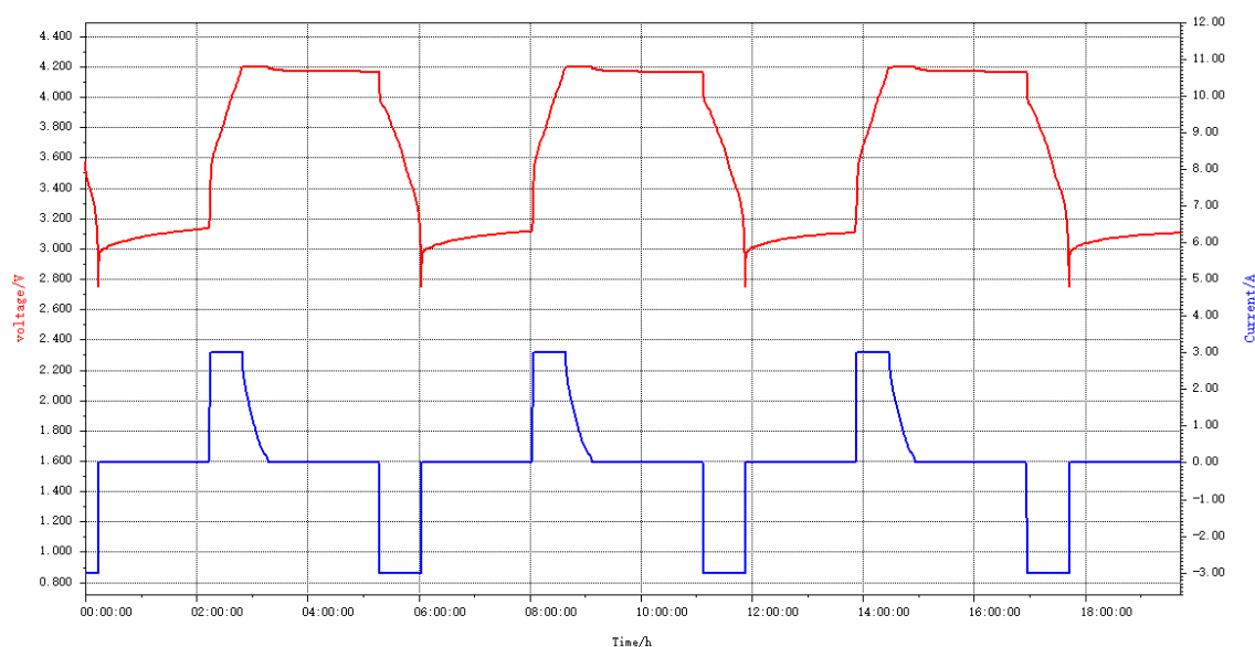
Figure 9. Time-domain voltage and current profiles during the capacity calibration process.
