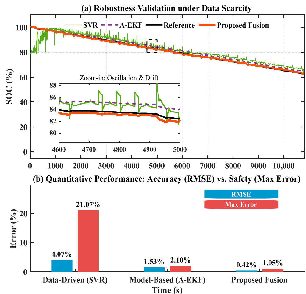
Figure 12. Performance benchmarking against state-of-the-art SOC estimation methods under data-scarce conditions.
