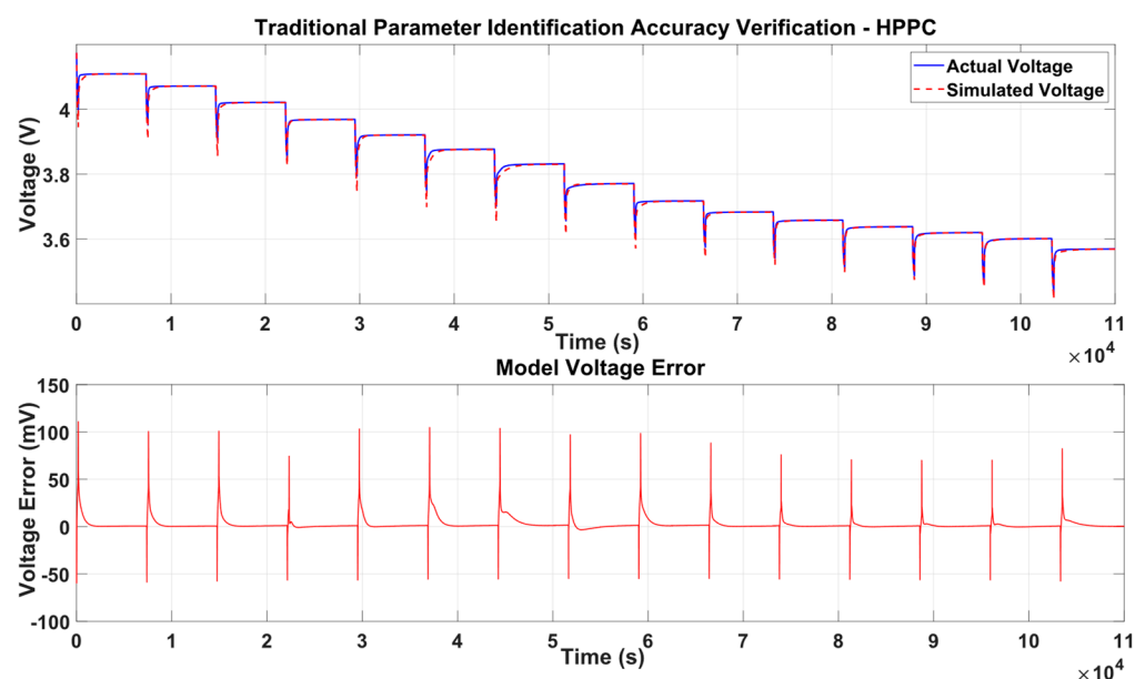
Figure 5. Verification Results for the Model with Parameters Identified by the Traditional Method.
