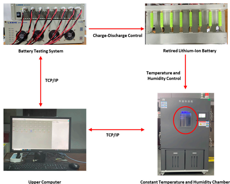
Figure 8. The experimental setup for battery testing. The red circle indicates the chamber work-space where the battery fixture is placed for temperature and humidity control.
