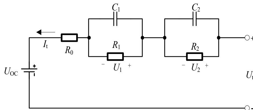
Figure 1. Schematic of the second-order RC equivalent circuit model.
