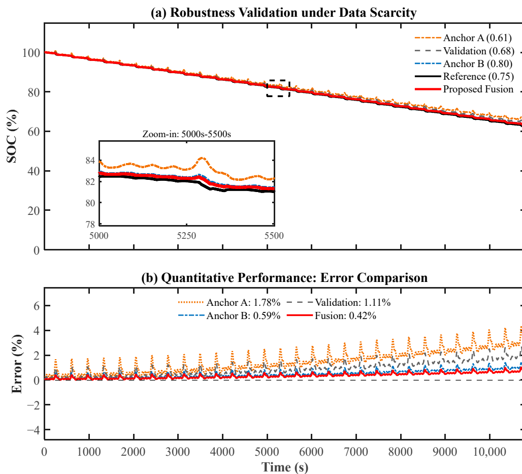
Figure 10. Comparison of SOC estimation results between the proposed Dual-Anchor Fusion framework and static fixed-parameter models (Anchors and Validation) under DST cycles.
