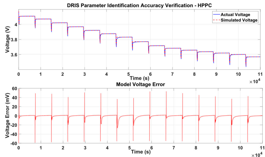
Figure 6. Verification Results for the Model with Parameters Identified by the DRIS Strategy.
