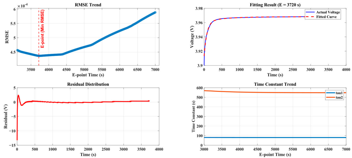
Figure 4. Analysis of the DRIS Strategy for Parameter Identification at a Typical SOC Interval.
