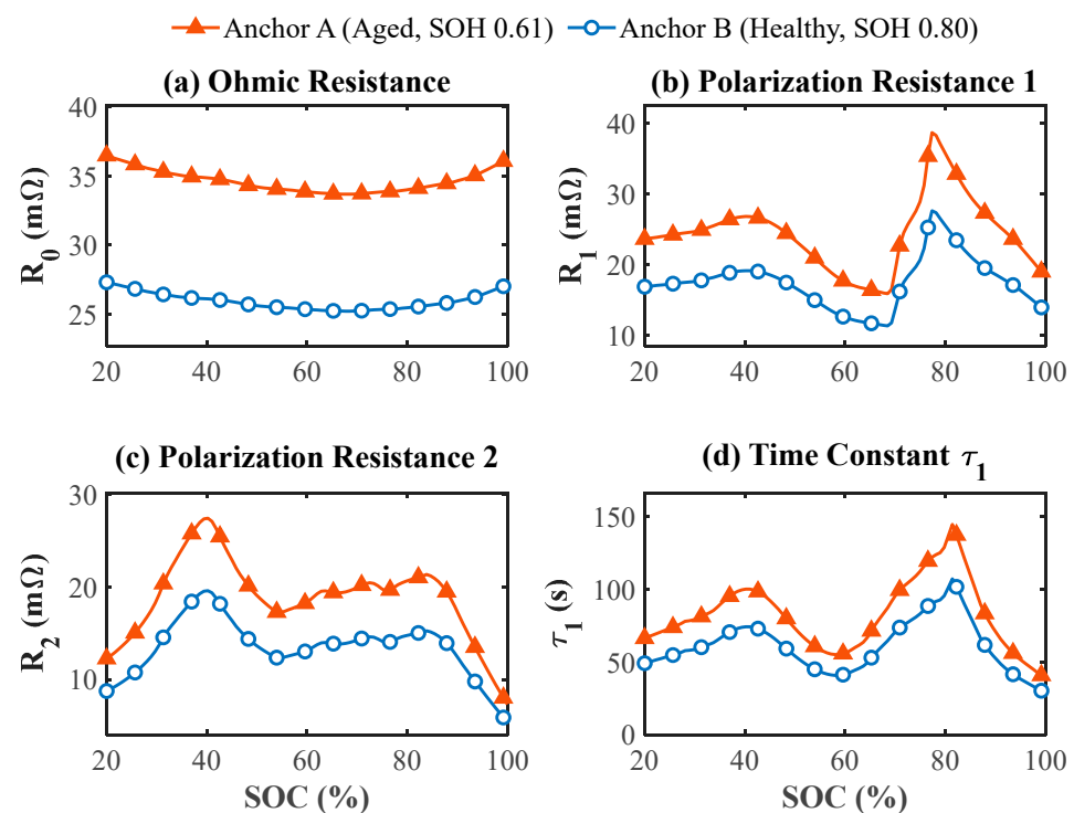
Figure 7. Comparison of identified model parameters ( R_0 , R_1 , R_2 , \tau_1 ) for the two anchor boundaries (SOH 0.61 vs. SOH 0.80) across the operating SOC range.
