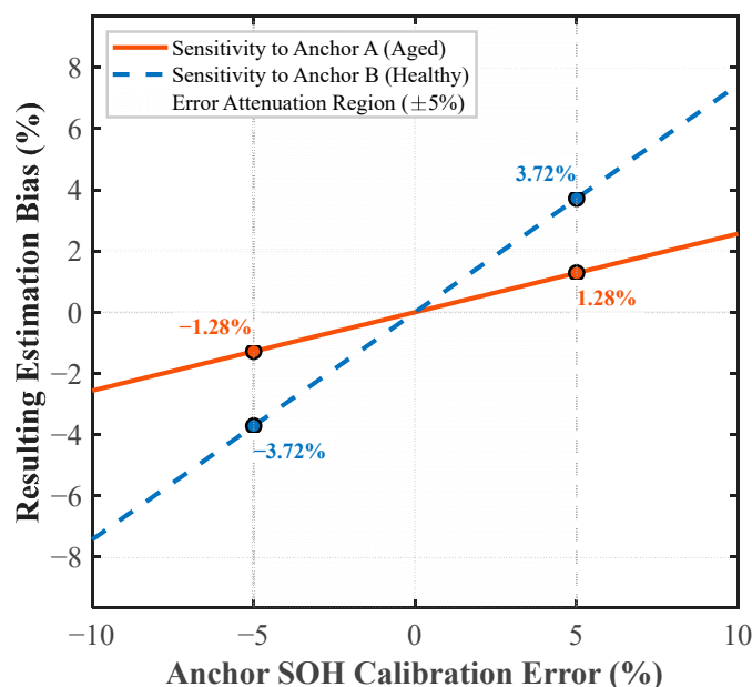
Figure 14. Sensitivity analysis of SOH estimation bias versus anchor calibration errors.
