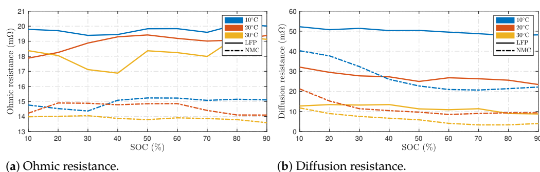
Figure 7. Estimated resistances recorded from [35].
