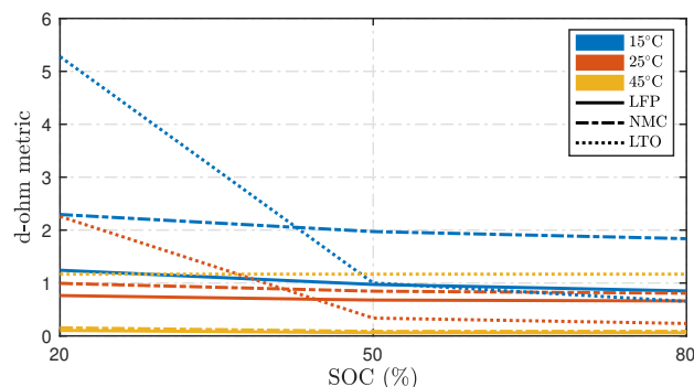
Figure 10. Proposed d-ohm metric computed using (12) using estimated resistances recorded from [13].
