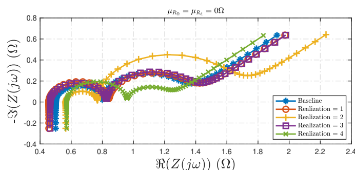
Figure 5. Variations in the impedance spectrum due to different variance values for ohmic and diffusion resistances, \sigma_{R_\Omega} = 0.1 \Omega and \sigma_{R_d} = 0.26 \Omega . It is assumed that \mu_{R_\Omega} = \mu_{R_d} = 0 \Omega .
