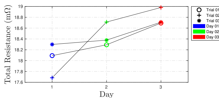
(b) Total Resistance defined in (20).
