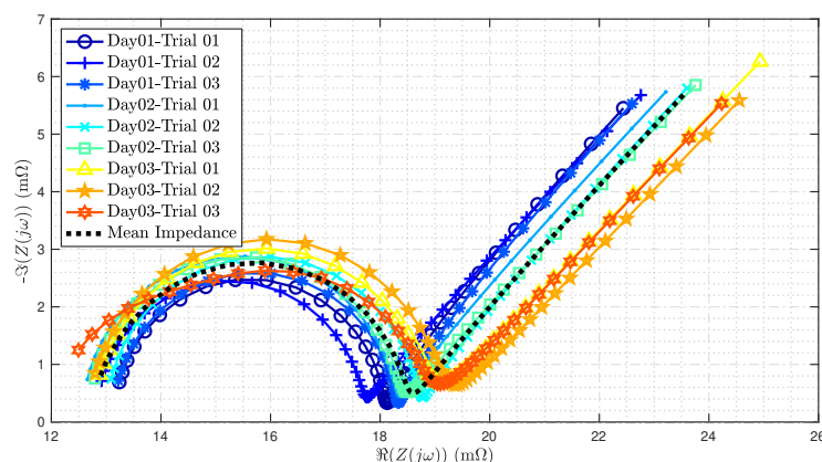
Figure 18. Impedance spectrum from estimated parameters for three repeated trials on three different days for the battery. See the corresponding measured data in Figure 17.
