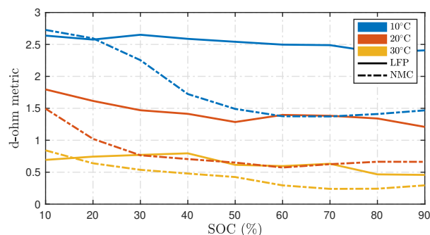
Figure 8. Proposed metric ‘d-ohm’ computed using (12) using estimated resistances recorded from [35].
