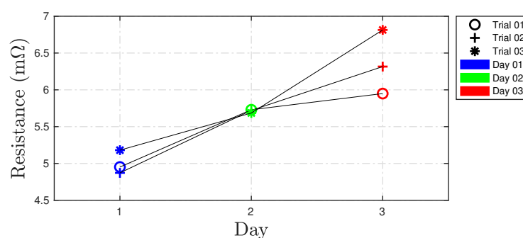
(a) Diffusion Resistance defined in (5).
