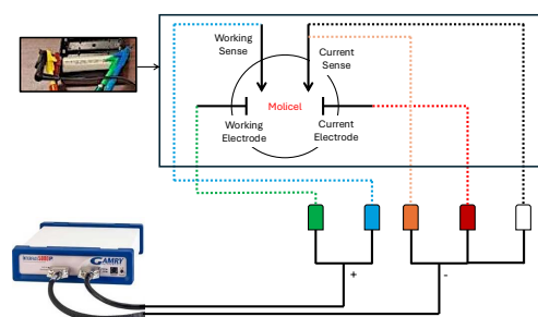
(a) Connection diagram.
