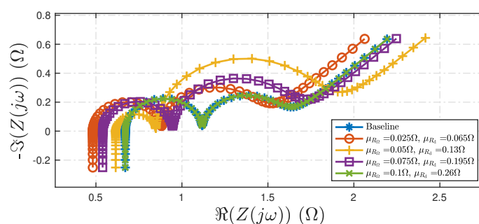
Figure 6. Variations in the impedance spectrum due to different bias and variance values for the assumed Gaussian distributions of resistances in (8) and (9). Assumed variances are \sigma_{R_\Omega} = 0.1 \Omega and \sigma_{R_d} = 0.26 \Omega .
