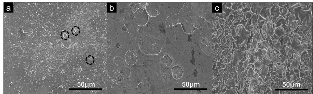
Figure 6. SEM analysis of U-2 OS cells seeded on square glass cover slips coated with (a) PEI coating, (b) PDPA coating and (c) CHI coating, examined at a magnification of \times 1k and cultured under standard conditions for 7 days.
