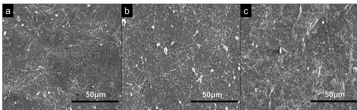
Figure 2. SEM analysis of 60 QL (a) PEI, (b) PDDA and (c) CHI coatings on glass microscopic slides examined at a magnification of \times 1k .
