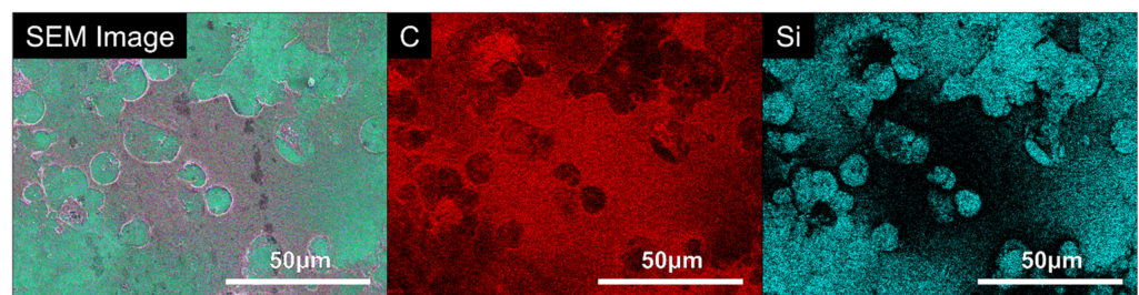
Figure 7. EDX analysis of the U-2 OS film formed on the square glass cover slips coated with the PDPA coating.
