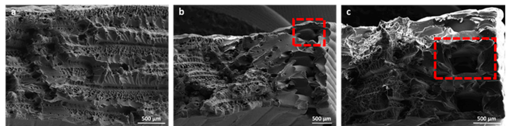
Figure 12. Explanatory SEM images of the fractured surfaces: (a,b) from specimen tested at 0.5 mm/min and (c) from specimen tested at 10 mm/min. Red boxes indicate the possible crack initiation site. Original images, from Figures S1–S3, are available in the Supplementary Materials.
