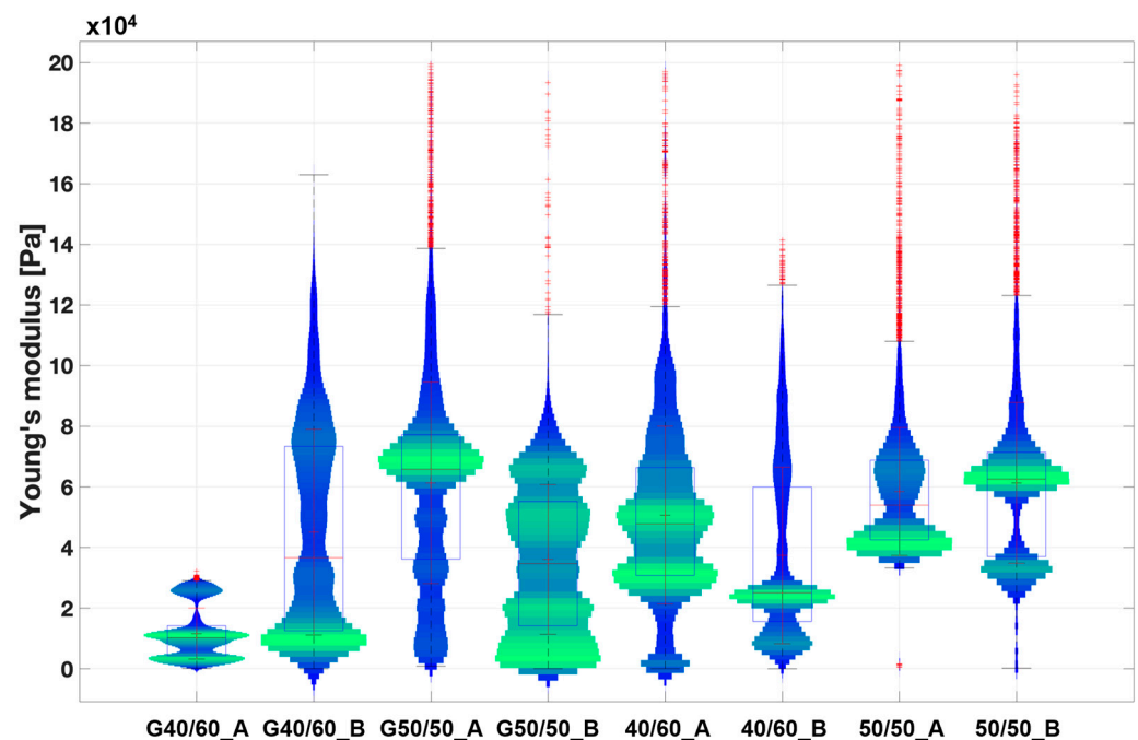
Figure 7. Violin plot of the extracted Young's modulus from the collected extended curves of PCL fibrous scaffold samples in wet conditions. Scaffolds coated with Gelatin are coded with G. The graph illustrates the distribution of the measured Young's modulus values across various scaffold surface areas. A broader and more pronounced green range indicates a higher frequency of measured values within that range, while blue range represents less frequently detected values. Finally, each red cross stands for an outlier value.
