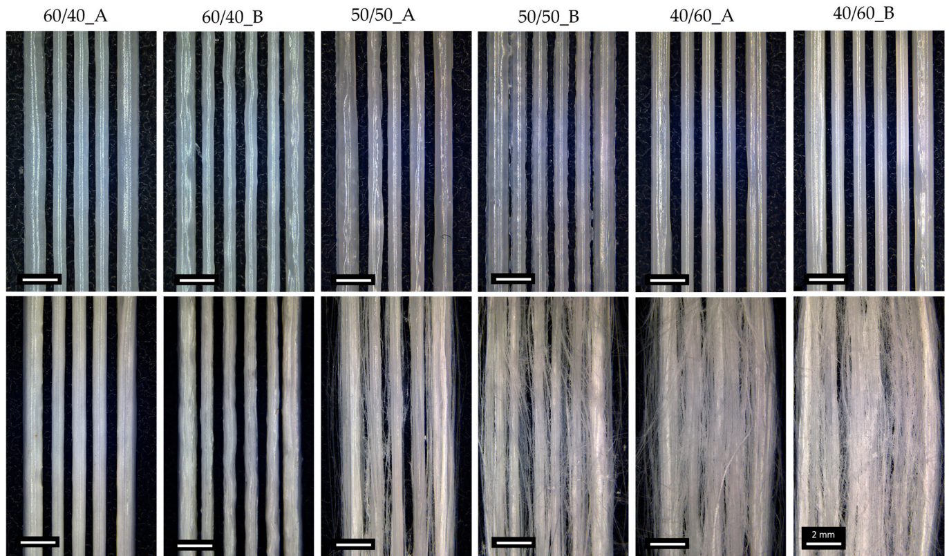
Figure 2. Optical images of 3D-printed PCL/PEG scaffolds before (up) and after (down) the leaching process, showing the effect of the blend composition and FD on fiber formation.
