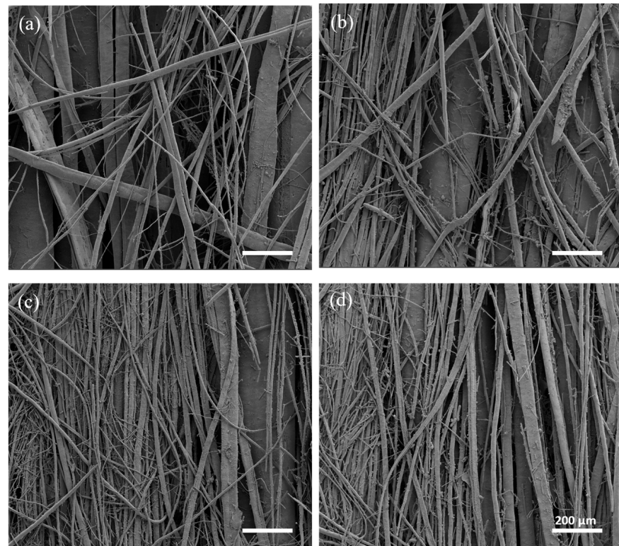
Figure 4. SEM images taken at a high magnification (100×): (a) 50/50_A, (b) 50/50_B, (c) 40/60_A, and (d) 40/60_B.
