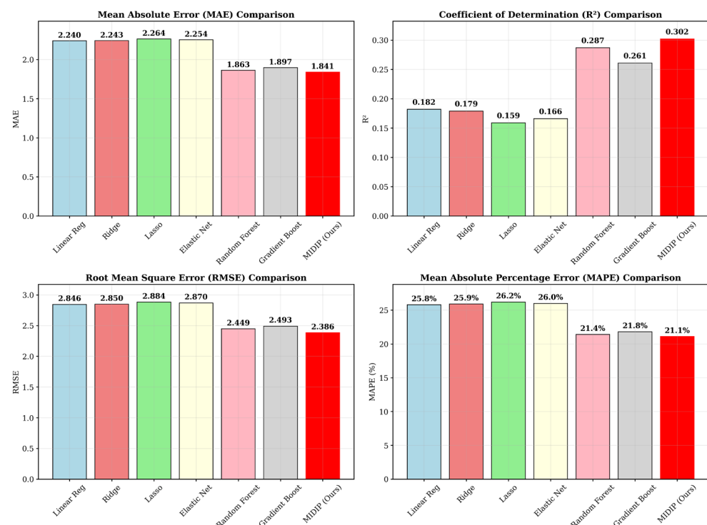
Figure 3. Comparison of the proposed model with MIDIP using representative regression evaluation indices.
