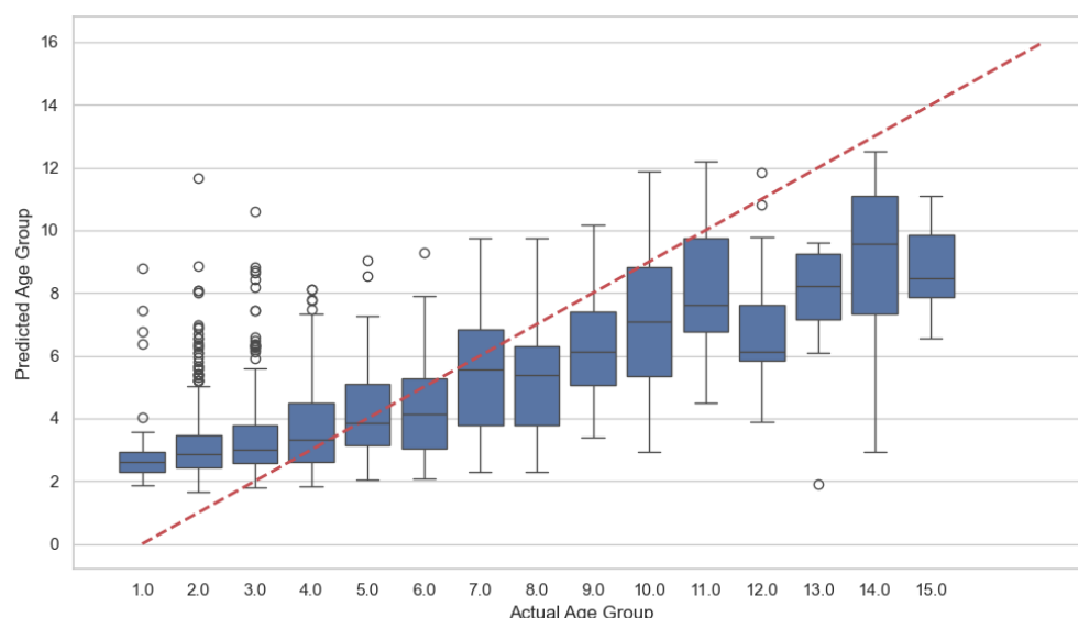
Figure 4. Age group prediction: Actual values vs. predicted values (random forest).
