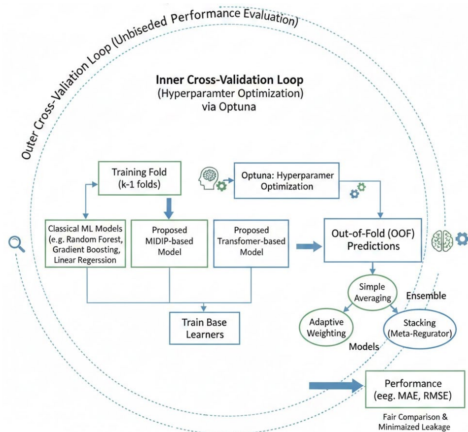
Figure 2. Schematic overview of the nested cross-validation and ensemble learning framework.
