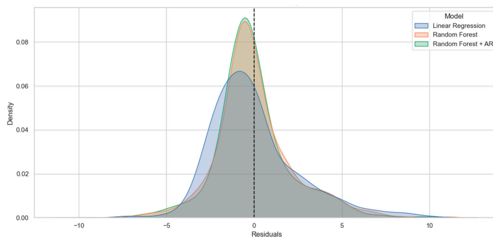
Figure 5. Comparison of residual distributions. Blue: linear regression, red: random forest, green: random forest and AR (vertical axis represents density).
