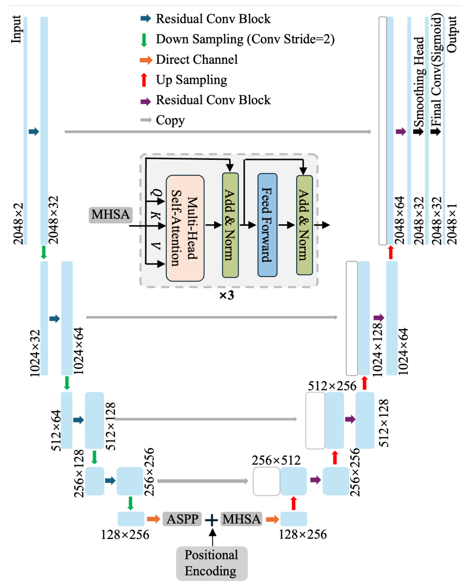
Figure 3. Proposed 1D U-Net–MHSA architecture with residual encoder–decoder, skip connections, ASPP+MHSA bottleneck, and a smoothing head with sigmoid output.
