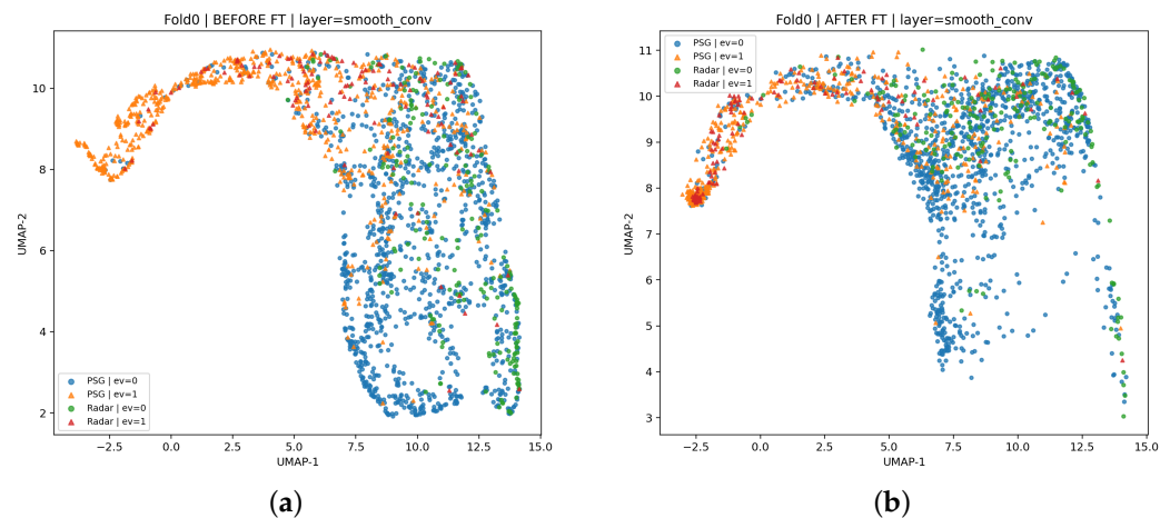
Figure 5. UMAP visualization of PSG and radar features at layer smooth_conv. (a) Before fine-tuning. (b) After fine-tuning. The UMAP embedding was fitted on pre-fine-tuning features, and post-fine-tuning features were projected using the same scaler and UMAP reducer for direct comparison.
