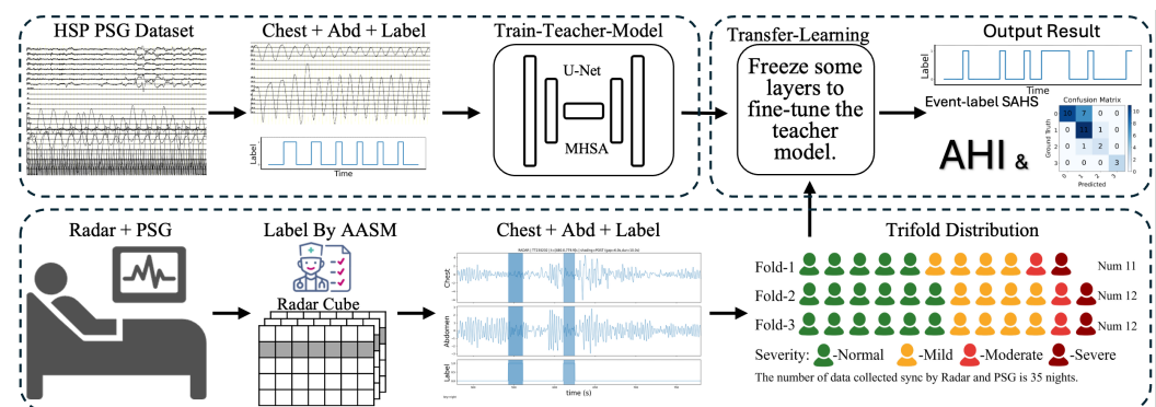
Figure 1. PSG-to-radar transfer-learning pipeline: train a teacher on HSP PSG and fine-tune on synchronized radar data to predict SAHS events and AHI (3-fold, 35 nights).
