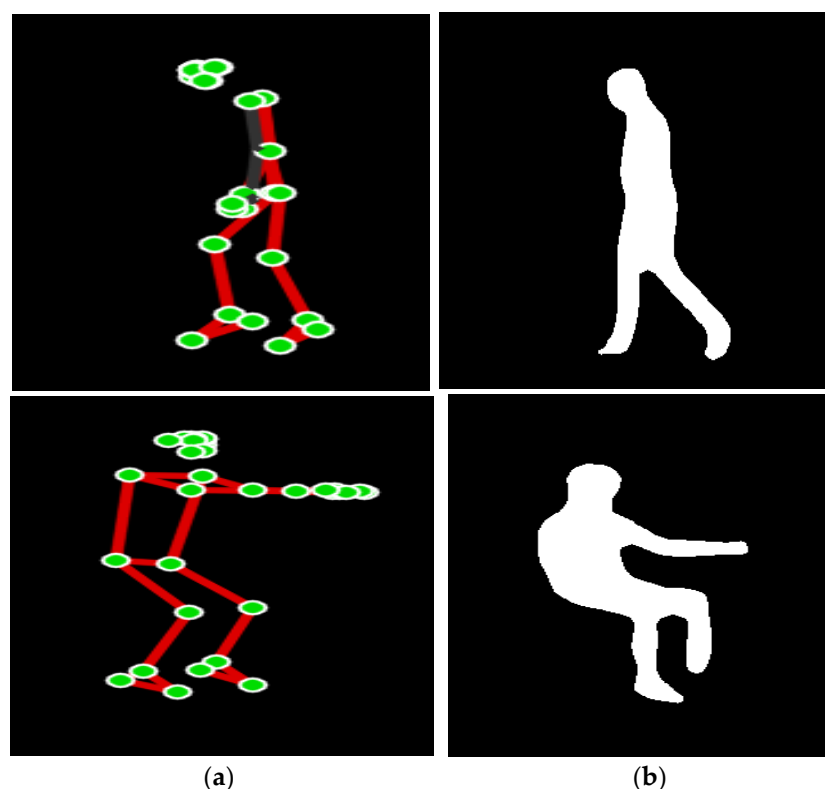
Figure 4. Results of skeleton modeling and silhouette extraction with (a) skeleton model, (b) silhouette extraction over VIDIMU dataset.
