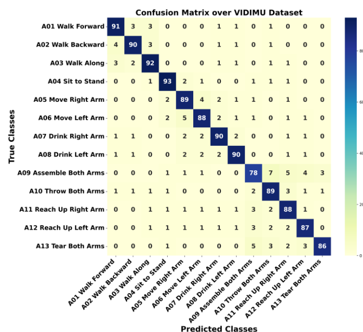
Figure 15. Confusion matrix for various classes for VIDIMU dataset.
