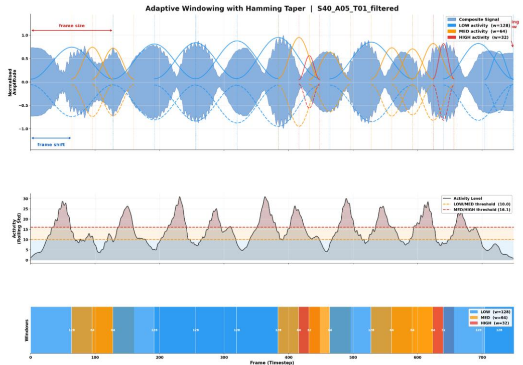
Figure 3. Adaptive windowing with Hamming taper showing composite inertial signal, activity intensity levels with thresholds, and resulting variable-length windows categorized into low, medium, and high activity over VIDIMU dataset.
