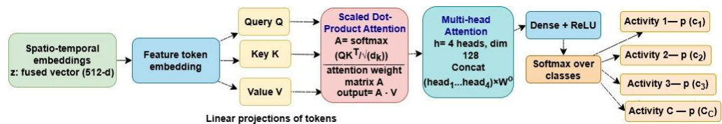
Figure 14. Architecture of attention-based classification network.
