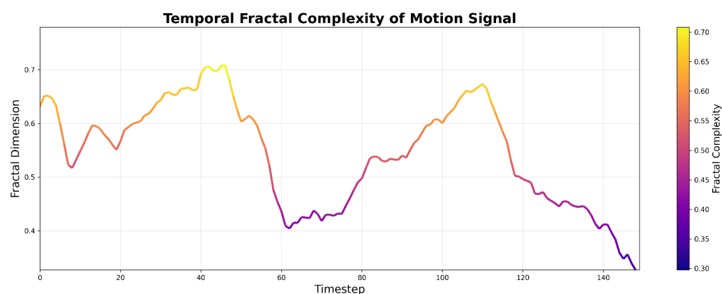
Figure 7. Temporal variation in Fractal Dimension representing motion complexity over time. Higher values indicate irregular, chaotic movements, while lower values reflect smoother and stable activity patterns over VIDIMU dataset.
