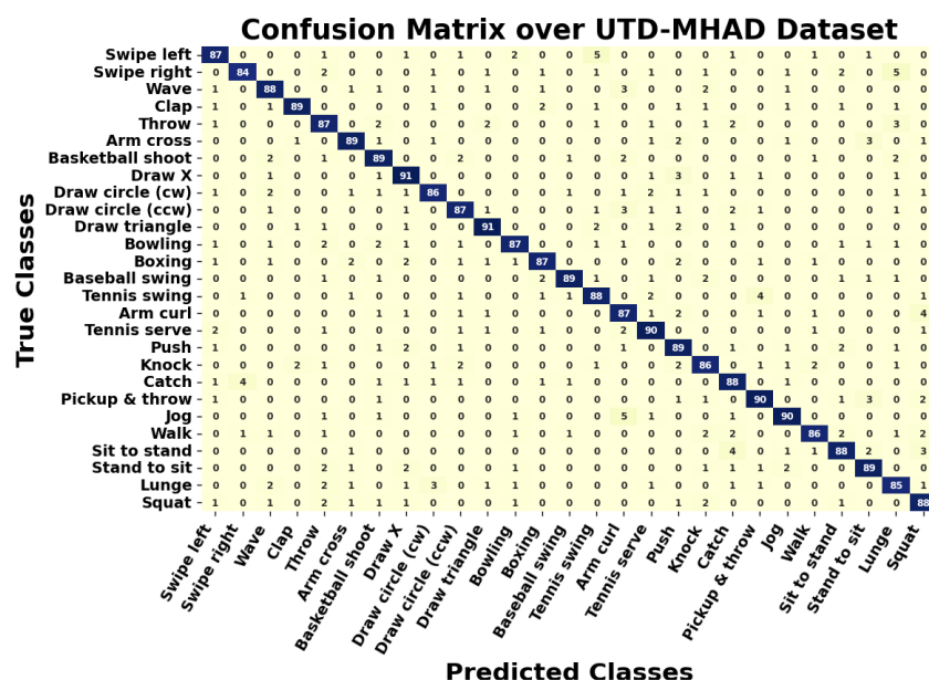
Figure 16. Confusion matrix for various classes for UTD-MHAD dataset.
