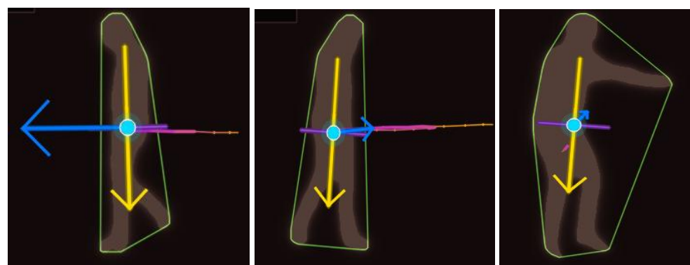
Figure 9. Body orientation (yellow axis) is estimated via PCA and centroid-based trajectory (blue vector) across frames. Motion direction and posture changes are captured jointly, highlighting spatial alignment and temporal displacement patterns.
