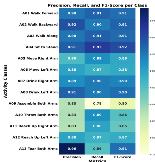
Figure 17. Evaluation matrices (precision, recall and F1 score) for various classes for VIDIMU dataset.
