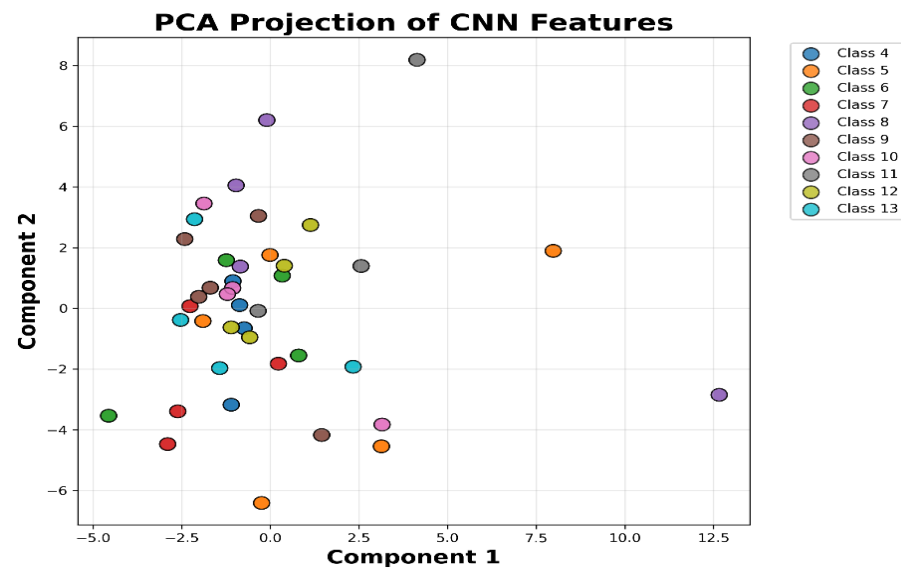
Figure 5. PCA projection of 1D-CNN-extracted deep features onto two principal components, illustrating the distributional spread of 10 activity classes (Classes 4–13) from the VIDIMU dataset.
