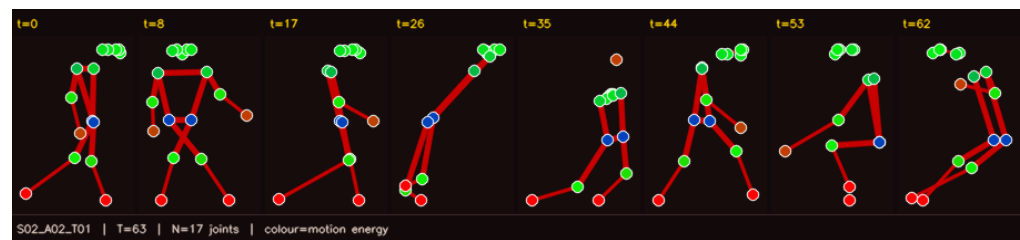
Figure 11. Temporal sequence of skeleton graphs illustrating joint connectivity and motion evolution across frames. Node colors represent motion energy, highlighting dynamic joints and activity intensity over time.
