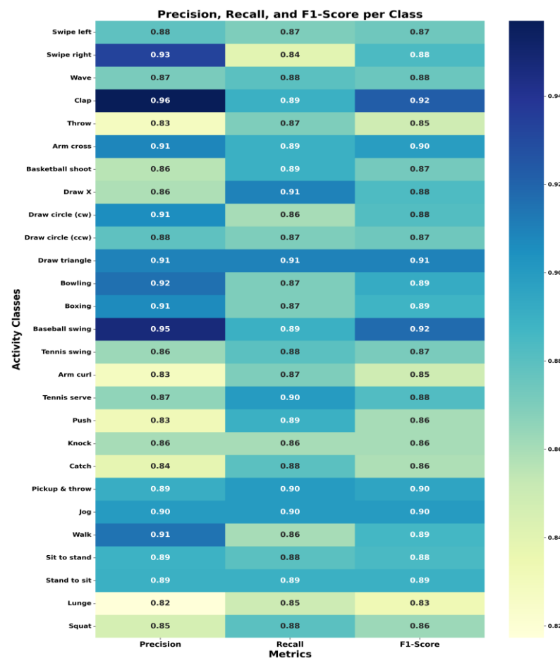
Figure 18. Evaluation matrices (precision, recall and F1 score) for various classes for UTD-MHAD dataset.
