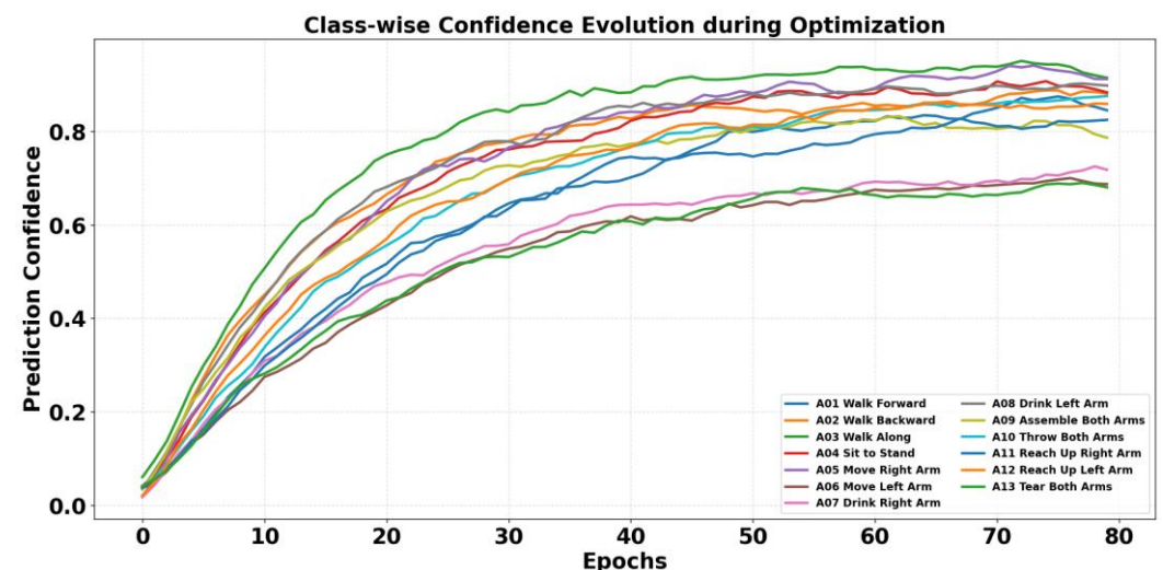
Figure 13. Ranger optimization results for VIDIMU dataset.
