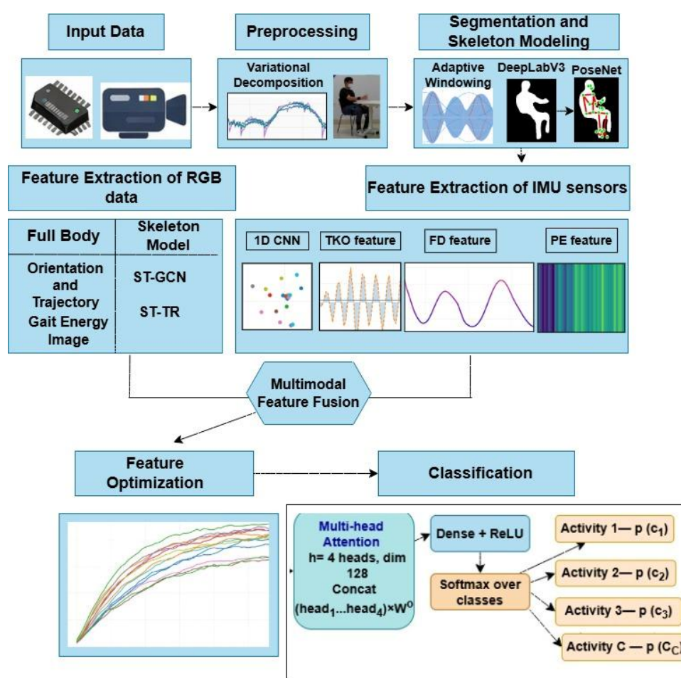
Figure 1. The system architecture of the proposed model.
