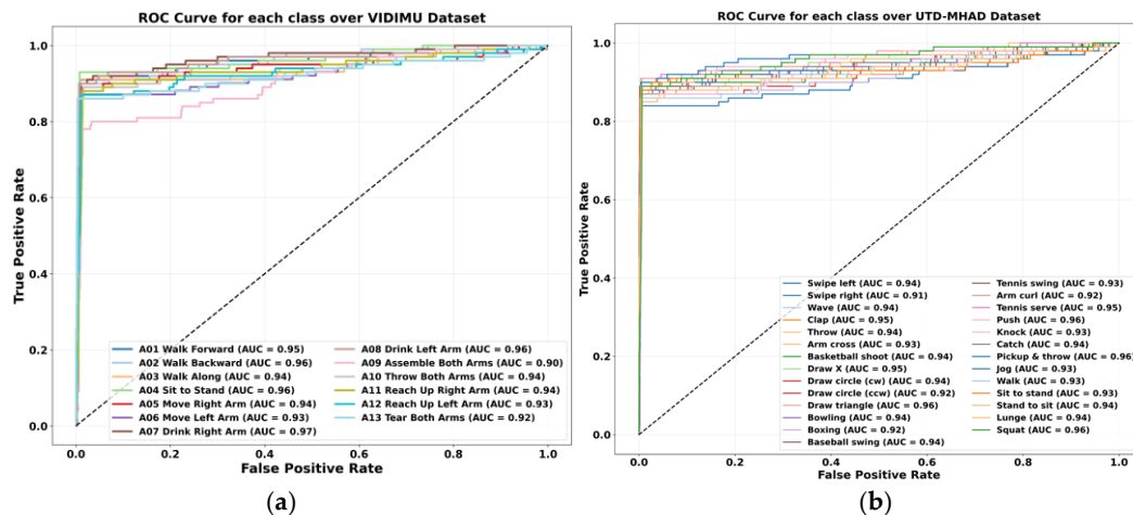
Figure 19. ROC curves for (a) VIDIMU and (b) UTD-MHAD datasets.
