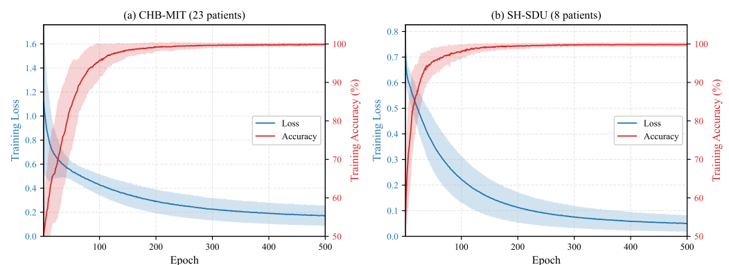
Figure 3. Average cross-entropy training loss and training accuracy curves. (a) CHB-MIT dataset (23 patients). (b) SH-SDU dataset (8 patients). The shaded area around the curves represents the \pm 1 standard deviation region.
