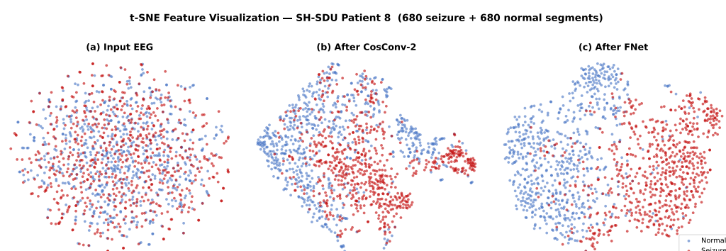
Figure 5. t-SNE feature visualization for SH-SDU Patient 8. (a) Raw input EEG; (b) after CosConv Layer-2; (c) after FNet encoder. Red indicates seizure segments and blue indicates normal segments.
