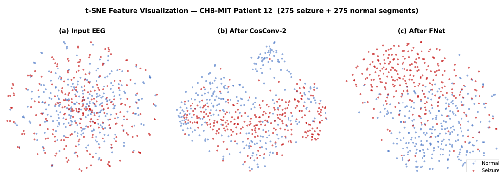
Figure 4. t-SNE feature visualization for CHB-MIT Patient 12. (a) Raw input EEG; (b) after CosConv Layer-2; (c) after FNet encoder. Red indicates seizure segments and blue indicates normal segments.
