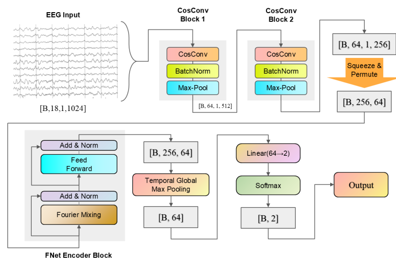
Figure 1. Overall architecture of CosFNet. The arrows indicate the direction of data flow; the orange arrow denotes the squeeze-and-permute operation that transforms the feature tensor from [B, 64, 1, 256] to [B, 256, 64] . The model comprises two CosConv blocks for local feature extraction, an FNet encoder for global token-feature mixing, and a max-pooling classification head.
