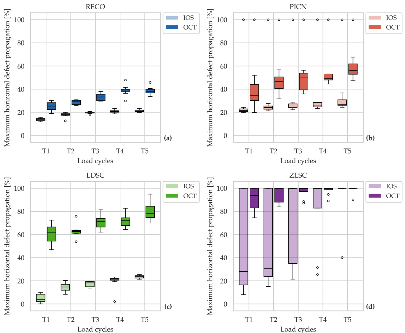
Figure 4. Maximum horizontal defect propagation (%) by intraoral scanning (IOS, surface wear) and optical coherence tomography (OCT, subsurface damage) for four CAD/CAM crown materials: (a) resin composite (RECO, Brilliant Crios), (b) polymer-infiltrated ceramic network (PICN, Vita Enamic), (c) lithium disilicate ceramic (LDSC, IPS e.max CAD), and (d) zirconia-reinforced lithium silicate ceramic (ZLSC, Cerec Tessera). OCT values are normalized to the cusp-tip distance; IOS values to a 7 mm reference. RECO data were previously reported in Kuhl et al. [1] and are included for cross-material comparison. Collapsed boxes (single horizontal line at 100 %) indicate that all specimens within that group reached the maximum value, defined as either full-thickness cracking through the entire crown layer or catastrophic failure of the crown. Timepoints: after 250,000 (T1), 500,000 (T2), 750,000 (T3), 1,000,000 (T4), and 1,250,000 (T5) load cycles.
