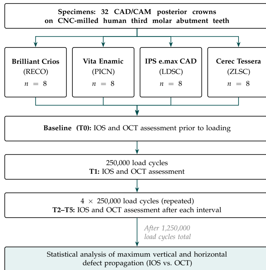
Figure 1. Schematic overview of the study protocol. CNC = computer numerical control; CAD/CAM = computer-aided design/computer-aided manufacturing; RECO = resin composite; PICN = polymer-infiltrated ceramic network; LDSC = lithium disilicate ceramic; ZLSC = zirconia-reinforced lithium silicate ceramic; IOS = intraoral scanning; OCT = optical coherence tomography.
