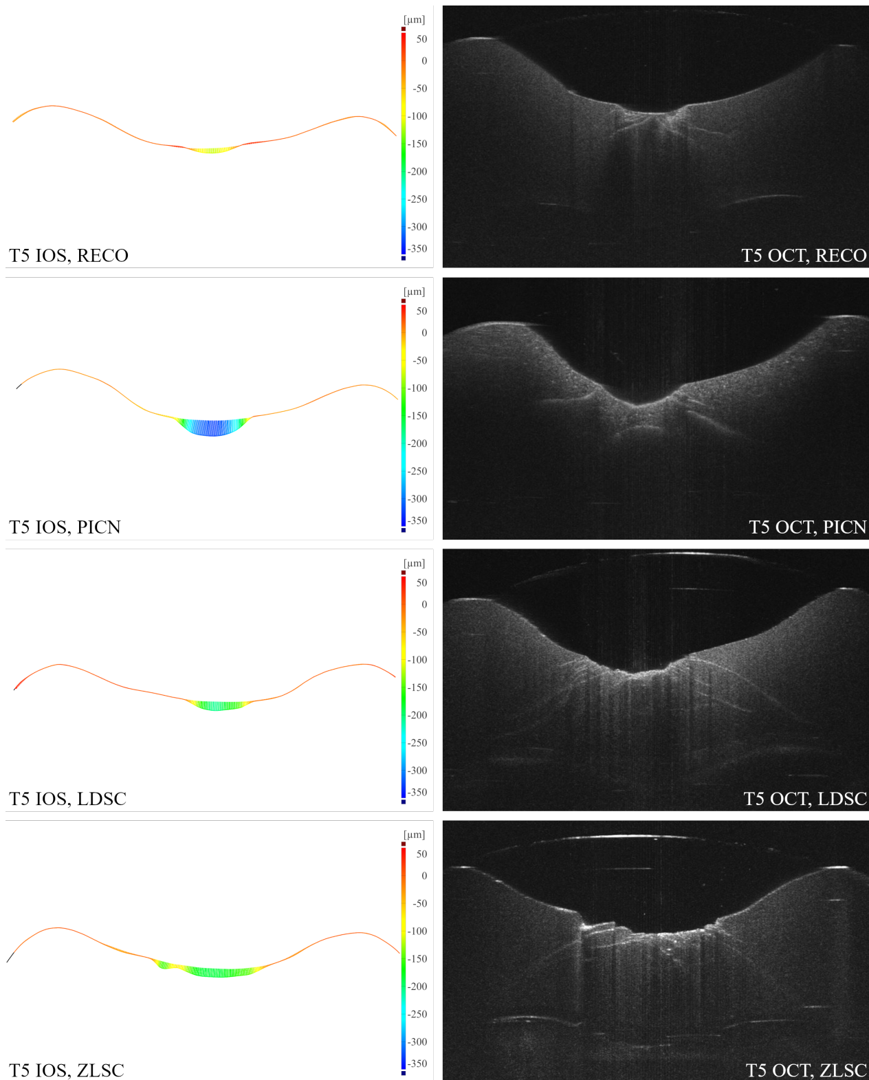
Figure 2. Comparison of surface wear and subsurface damage at T5 (after 1,250,000 load cycles) across all material classes; resin composite (RECO), polymer-infiltrated ceramic network (PICN), lithium disilicate ceramic (LDSC), and zirconia-reinforced lithium silicate ceramic (ZLSC). Left: Intraoral scanning (IOS) surface deviation maps referenced to T0. Right: Representative optical coherence tomography (OCT) cross-sections illustrating the qualitative extent and propagation of subsurface damage. Due to optical distortion caused by the water droplet used to reduce specular reflection and improve image contrast, the OCT images are intended for qualitative visualization only and do not provide reliable absolute spatial dimensions. RECO data previously reported in Kuhl et al. [1].
