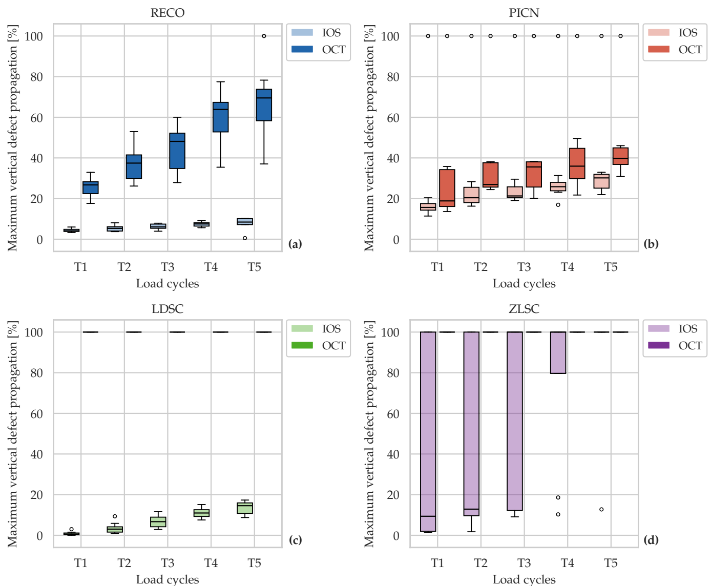
Figure 3. Maximum vertical defect propagation (%) by intraoral scanning (IOS, surface wear) and optical coherence tomography (OCT, subsurface damage) for four CAD/CAM crown materials: (a) resin composite (RECO, Brilliant Crios), (b) polymer-infiltrated ceramic network (PICN, Vita Enamic), (c) lithium disilicate ceramic (LDSC, IPS e.max CAD), and (d) zirconia-reinforced lithium silicate ceramic (ZLSC, Cerec Tessera). OCT values are normalized to local occlusal thickness and IOS values to a 1.5 mm reference. RECO data were previously reported in Kuhl et al. [1] and are included for cross-material comparison. Collapsed boxes (single horizontal line at 100%) indicate that all specimens within that group reached the maximum value, defined as either full-thickness cracking through the entire crown layer or catastrophic failure of the crown. Timepoints: after 250,000 (T1), 500,000 (T2), 750,000 (T3), 1,000,000 (T4), and 1,250,000 (T5) load cycles.
