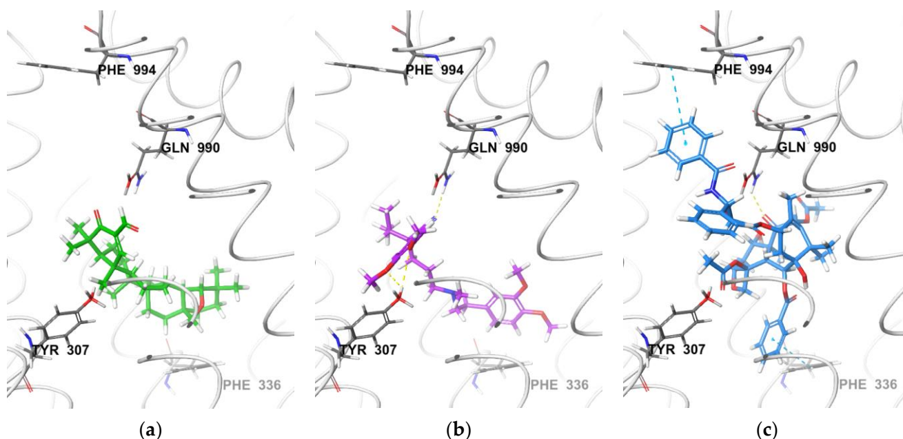
Figure 2. Comparison of the best GOLD docking conformations with human P-gp (PDB ID: 6QEX) for (a) OA; (b) verapamil; and (c) co-crystallized taxol.
