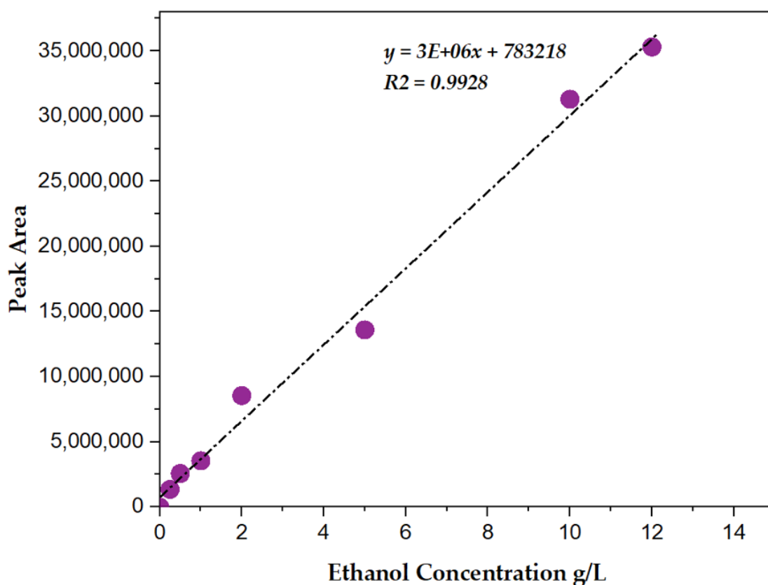
Figure 1. External calibration curve used for ethanol quantification by GC–MS. Purple circles represent the experimental calibration data, while the dashed line represents the linear regression fit.
