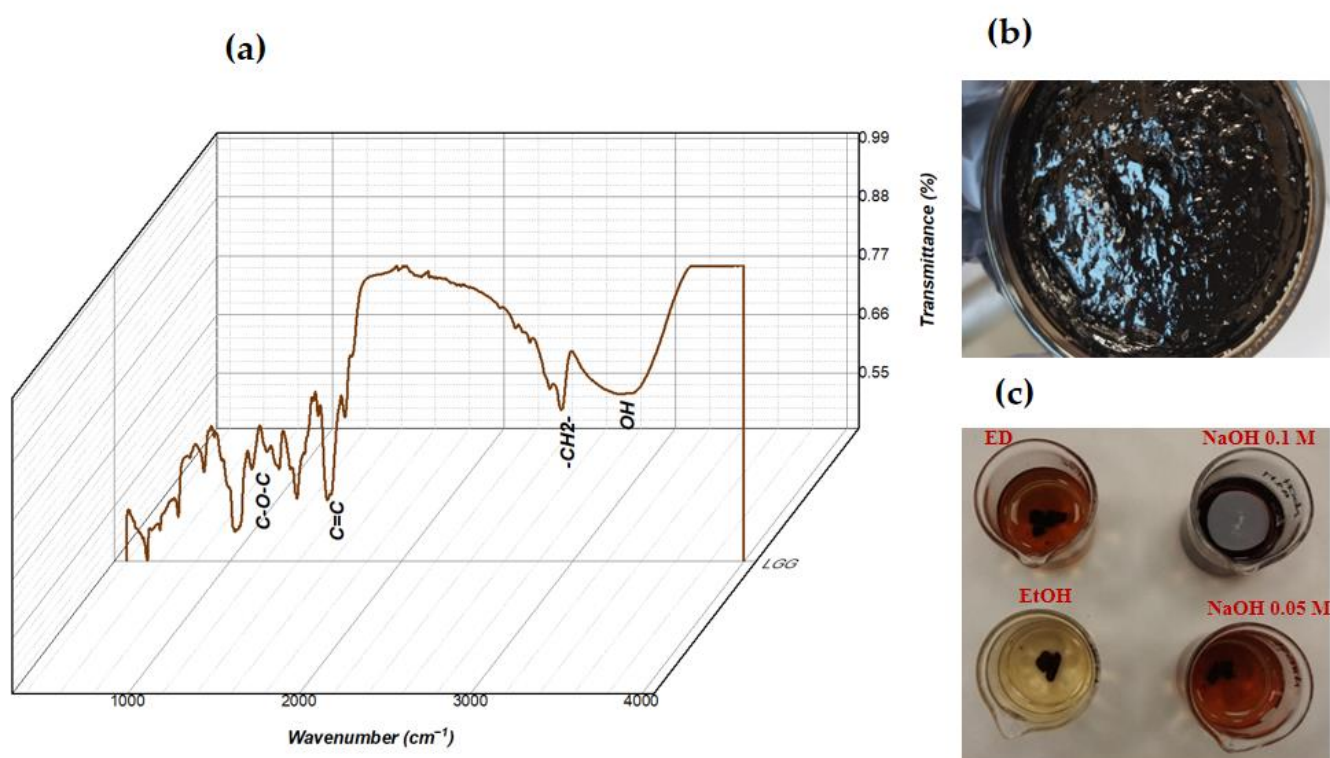
Figure 7. (a) FTIR spectrum of the lignin-based resin, (b) visual appearance of the synthesized resin, and (c) solubility of the resin in different solvents and alkaline solutions.
