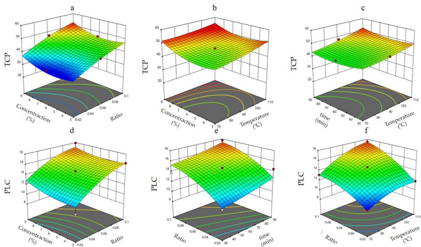
Figure 3. Three-dimensional response surface plots generated from the RSM models for TPC and PLC. The variables studied are temperature ( T , °C), NaOH concentration ( C , %), extraction time ( t , min), and solid-to-liquid ratio ( R , S/L). The response surfaces illustrate the interaction effects between the variables and their influence on TPC and PLC. Panels (a–c) represent the effects of the operating variables on TPC, while panels (d–f) show their effects on PLC.
