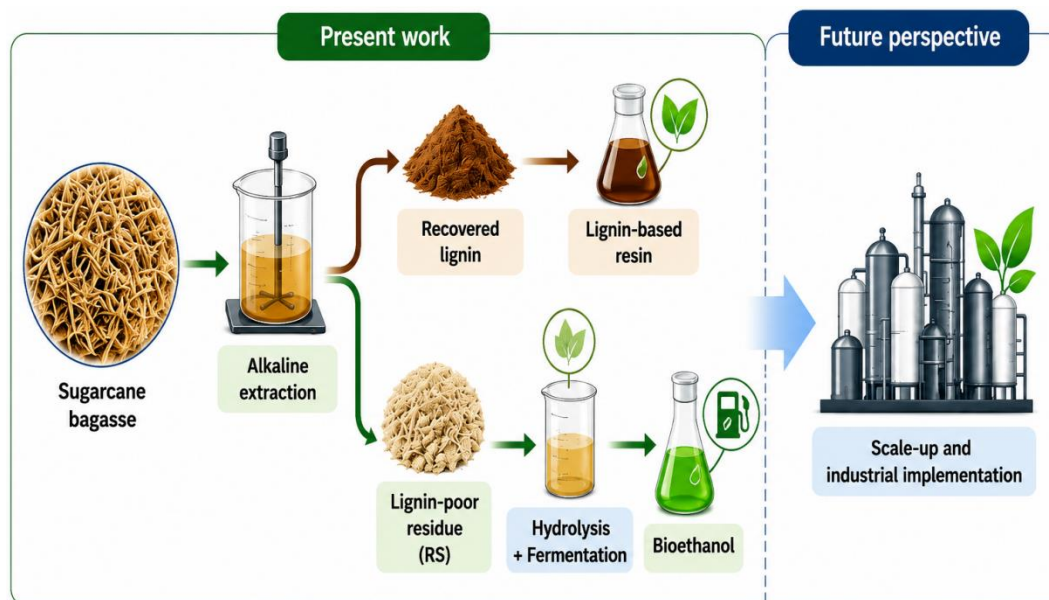
Figure 8. Schematic overview of the integrated valorization strategy proposed in this study, illustrating lignin recovery, lignin-based resin production, bioethanol generation from the lignin-poor residue, and the future perspective toward industrial implementation.
