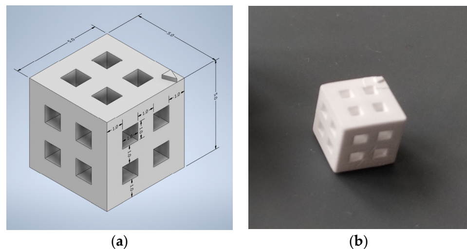
Figure 3. Virtual model of cube before oversizing process (a) and result after sintering (b).
