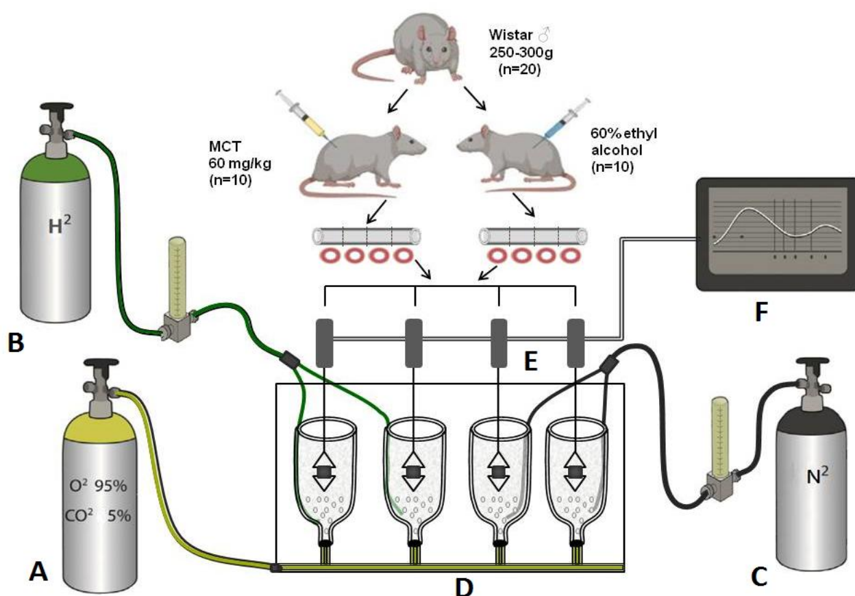
Figure 2. Study design and the scheme of the experimental setup. (A)—Gas mixture of oxygen (95%)/carbon dioxide (5%), (B)—Hydrogen 50 ppm, (C)—Nitrogen 100%, (D)—Four-chamber organ bath with Krebs solution and rat aortic rings, (E)—Force displacement transducer, (F)—Data acquisition system (PowerLab) and computer.
