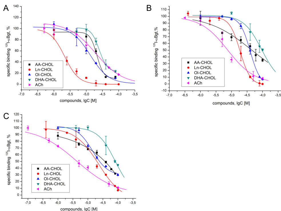
Figure 2. Competition of ^{125}\text{I} -labeled \alpha\text{Bgt} with acylcholines for binding to (A) L. stagnalis AChBP; (B) Torpedo californica nAChR; and (C) human \alpha 7 nAChR expressed in the GH4C1 cell line. \text{IC}_{50} values and 95% CIs are presented in Table 1. Each point is the mean \pm SEM value of two measurements for each concentration in two (for DHA-CHOL with T. californica and \alpha 7 nAChR) or three (all other cases) independent experiments.
