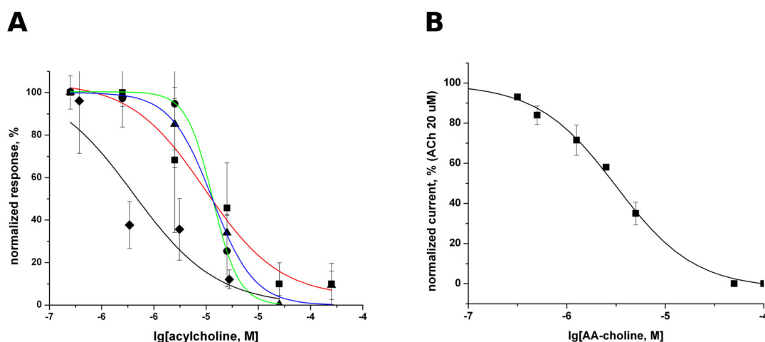
Figure 3. Inhibition of nAChR function by various acylcholines. (A) Inhibition curves for AA-CHOL (red line, squares), Ol-CHOL (blue line, triangles), Ln-CHOL (black line, diamonds), and DHA-CHOL (green line, circles) of \text{Ca}^{2+} influx evoked by acetylcholine in the presence of PNU 120596 on SH-SY5Y cell line. The \text{IC}_{50} values are listed in Table 2; (B) ACh evoked current in the mouse muscle nAChR expressed in Xenopus oocyte is inhibited by AA-CHOL at low micromolar concentrations ( \text{IC}_{50} 3.16 \pm 0.26 \mu\text{M} ).
