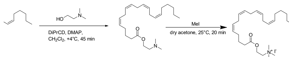
Scheme 1. Synthesis of acylcholines on the example of AA-CHOL: DiPrCD, diisopropyl carbodiimide; DMAP, N,N -dimethylaminopyridine [13].
