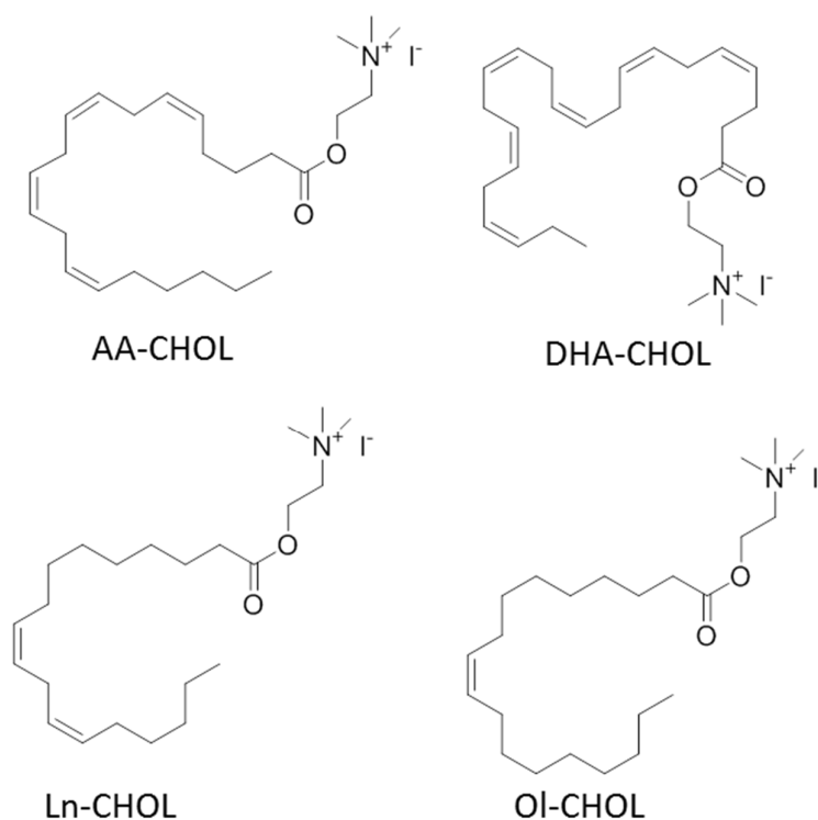
Figure 1. The structures of the synthesized acylcholines.
