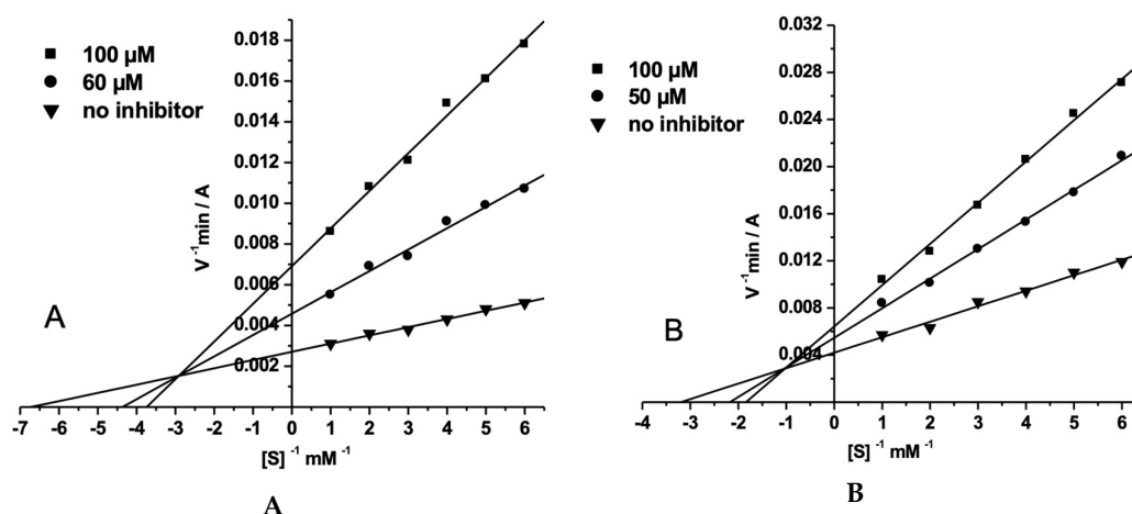
Figure 6. Lineweaver–Burk plots for steady state inhibition of AChE (A) and BChE (B) by AA-CHOL.
