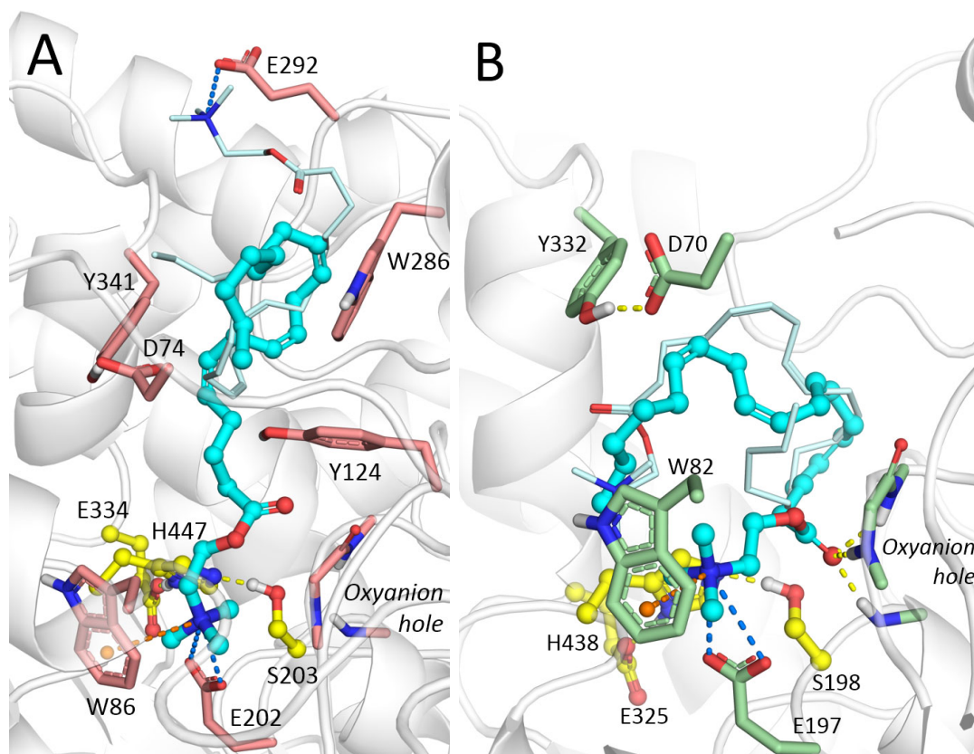
Figure 7. Docked poses of AA-CHOL inside (A) AChE and (B) BChE gorges. The best binding pose of AA-CHOL is shown with balls and sticks, carbon atoms colored cyan, poses in the PAS (for AChE) and outside active site (for BChE) are shown with lines, carbon atoms colored pale cyan.
