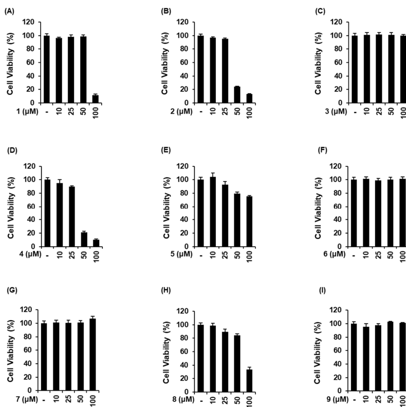
Figure 2. Comparison in the effects of 9 sesquiterpenes isolated from Artemisia argyi in LLC-PK1 cells. (A–I) Cells were exposed to nine sesquiterpene compounds including (A) moxartenolide (compound 1), (B) dehydromatricarin A (compound 2), (C) tuberiferin (compound 3), (D) argyrolide G (compound 4), (E) deacetylmaticarin (compound 5), (F) rupicolin A (compound 6), (G) acrifolide (compound 7), (H) 3- epi -iso- seco -tanaparthalide (compound 8), and (I) iso- seco -tanaparthalide (compound 9), and cell viability was measured using an Ez-Cytox cell viability assay kit (mean \pm SD, n = 3 , * p < 0.05 compared with untreated LLC-PK1 cells).
