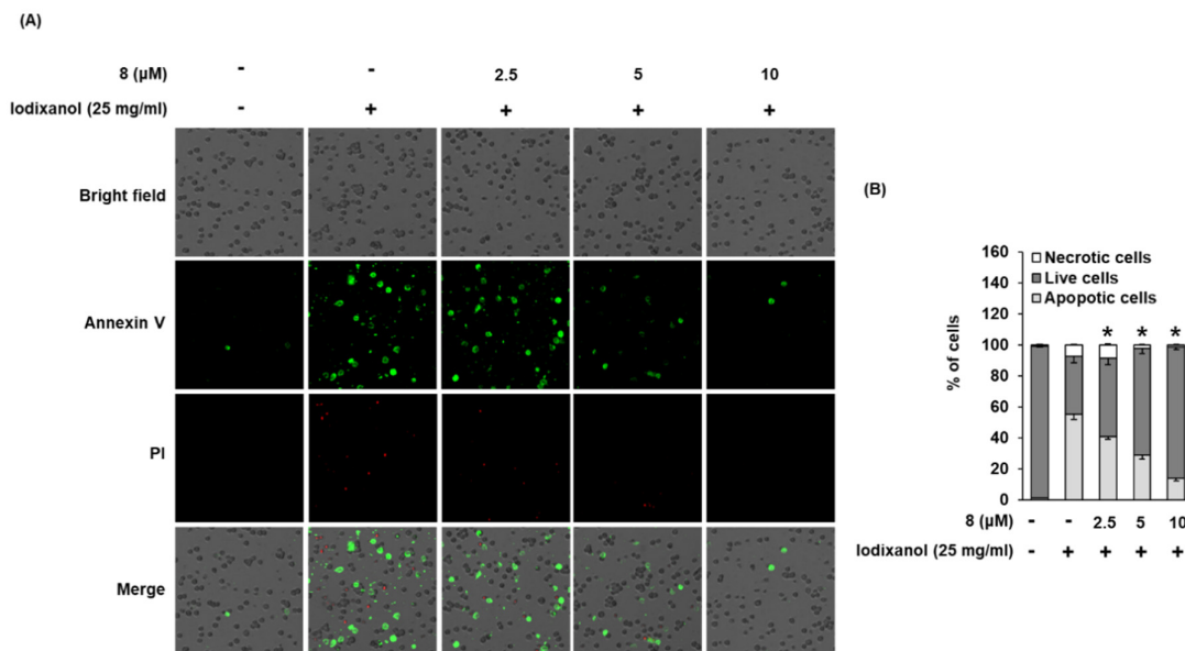
Figure 7. Effect of 3- epi -iso- seco -tanapartholide (compound 8 ) isolated from Artemisia argyi on iodixanol-induced apoptosis in LLC-PK1 cells. (A) Cells were treated to 25 mg/mL of iodixanol in the presence or absence of compound 8 for 24 h, and stained with annexin V Alexa Fluor 488 (green fluorescence) and PI (red fluorescence). Images were quantitatively determined using a Tali image-based cytometer. (B) The percentages of apoptotic, necrotic, and live cells are represented as a bar graph (mean \pm SD, n = 3 , * p < 0.05 compared with iodixanol-treated LLC-PK1 cells).
