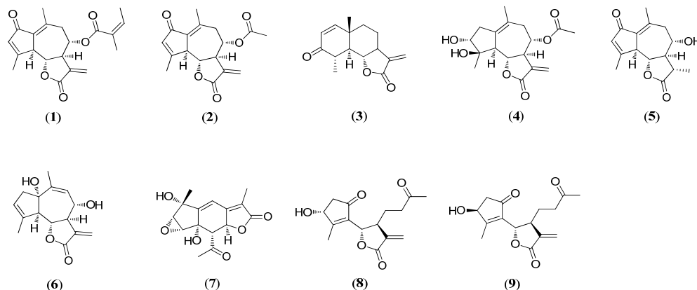
Figure 1. Chemical structures of nine sesquiterpenes including moxartenolide (compound 1 ), dehydromatricarin A (compound 2 ), tuberiferin (compound 3 ), argyinolide G (compound 4 ), deacetylmatricarin (compound 5 ), rupicolin A (compound 6 ), acrifolide (compound 7 ), 3- epi -iso- seco -tanaparthalide (compound 8 ), and iso- seco -tanaparthalide (compound 9 ) isolated from Artemisia argyi .
