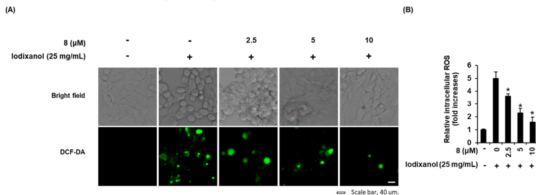
Figure 4. Effects of 3- epi-iso-seco-tanapartholide (compound 8 ) isolated from Artemisia argyi on iodixanol-induced morphological changes and ROS generation in LLC-PK1 cells. (A) Cells were exposed to 25 mg/mL of iodixanol in the absence or presence of compound 8 and stained with H 2 DCFDA. The fold-increases of intracellular ROS levels detected by DCF fluorescence (green fluorescence) are represented as a bar graph (mean \pm SD, n = 3 , * p < 0.05 compared with iodixanol-treated LLC-PK1 cells). (B) Representative bright field and fluorescence images were obtained using an IX50 fluorescence microscope. White scale bar, 40 \mu m.
