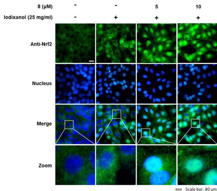
Figure 6. The effects of 3- epi -iso- seco -tanapartholide (compound 8) on the nuclear translocation of Nrf2 in LLC-PK1 cells exposed to iodixanol. LLC-PK1 cells were treated with 25 mg/mL iodixanol in the presence or absence of 8, and immunofluorescence staining was performed using antibodies for Nrf2 that were visualized with a goat anti-rabbit IgG-heavy- and light-chain FITC-conjugated antibody (green fluorescence) and mounted with ProLong® Gold antifade reagent with DAPI-stained nuclei (DAPI). The white arrows indicate the presence of Nrf2. White scale bar, 40 \mu m.
