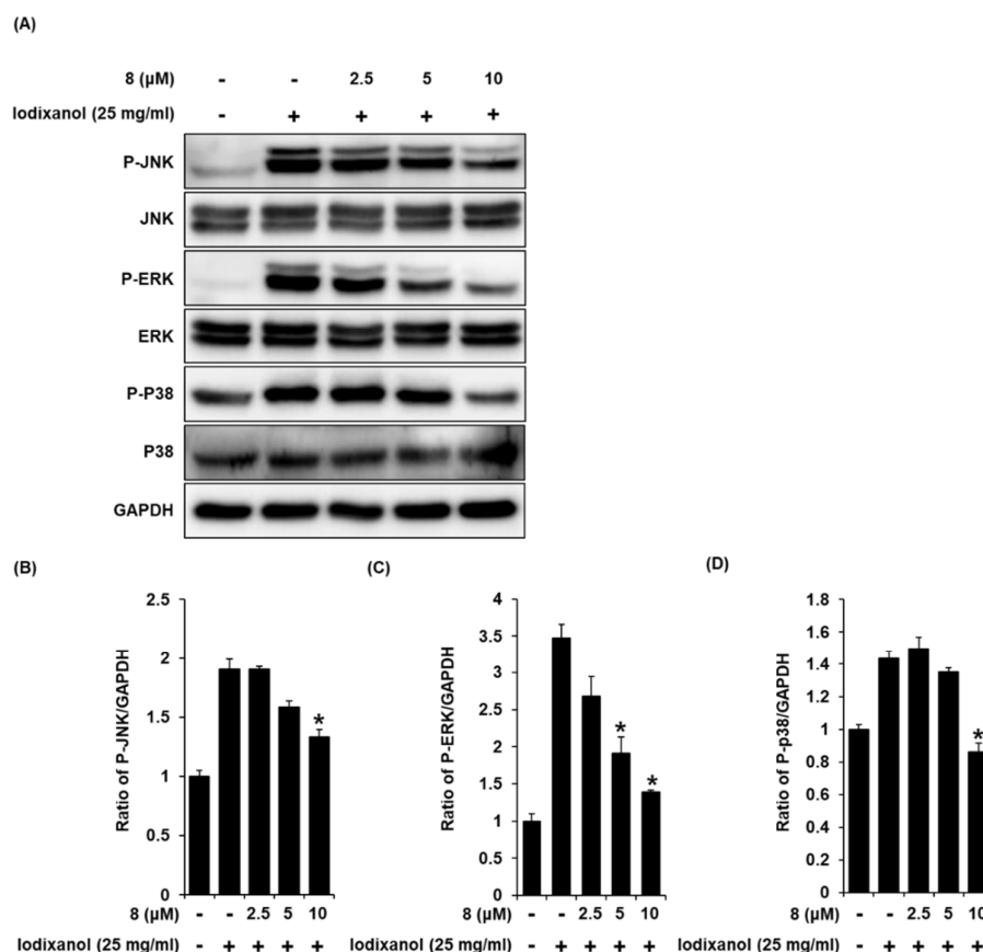
Figure 9. The effects of 3- epi -iso- seco -tanapharholide (compound 8 ) on the expression of JNK, ERK, p38 proteins associated with MAPK pathways in LLC-PK1 cells treated with iodixanol. (A) LLC-PK1 cells were treated with 25 mg/mL iodixanol in the absence or presence of compound 8 , and western blot analysis was performed using antibodies for P-JNK, JNK, P-ERK, ERK, P-P38, P38, and GAPDH. (B–D) The ratios of JNK, ERK, and P38 phosphorylation compared with untreated cells are represented as a bar graph (mean \pm SD, n = 3 , * p < 0.05 compared with iodixanol-treated LLC-PK1 cells).
