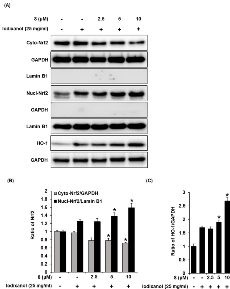
Figure 5. The effect of 3- epi -iso- seco -tanapartholide (compound 8) on the nuclear expression of Nrf2 and HO-1 proteins associated with antioxidant pathways in LLC-PK1 cells exposed to iodixanol. (A) LLC-PK1 cells were treated with 25 mg/mL iodixanol in the absence or presence of 8, and western blot analysis was conducted using antibodies for Nrf2, Lamin B1, HO-1, and glyceraldehyde 3-phosphate dehydrogenase (GAPDH). Lamin B1 and GAPDH were used as a cytosolic and nuclear controls for western blot analysis, respectively. (B and C) The ratios of nuclear Nrf2, cytosolic Nrf2, and HO-1 compared with untreated cells are represented as a bar graph (mean \pm SD, n = 3 , * p < 0.05 compared with iodixanol-treated LLC-PK1 cells).
