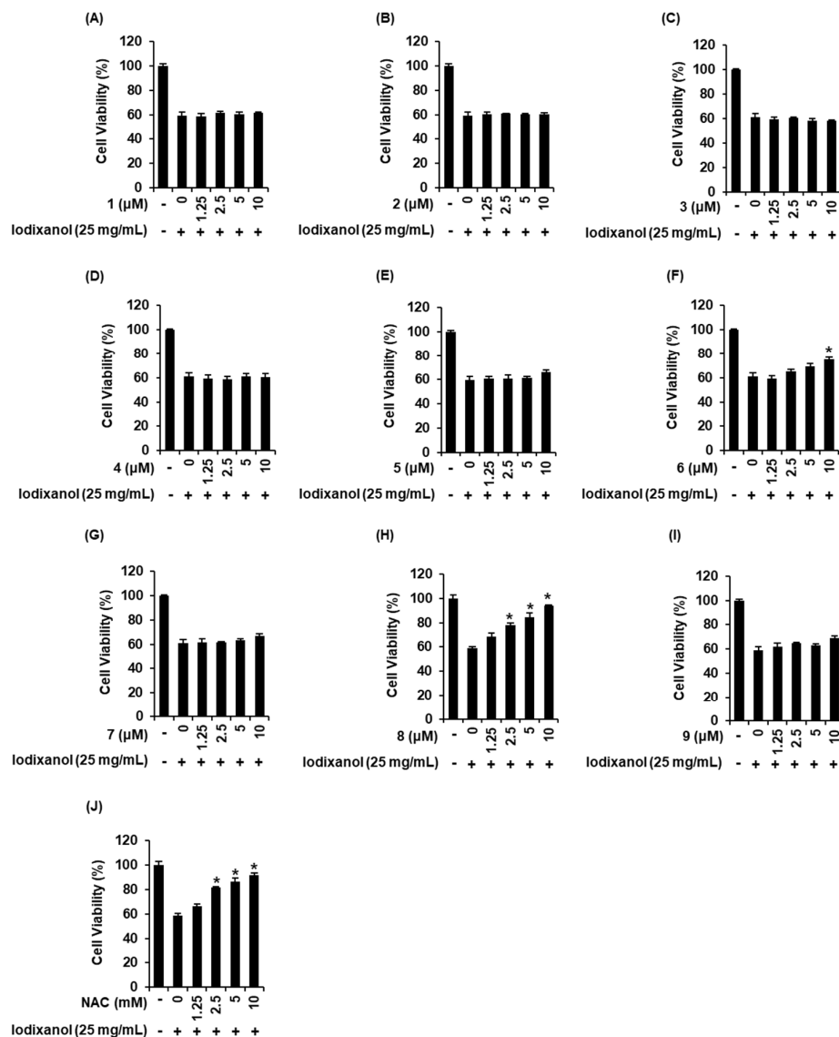
Figure 3. Comparison in the protective effects of nine sesquiterpenes isolated from Artemisia argyi on iodixanol-induced cytotoxicity in LLC-PK1 cells. (A–J) Cells were exposed to 25 mg/mL iodixanol in the presence or absence of nine sesquiterpene compounds including (A) moxartenolide (compound 1), (B) dehydromatricarin A (compound 2), (C) tuberiferin (compound 3), (D) argyrolide G (compound 4), (E) deacetylmaticarin (compound 5), (F) rupicolin A (compound 6), (G) acrifolide (compound 7), (H) 3-epi-iso-seco-tanapartholide (compound 8), and (I) iso-seco-tanapartholide (compound 9) and (J) N-acetyl cysteine (NAC) and cell viability was measured using an Ez-Cytox cell viability assay kit (mean \pm SD, n = 3 , * p < 0.05 compared with iodixanol-treated LLC-PK1 cells).
