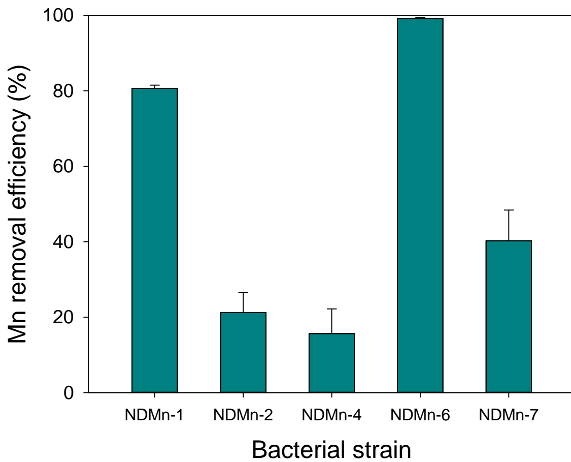
Fig. S2 Comparison of Mn removal efficiency by five isolated strains
