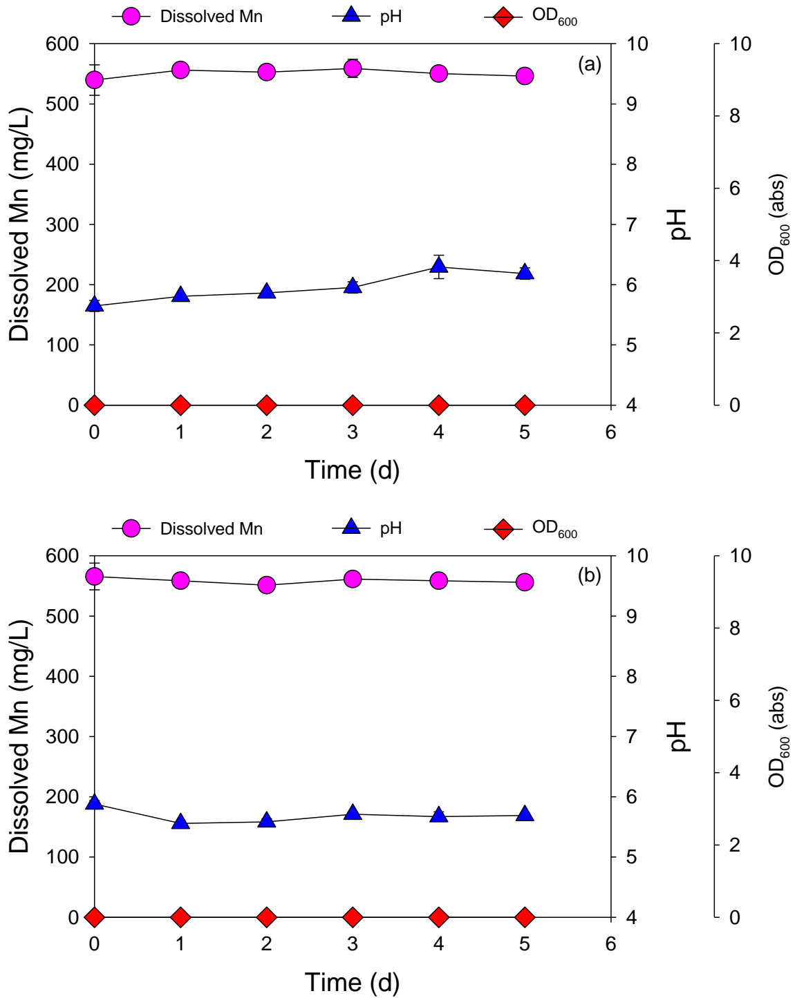
Fig. S1 Changes of dissolved Mn, pH, and OD of abiotic control basal salt medium (a) and nutrient broth medium (b).
