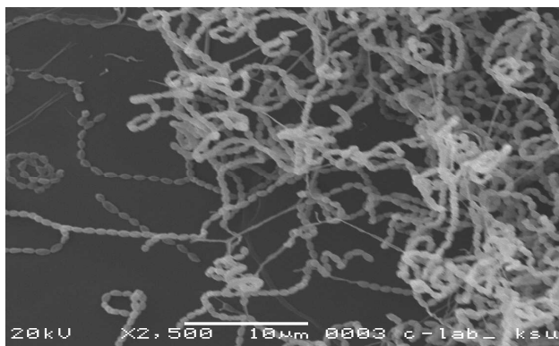
Figure 1. Scanning electron micrograph of actinomycete isolate 2 as a representative photo of the Streptomyces isolates used in this study (2500×).
