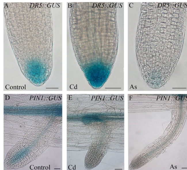
Figure 2. Expression patterns of DR5::GUS and PIN1::GUS in lateral roots (LRs) of Arabidopsis DR5::GUS and PIN1::GUS seedlings non-exposed (Control, (A,D)) or exposed to 60 \mu M CdSO 4 (Cd, (B,E)) or 400 \mu M Na 2 HAsO 4 ·7H 2 O (As, (C,F)). Bars = 20 \mu m (A–C), 30 \mu m (D) and 50 \mu m (E–F).
