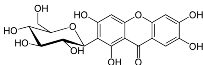
Figure 1. Molecular structure of mangiferin.
