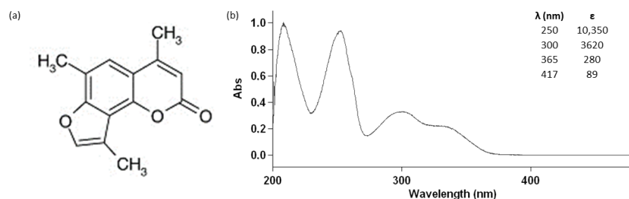
Figure 1. Chemical structure (a) and absorption spectrum (b) of 4,6,4'-trimethylangelicin (TMA) and its molar extinction coefficients at 250 nm, 300 nm, 365 nm, and 417 nm.
