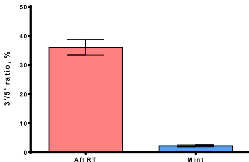
Figure 9. The 5'/3'-ratio of cDNA synthesized by Afl RT and M-MuLV RT. MS2 genomic RNA (3569 nt) served as a template for reverse transcription. Each reaction was run in three technical repeats. The 5'/3'-ratio of cDNA ends was determined using ddPCR with primers for 5'- and 3'-ends of MS2 genomic RNA.
