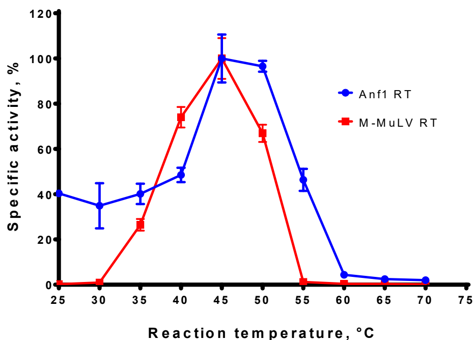
Figure 3. Optimal temperature assay. The optimal temperature for RTs was determined in RT activity assay using radioactively labeled oligo(dT) 40 primer in poly(rA)/oligo(dT) 40 substrate. Each experiment was triplicated.
