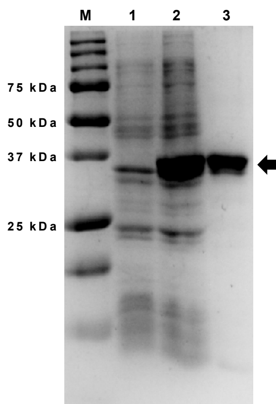
Figure 2. Expression and purification of Afl RT. The enzyme was expressed in E. coli strain BL-21 (DE3) pLysS and purified using affinity and ion-exchange chromatography. Lane assignment: M—Precision Plus Protein standards (Bio-Rad, Hercules, CA, USA), 1— E. coli lysate before expression of Afl RT, 2—crude lysate after expression, 3—purified Afl RT. Afl RT is marked with an arrow. Original images can be found in Figure S1.
