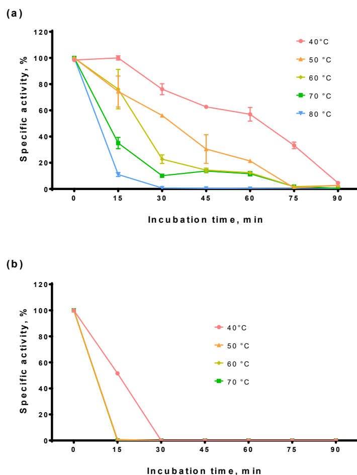
Figure 4. Thermostability assay. (a) —Afl RT, (b) —M-MuLV RT. Enzymes were incubated at 40–80 °C for up to 90 min following RT activity assay using radioactively labeled oligo(dT) 40 primer in poly(rA)/oligo(dT) 40 substrate. Each experiment was triplicated.
