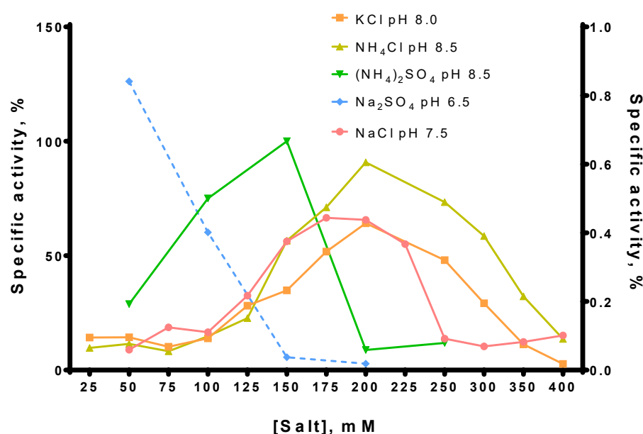
Figure 6. Comparison of optimal salts and pH for Afl RT. RT activity assay with radioactively labeled oligo(dT) 40 primer in poly(rA)/oligo(dT) 40 substrate. The dashed line (Na 2 SO 4 , pH 6.5) belongs to the right Y-axis.
