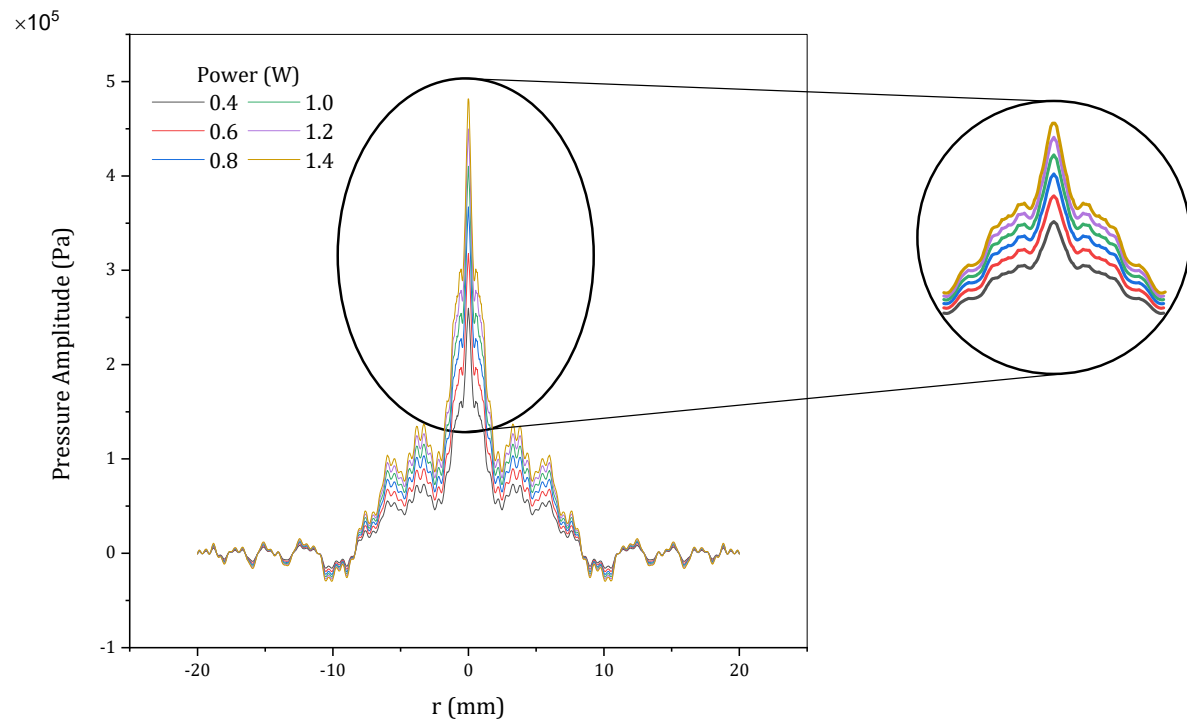
Figure 7. Pressure amplitude along the radial axis at various acoustic powers, obtained from the numerical model.
