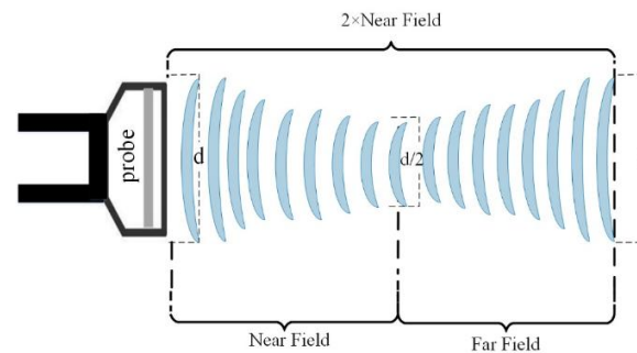
Figure 1. Illustration of the near-field, Fresnel, and Fraunhofer regions of a linear probe, with d as the probe diameter.
