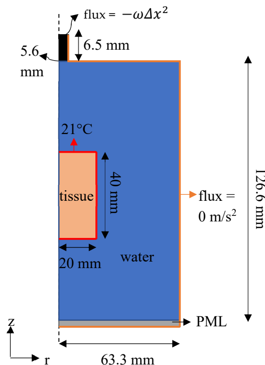
Figure 3. Schematic of the geometry of the model and boundary conditions.
