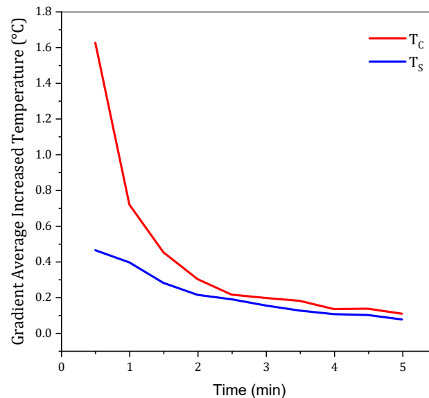
Figure 6. Graph of the T_c and T_s gradients.
