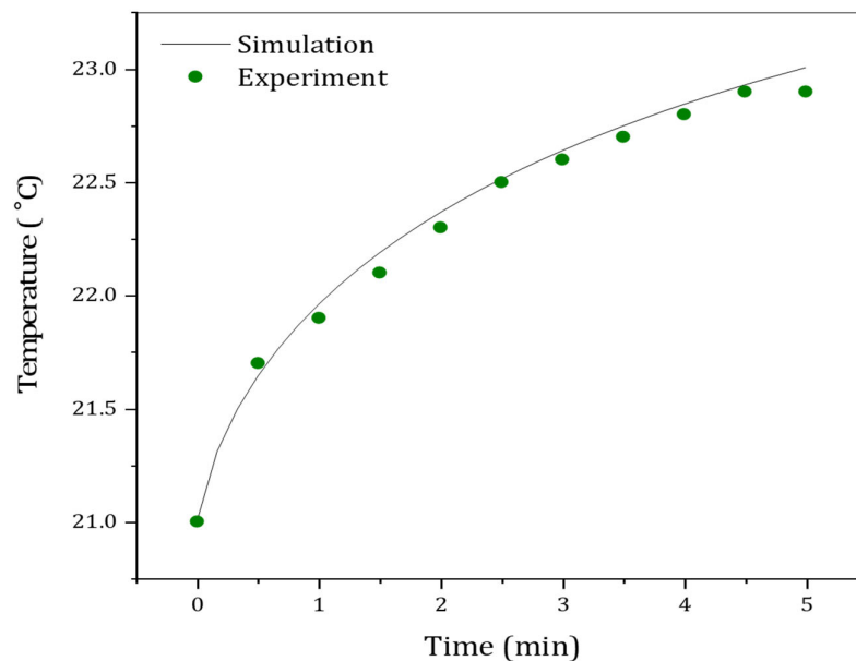
Figure 10. Comparison of the time-dependent temperature of the center of the tissue obtained from the numerical simulation and from the experiment.
