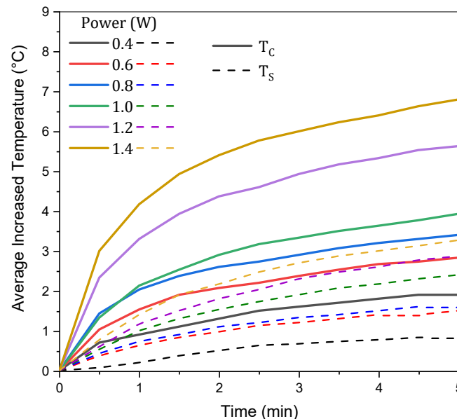
Figure 5. The increases in temperature with 3 MHz ultrasound beams with powers of 0.4–1.4 W at T_c and T_s .
