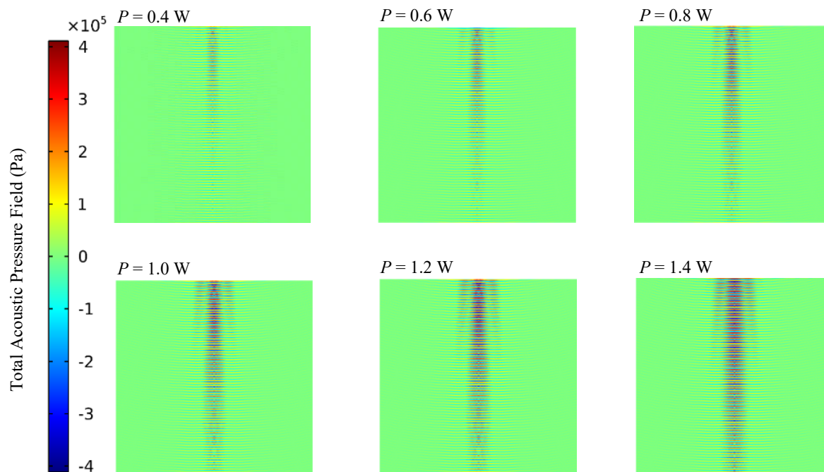
Figure 8. Simulated acoustic pressure distribution within tissues at t = 5 min for different transducer power levels, predicted by the numerical model.
