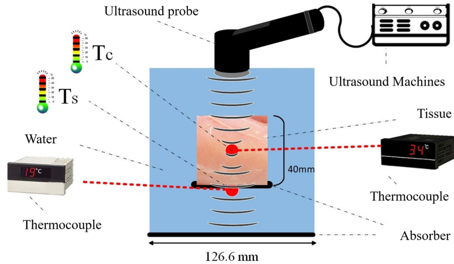
Figure 2. A schematic representation of the experiment showing the locations of the tissue, thermocouples, and ultrasound probe.
