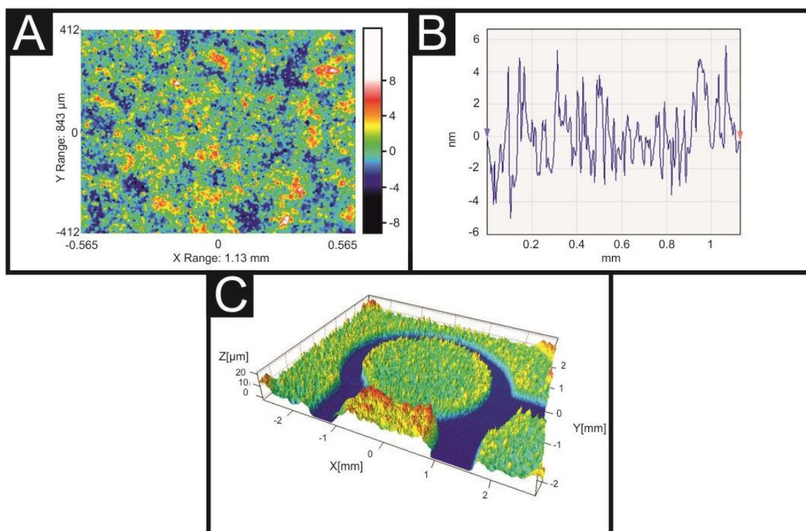
Figure S1. Topography measurement on a screen-printed electrode (A), height profile (B) from data shown in A and a 3D plot of the topography measurements (C).
