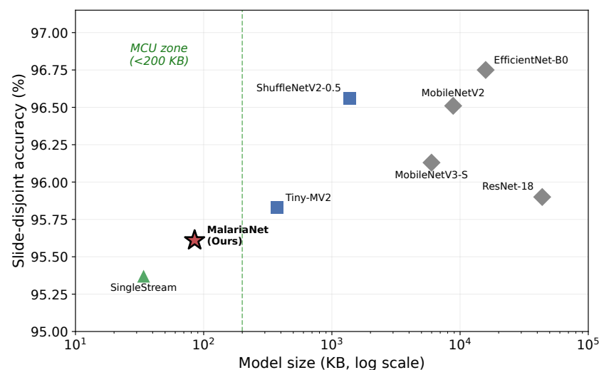
Figure 8. Leakage-free (slide-disjoint) accuracy vs. model size (3-seed mean). Green zone: MCU-deployable (<200 KB). Under rigorous evaluation, MalariaNet is the most accurate model in the deployable zone but sits \approx 1 pp below the larger baselines, corresponding to a compactness/accuracy trade-off, not the “matches large models” picture the per-cell protocol produced.
