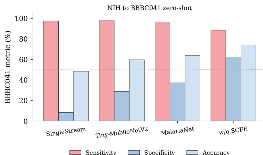
Figure 5. Zero-shot NIH to BBBC041 transfer (per-cell-trained models, no fine-tuning). All models keep high sensitivity but collapse in specificity off-domain. The apparent left-to-right ordering is a per-cell training pattern that does not survive slide-disjoint training (Section 4.8); we draw no architectural conclusion from it. The robust message is that no compact model transfers acceptably to the unseen species without target-site adaptation. The dashed horizontal line marks the 50% chance level.
