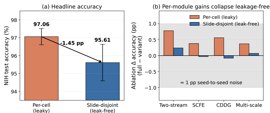
Figure 7. Slide leakage inflates accuracy and distorts ablation conclusions. (a) Headline NIH accuracy, per-cell vs. slide-disjoint (3-seed mean \pm std). (b) Per-module ablation \Delta (full – variant): large under per-cell splitting, collapsing into seed noise (grey band) and partly inverting under slide-disjoint evaluation.
