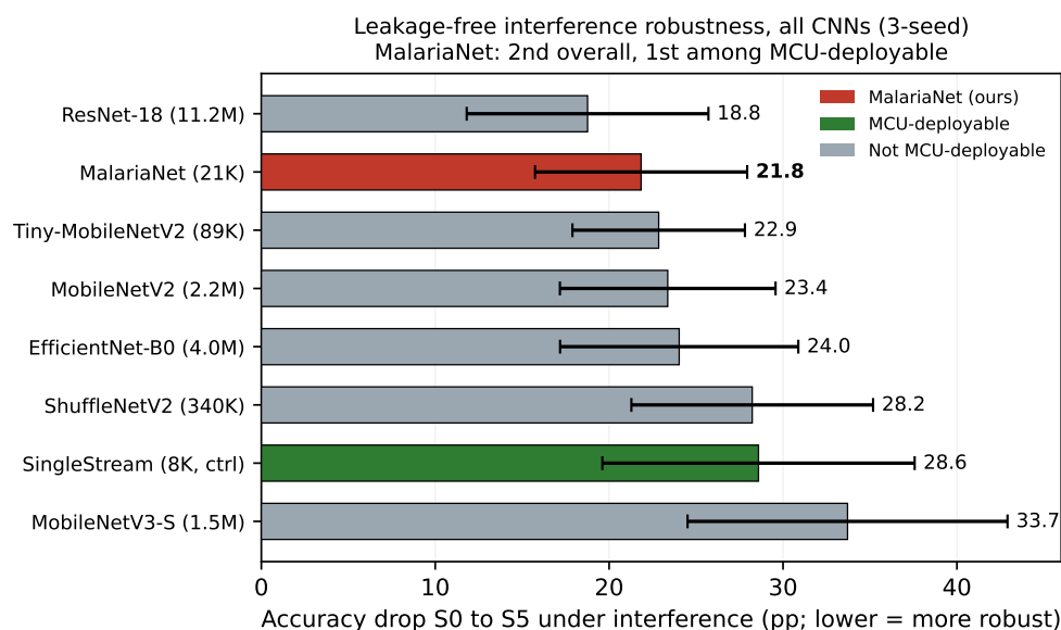
Figure 6. Leakage-free interference robustness across all eight CNNs (slide-disjoint, 3-seed; error bars = seed std). MalariaNet (red) is the second most robust overall and the most robust MCU-deployable model; SingleStream (the deployable control) is among the least robust.
