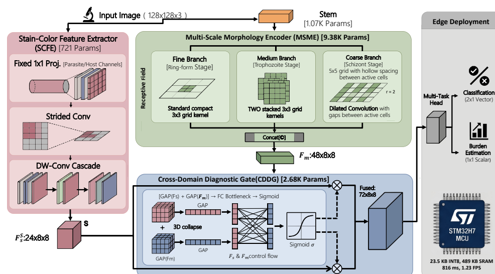
Figure 1. Architecture of MalariaNet. Two parallel streams (SCFE and MSME) are fused via CDDG for multi-task output.
