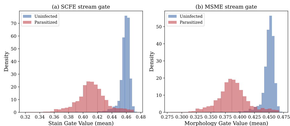
Figure 10. CDDG gate-value distribution (transparency only): the gate takes differentiated values for parasitized vs. uninfected cells, but this does not translate into a measurable accuracy gain under leakage-free evaluation (Section 4.4).
