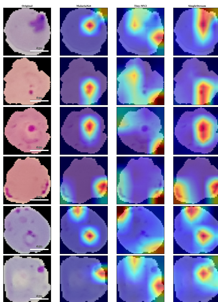
Figure 9. Grad-CAM++ on parasitized cells (qualitative). Columns: original, MalariaNet, Tiny-MV2, and SingleStream; each row is one cell shown across the methods, so a row shares the same scale. All panels are shown at the 128 \times 128 model-input resolution. As in Figure 3, the white bar is an approximate \sim 5 \mu\text{m} reference, and the absolute scale varies between rows because cells are individually segmented and resized. Warmer colours indicate higher class-discriminative activation.
