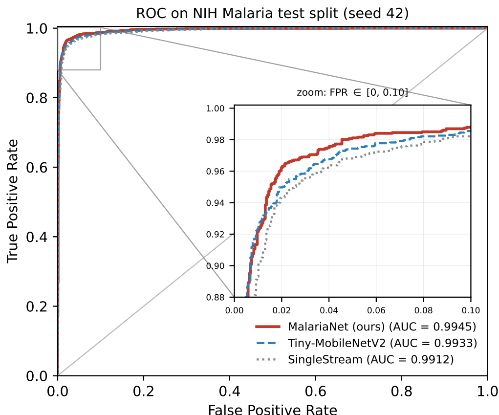
Figure 4. ROC on the NIH test split with the per-cell protocol (optimistic, seed 42), retained for comparability with prior work. Per-cell AUCs are inflated relative to the slide-disjoint values (MalariaNet, 0.988 \pm 0.003 ; Table 3); the small inter-model gaps shown here do not survive leakage-free evaluation and are not used to claim superiority. The grey diagonal marks chance (AUC 0.5); the inset zooms into the low-false-positive region ( \text{FPR} \leq 0.10 ), where the otherwise-overlapping curves separate.
