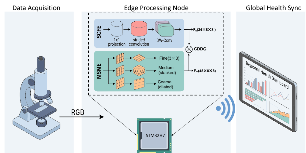
Figure 11. Point-of-care edge deployment concept. Only the on-device single-cell classification stage (STM32H743, measured 816 ms per 128 \times 128 cell) is validated; image acquisition, connectivity and aggregation are shown as concepts. Device power was not measured; the bill of materials is an estimate.
