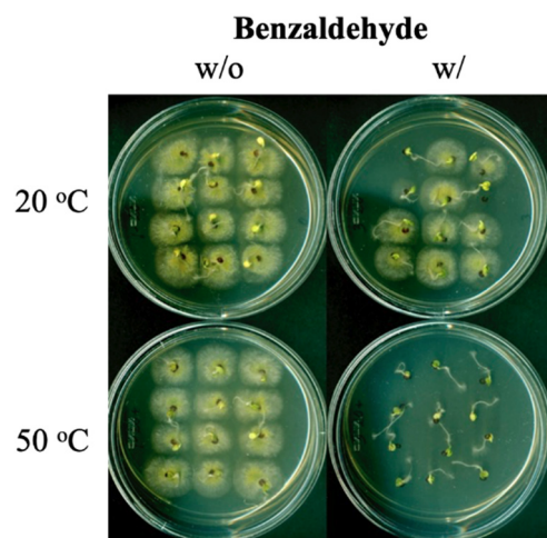
Figure 2. Representative assay showing enhanced seed sanitation via benzaldehyde-mediated heat sensitization (hurdle technology). Co-treatment of benzaldehyde at 3 mM and mild heat (50 °C) for 20 min completely inhibited the growth of A. flavus on the surface of seeds while the frequency of seed germination was unaffected.
