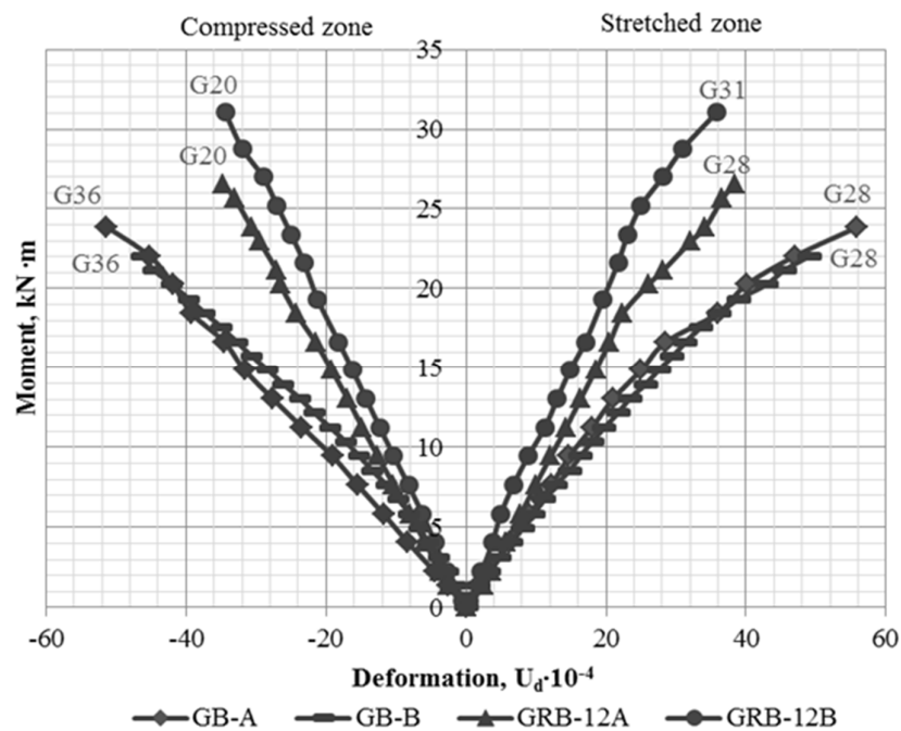
Figure 7. Graphical charts of deformations of most stressed fibers of wood in GB-A, GB-B, GRB-12A, and GRB-12B beams.
