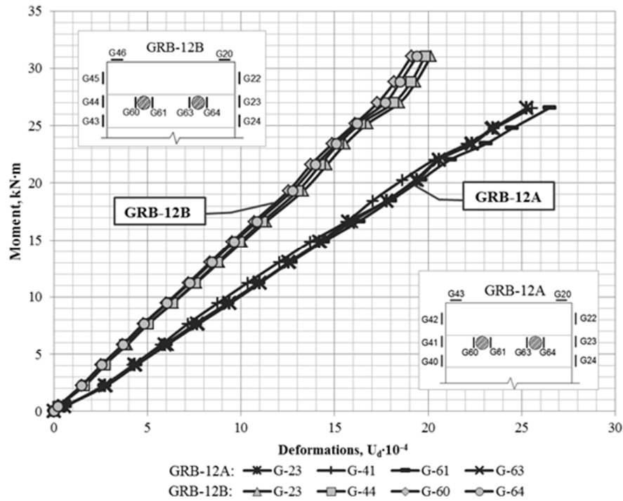
Figure 6. Graphical charts of wood- and steel-reinforcement deformations of GRB-12A and GRB-12B beams.
