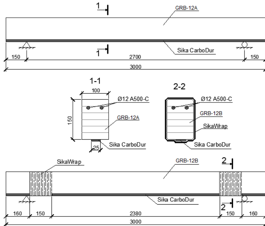
Figure 1. Scheme of reinforcing beams by means of metal and composite reinforcement.
