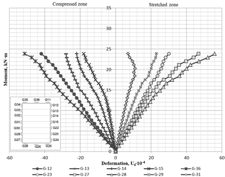
Figure 3. Graphical chart of layer deformation of cross-section fibers of GB-A beam in span middle.
