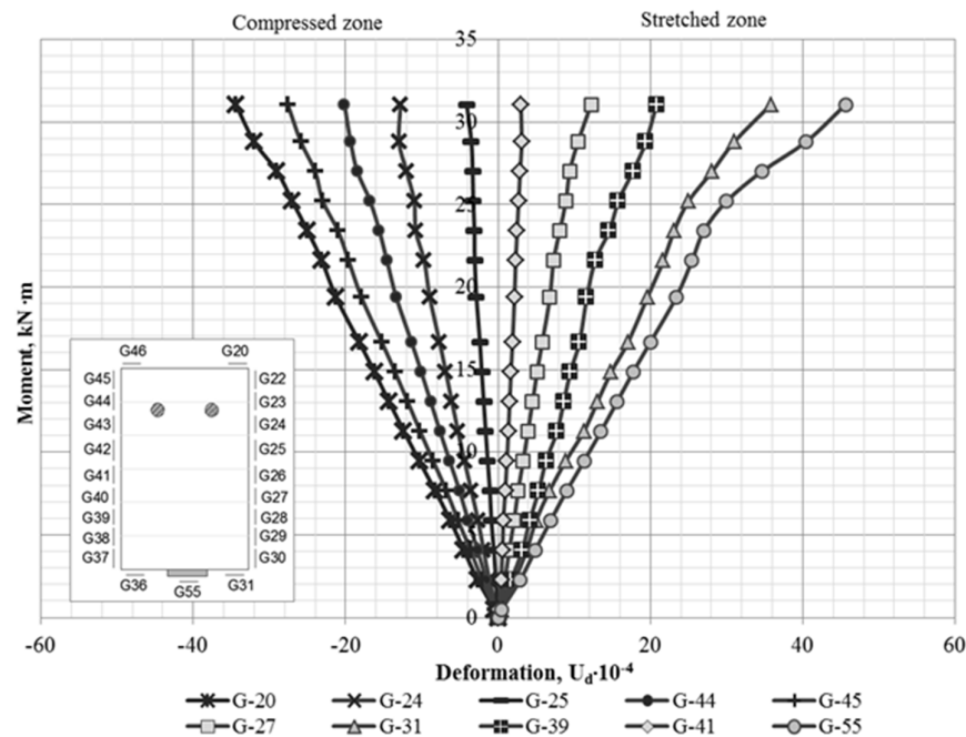
Figure 5. Graphical chart of layer deformation of sample cross-section fibers of GRB-12B beam in span middle.
