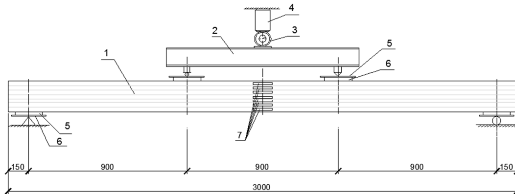
Figure 2. Scheme of experiment plant for testing beams made from glued laminated wood under bending: (1) studied beam; (2) metal traverse; (3) dynamometer; (4) jack; (5) metal plate; (6) wooden plate; (7) strain sensors.
