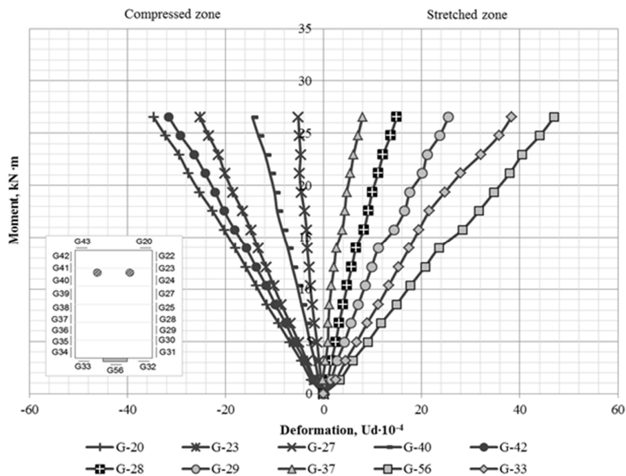
Figure 4. Graphical chart of layer deformation of cross-section fibers of GRB-12A beam in span middle.
