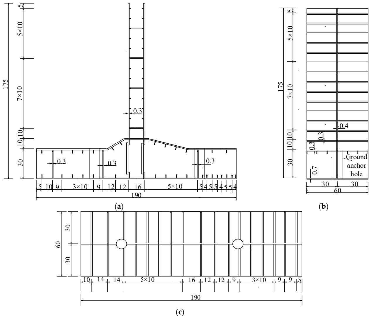
Figure 3. Design details of the T-shaped specimen (unit: cm). (a) Front view; (b) side view; (c) top view.
