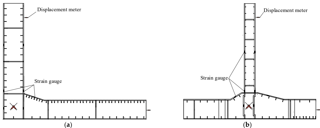
Figure 8. Specimen measurement point layout plan. (a) L-shaped specimen; (b) T-shaped specimen.
