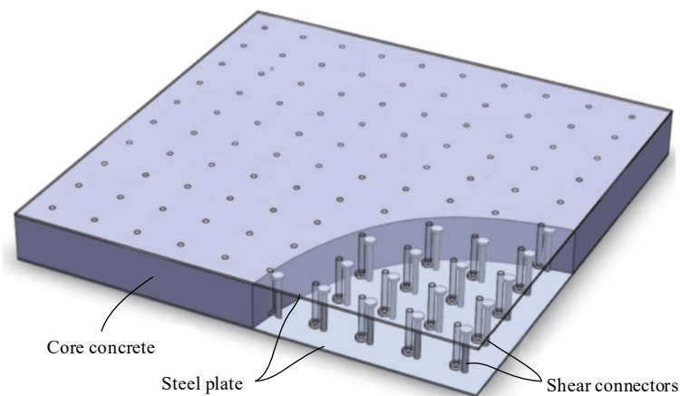
Figure 1. Double steel plate–concrete combination structure.
