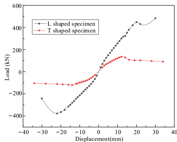
Figure 12. Specimen skeleton curve.
