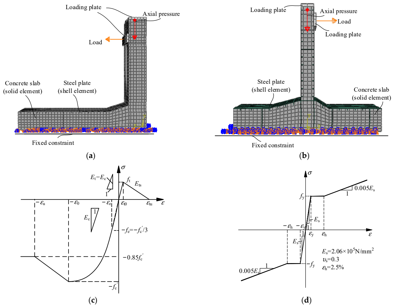
Figure 15. Finite element model of the specimen and material ontology. (a) L-shaped specimen; (b) T-shaped specimen; (c) concrete principal structure; (d) steel principal structure.
