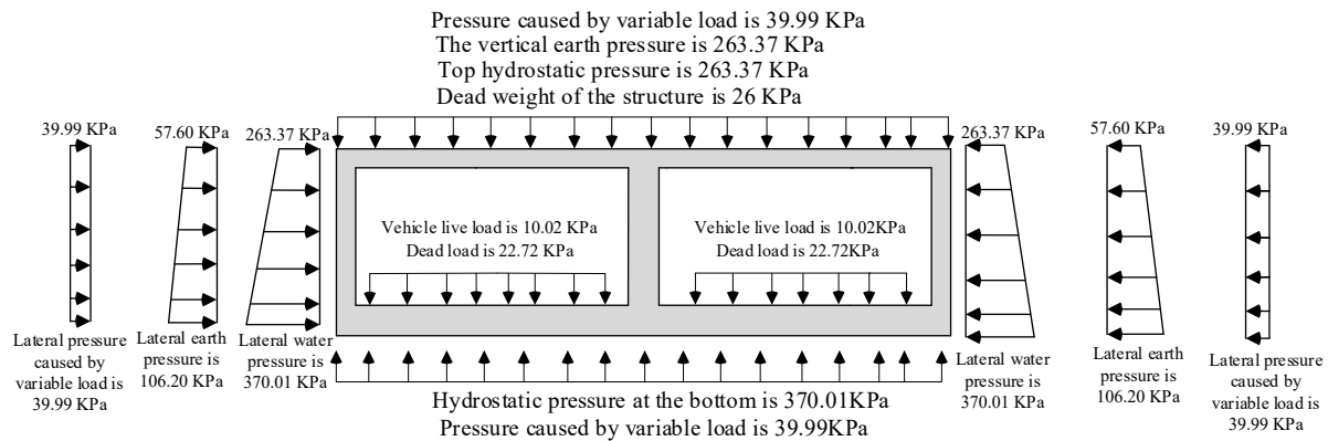
Figure 5. Schematic diagram of the load conditions.
