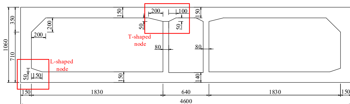
Figure 2. Cross section of the immersed tunnel (unit: cm).
