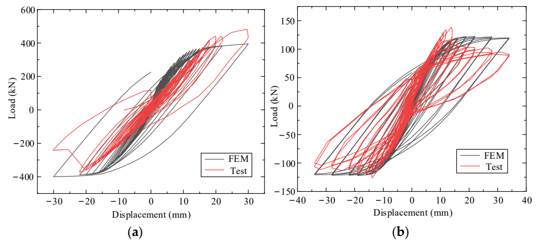
Figure 16. Comparison of the measured and calculated load displacement curves. (a) Shaped specimen; (b) shaped specimen.
