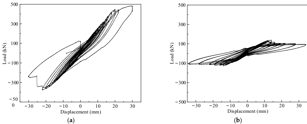
Figure 11. Hysteresis curve of the specimen. (a) L-shaped specimen; (b) T-shaped specimen.
