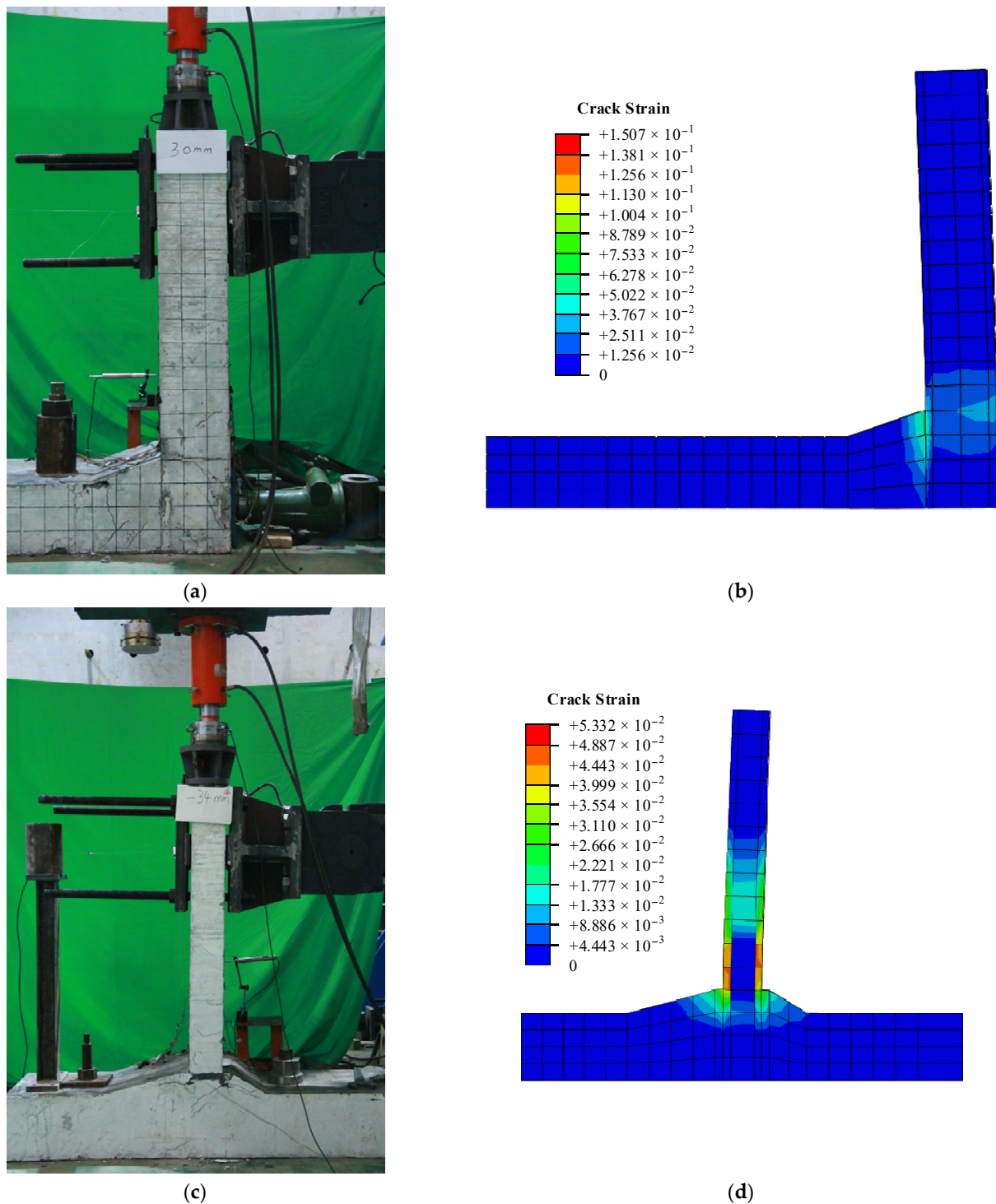
Figure 17. Comparison of the measured and calculated results of the crack distributions of specimens. (a) L-shaped specimen test phenomenon (30 mm); (b) calculated results for the L-shaped specimen (30 mm); (c) T-shaped specimen test phenomenon (-34 mm); (d) calculated results for the T-shaped specimen (-34 mm).
