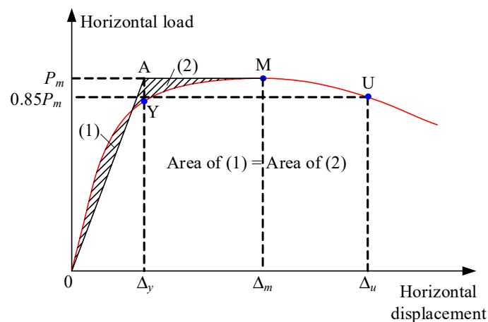
Figure 13. Equivalent yield point calculation diagram.
