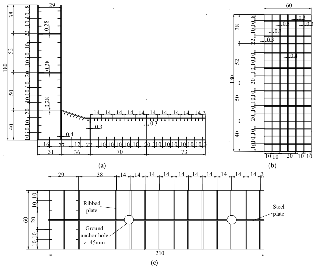
Figure 4. Design details of the L-shaped specimen (unit: cm). (a) Front view; (b) side view; (c) top view.
