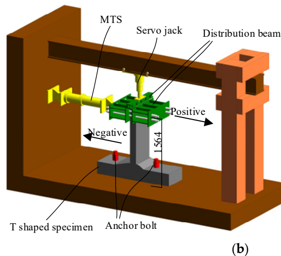
Figure 6. Diagram of the loading device. (a) L-shaped specimen; (b) T-shaped specimen.
