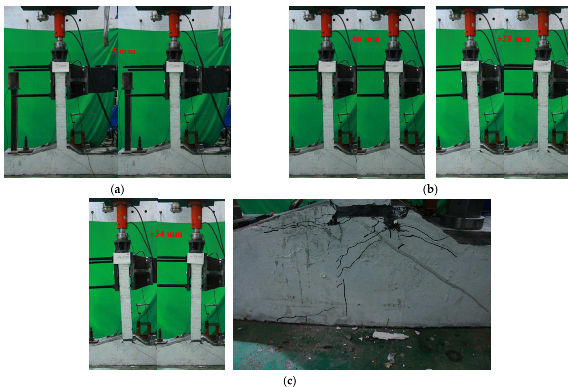
Figure 10. Test phenomenon of the T-shaped specimen. (a) Uncracked stage (5 mm); (b) cracking stage (6 to 28 mm); (c) damage phase (34 mm).
