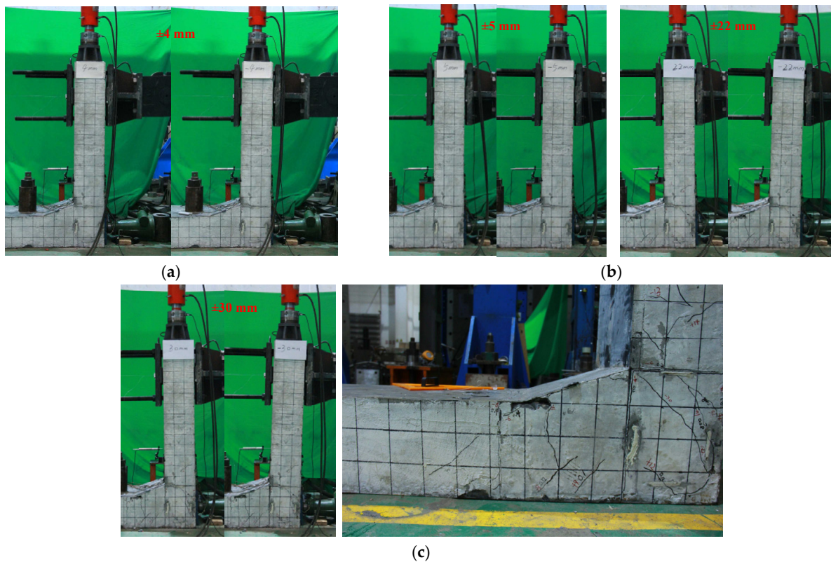
Figure 9. Test phenomena of L-shaped specimens. (a) Uncracked stage (4 mm); (b) cracking stage (5 to 22 mm); (c) damage phase (30 mm).
