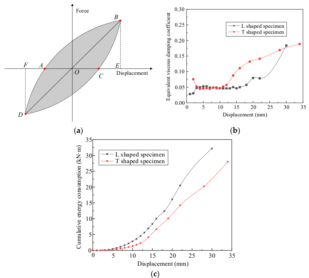
Figure 14. Specimen energy dissipation index. (a) Typical hysteresis loop; (b) equivalent viscous damping coefficient; (c) cumulative hysteresis energy consumption.
