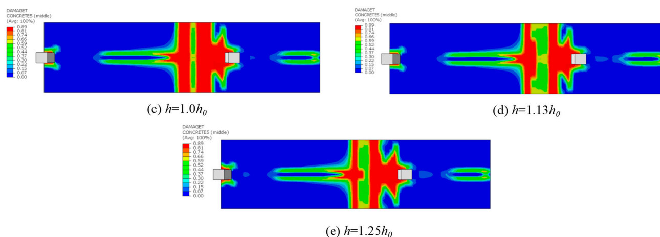
Figure 19. Concrete damage factor nephograms for the RC slab with different h values.
