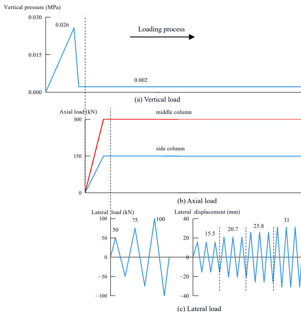
Figure 8. Loading protocol.
