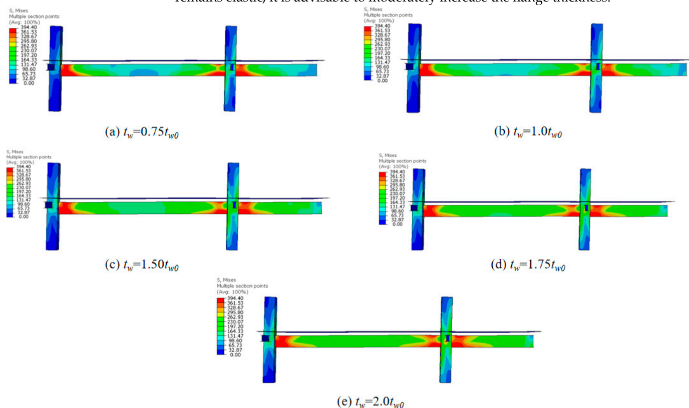
Figure 15. Stress clouds of composite frame with different t_w values.
