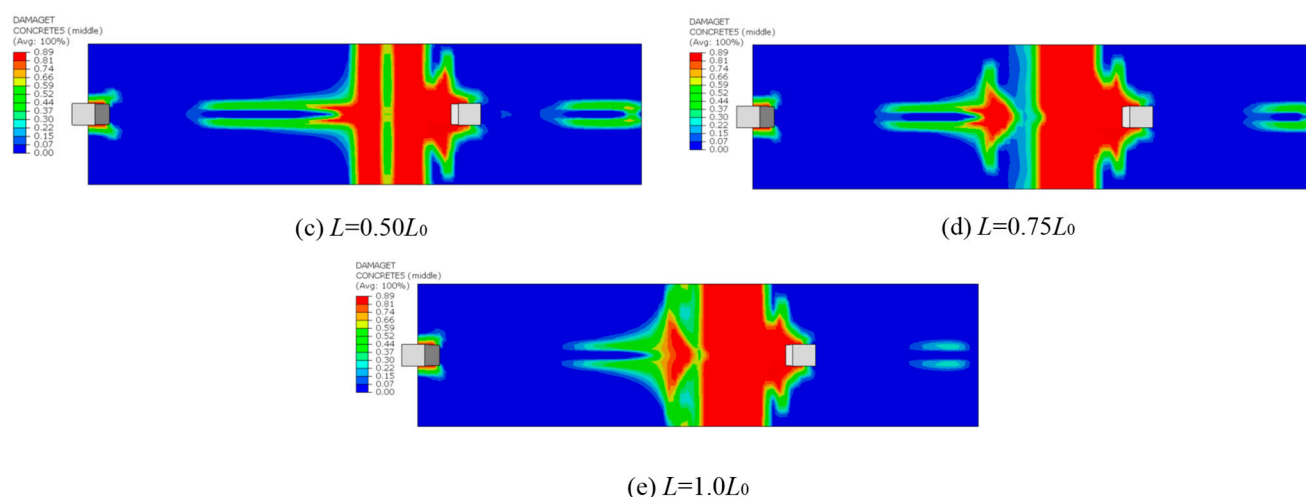
Figure 13. Concrete damage factor cloud distributions in the RC slab for varying L values.
