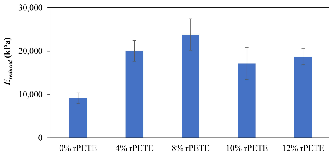
Figure 13. Results of reduced modulus for control and rPETE-modified binders.
