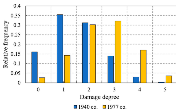
Figure 9. A comparison of the empirical damage probability histograms for medium- and high-rise RC buildings in Bucharest that were constructed before 1940 regarding the 1940 and 1977 Vrancea earthquakes.
