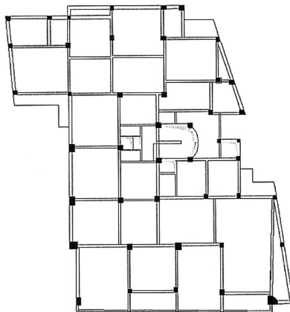
Figure 2. Typical layout of high-rise reinforced concrete structure built before 1940 in Bucharest [28].
