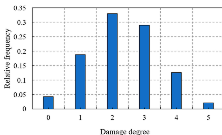
Figure 10. Empirical damage probability histograms for the unreinforced masonry structures in Barlád regarding the 1940 earthquake.
