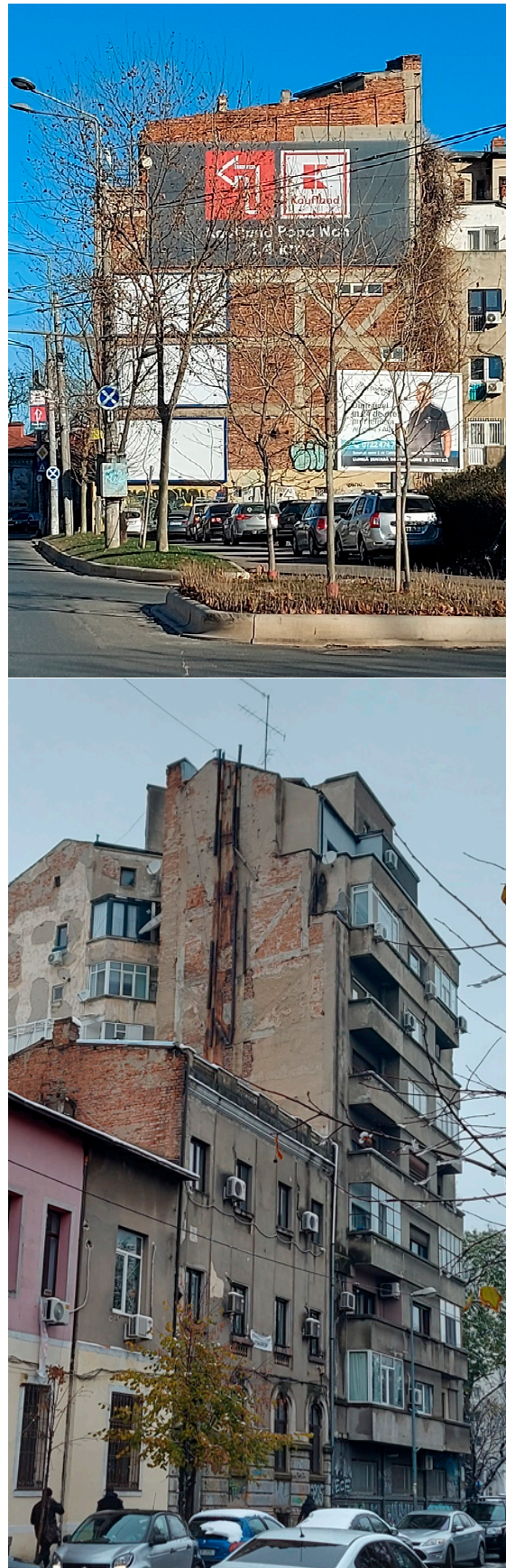
Figure 11. Examples of buildings with RC-braced frame structures that were constructed after the Vrancea 1940 earthquake.
