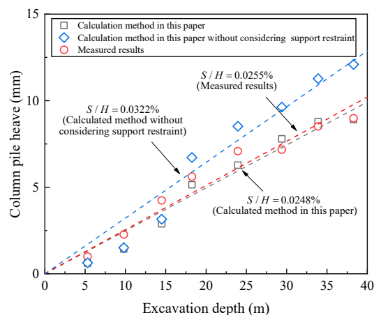
Figure 9. Comparison between calculated and measured value of upheave of column piles.
