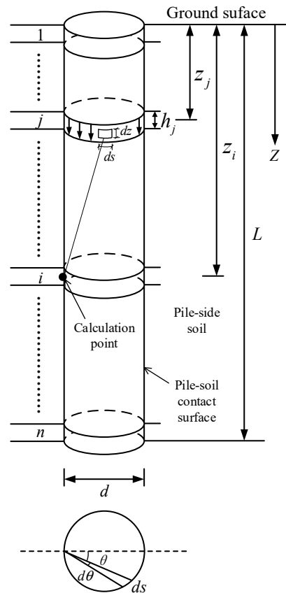
Figure 5. Sketch map of integral of soil stress under friction.
