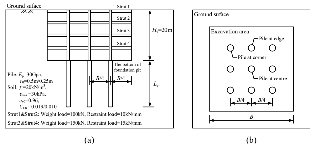
Figure 12. Calculation model for the parametric study: (a) profile of excavation; (b) plan of excavation.
