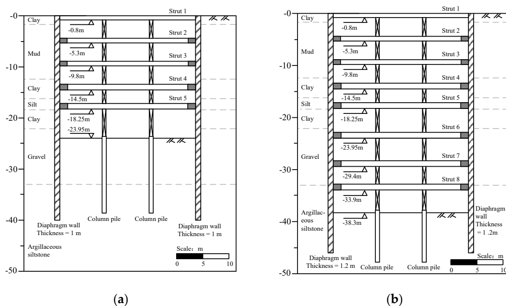
Figure 8. Section of retaining structures: (a) Section 1-1 (shallow excavation area); (b) Section 2-2 (deep excavation area).
