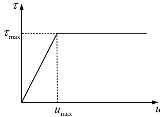
Figure 4. Model of soil resistance along the pile.
