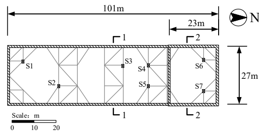
Figure 7. Excavation plan and arrangement of the monitoring points.
