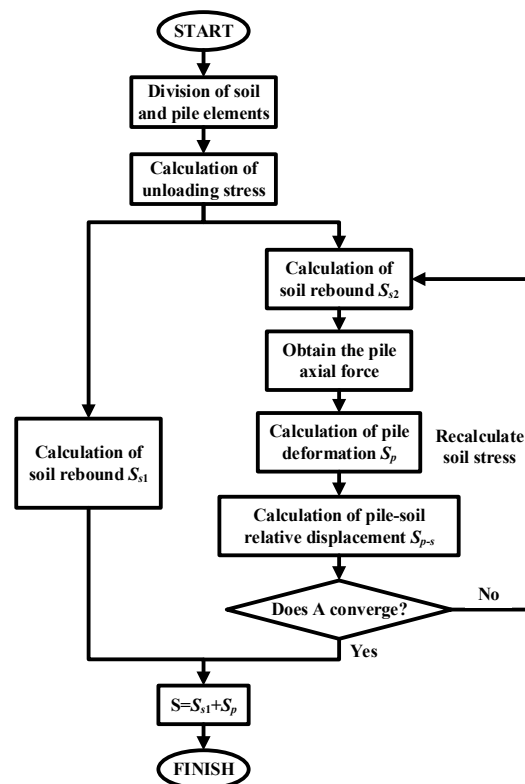
Figure 6. Flowchart of the calculation of column pile heave.
