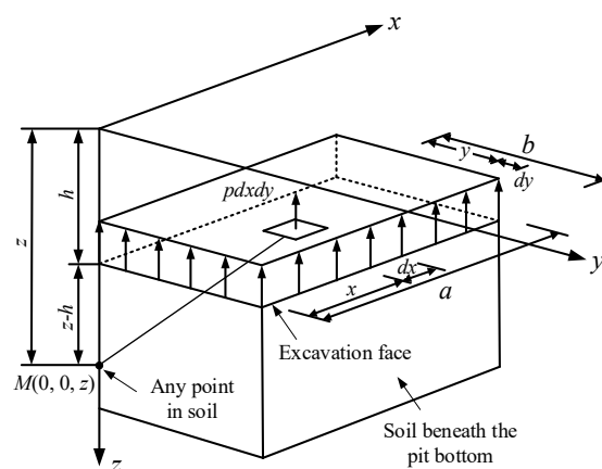
Figure 1. Calculation model of unloading stress under deep excavation.
