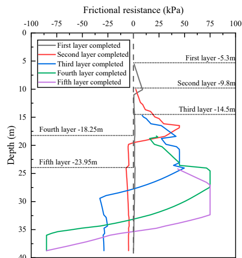
Figure 10. Variation in pile-side frictional resistance with excavation at the S5 measuring point.
