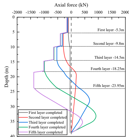
Figure 11. Variation in pile axial force with excavation at the S5 measuring point.
