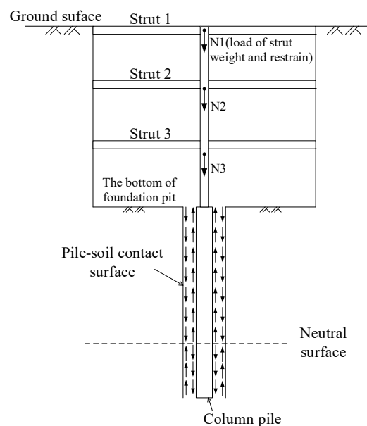
Figure 3. Simplified diagram of forces acting on a column pile in deep excavation during unloading.
