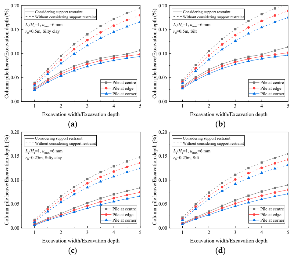
Figure 14. Effects of excavation width on column pile heave with various positions of pile: (a) r_0 = 0.5 m with silty clay; (b) r_0 = 0.5 m with silt; (c) r_0 = 0.25 m with silty clay; (d) r_0 = 0.25 m with silt.
