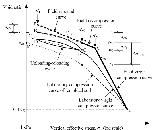
Figure 2. Method of estimating the field rebound–recompression curve based on the RRM.
