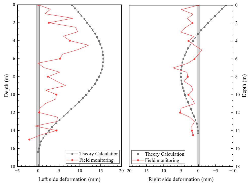
Figure 5. Comparison between in situ monitoring data and theoretical calculation of the deformation curve of the foundation pit retaining piles.
