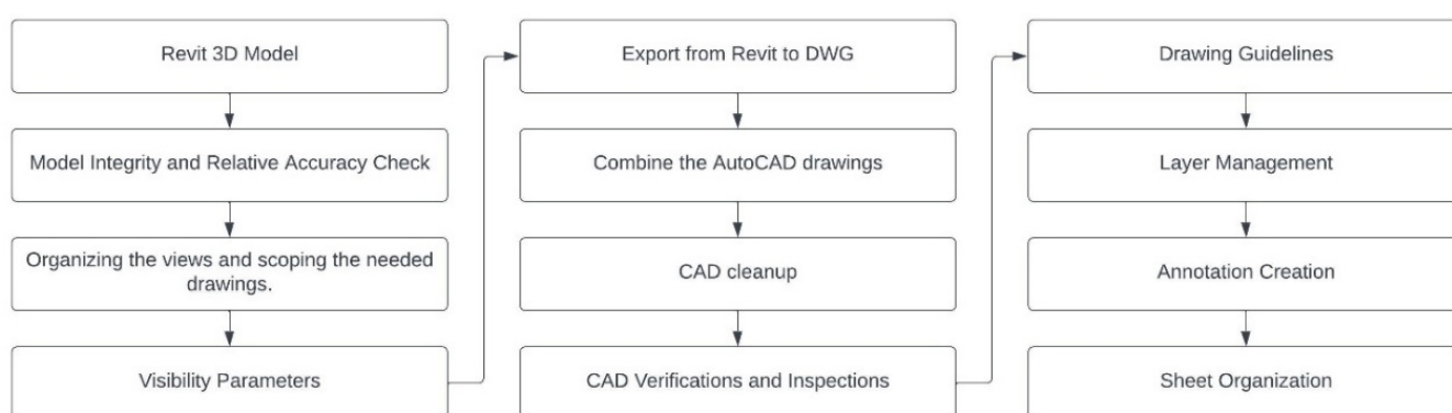
Figure 15. A process of developing the HAER drawings set.
