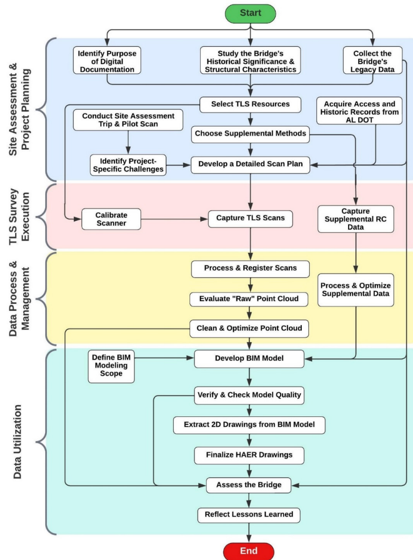
Figure 5. The process of documenting the Edmund Pettus Bridge.
