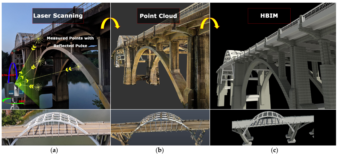
Figure 2. TLS technology and its application in heritage documentation. (a) Principle of TLS. (b) A resultant point cloud of TLS survey. (c) A Heritage BIM (HBIM) model developed using the TLS point cloud data.
