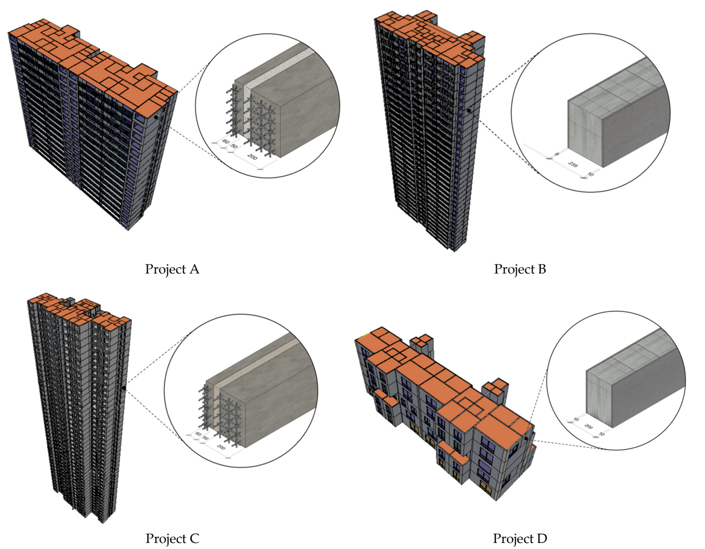
Figure 2. Building models and wall sections.
