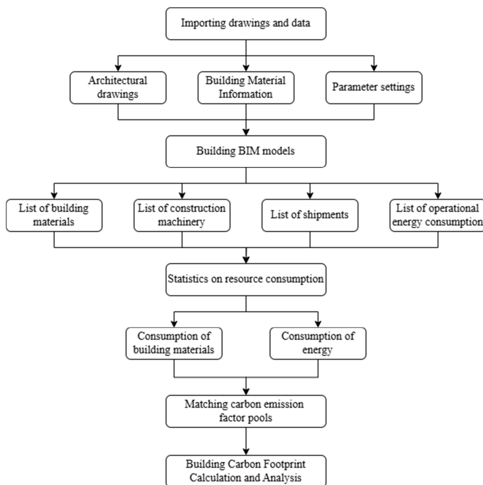
Figure 3. Algorithm logic of the carbon emission factor method based on BIM technology.
