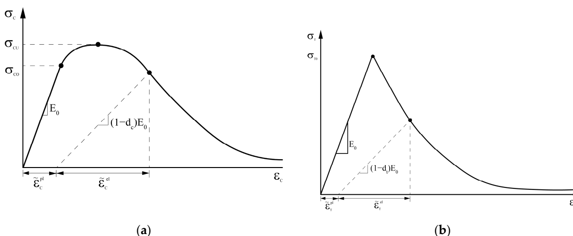
Figure 6. Graph of concrete stress–strain under uniaxial (a) compression and (b) tension (adapted from Simulia [52]).
