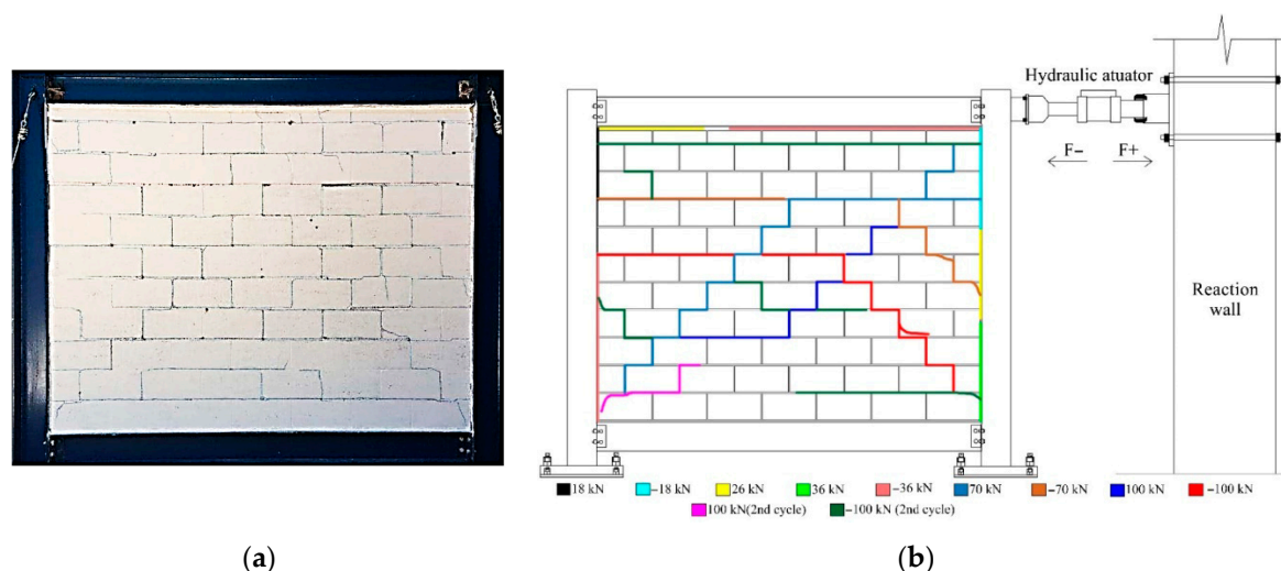
Figure 12. Cracks in the infilled frame PP-3-CE-0.5/2.0 in (a) the real image and (b) an illustration with cracks colored according to the breaking force (adapted from De Grandi [41]).
