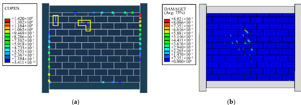
Figure 15. Results of applying the first 70 kN load to the right of (a) opening in the contacts (COPEN variable), and (b) masonry damage (displacement magnification: 1×).
