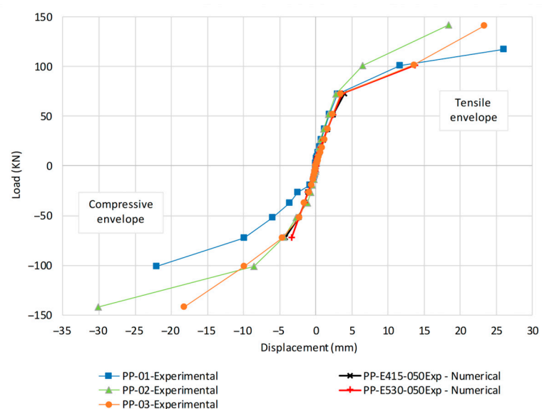
Figure 19. Comparison between the results of the tested frames and the numerical models. Note: The abscissa represents the displacements at the top of the frame (corresponding to point RP-13 in
