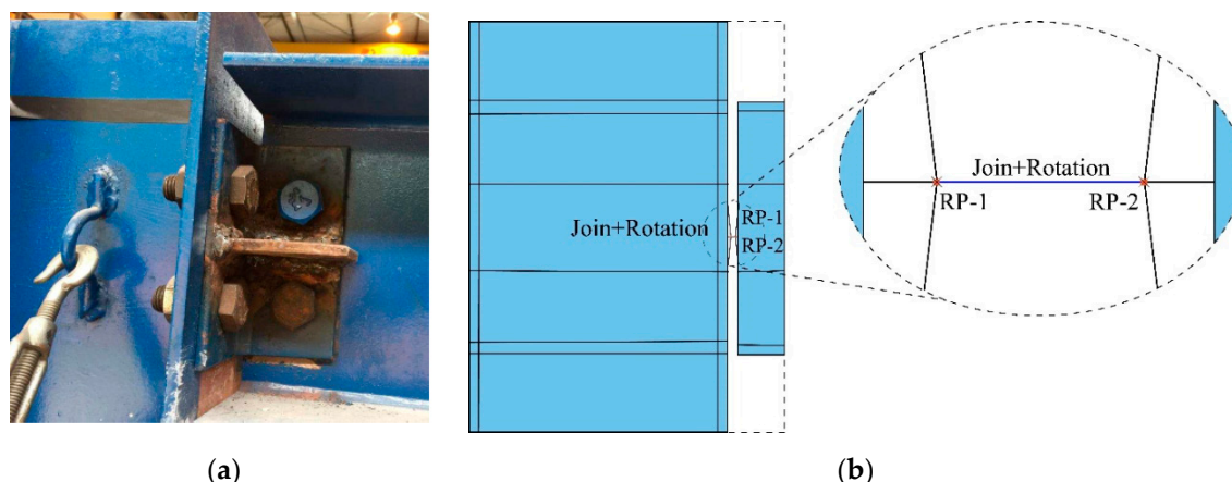
Figure 4. Connection between the steel I-profiles of the frame: (a) experimental and (b) numerical.
