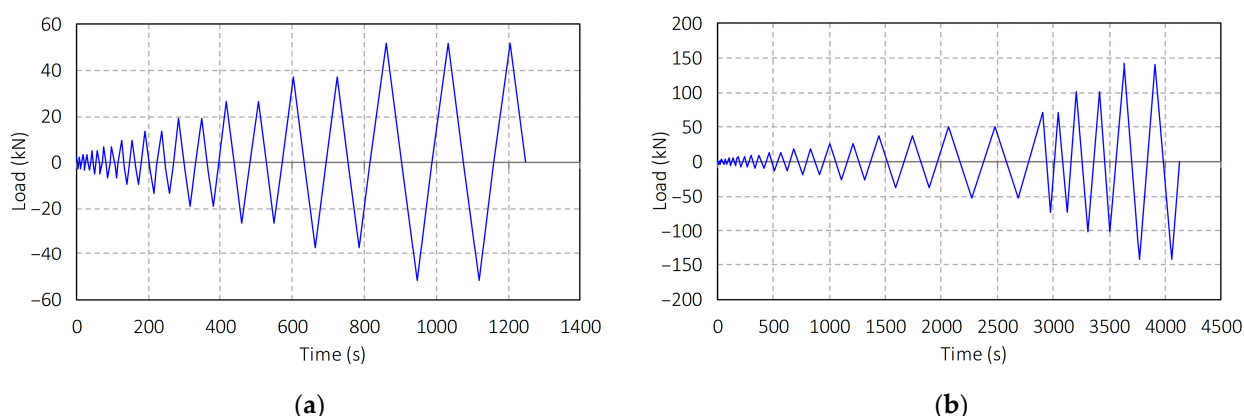
Figure 7. Load applied to the numerical model of (a) empty frame and (b) infilled frame.
