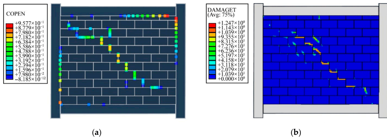
Figure 16. Results after the second load of 70 kN with (a) contact spacing (COPEN variable) and (b) damage to the blocks (displacement magnification: 1 \times ).
