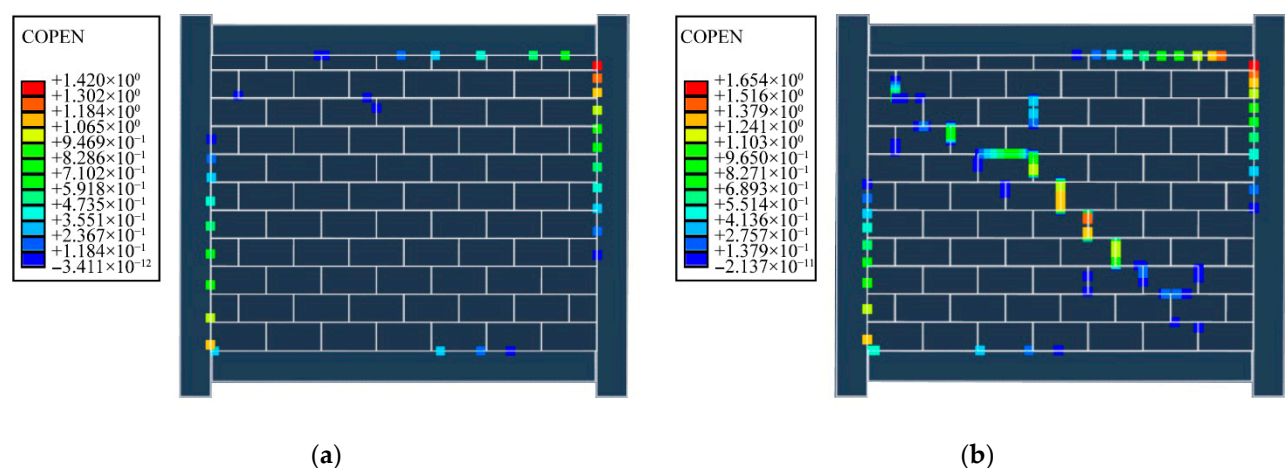
Figure 22. Separation between blocks obtained in numerical models (a) with friction and (b) without friction at the first load of 70 kN to the right (displacement magnification: 1×).
