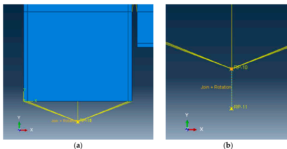
Figure 5. Semi-rigid connection of the pillar base using the Join + Rotation connector: (a) overall view of the connection model; (b) enlarged detail highlighting the connection region for improved visualization.
