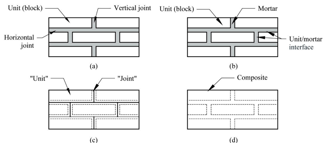
Figure 1. Masonry modeling approaches: (a) real masonry sample; (b) detailed micro-modeling; (c) simplified micro-modeling; (d) macro-modeling (adapted from Lourenço [48]).
