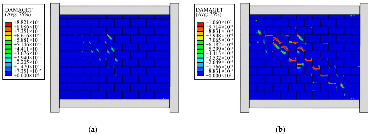
Figure 21. Damage assessed by numerical models (a) with friction and (b) without friction at the first load of 70 kN to the right (displacement magnification: 1×).
