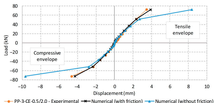
Figure 20. Experimental and numerical envelopes with and without friction.
