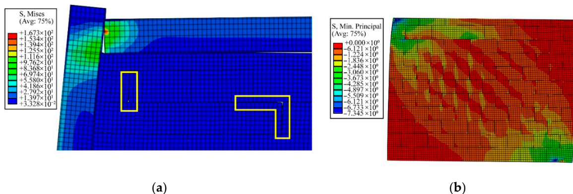
Figure 14. Displacement of the frame to the left side resulting in (a) separation of the units and (b) interference with the compression rod ( \sigma_{min} ) (displacement magnification: 40×).
