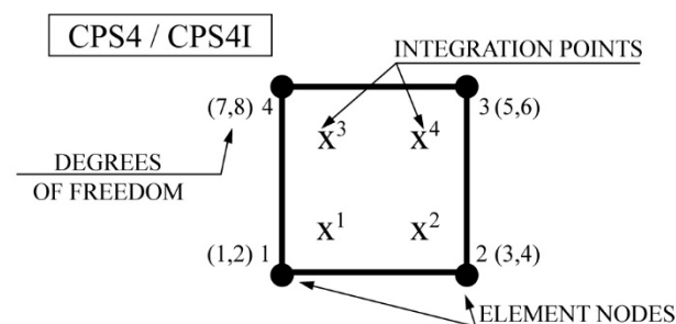
Figure 9. Diagram of the CPS4 element (adapted from Kawecki and Podgórski [66]).
