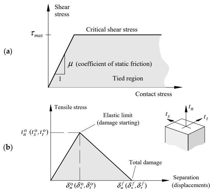
Figure 3. Criteria of (a) friction limited by a critical shear stress, and (b) cohesion at surfaces subject to separation (adapted from Simulia [52]).
