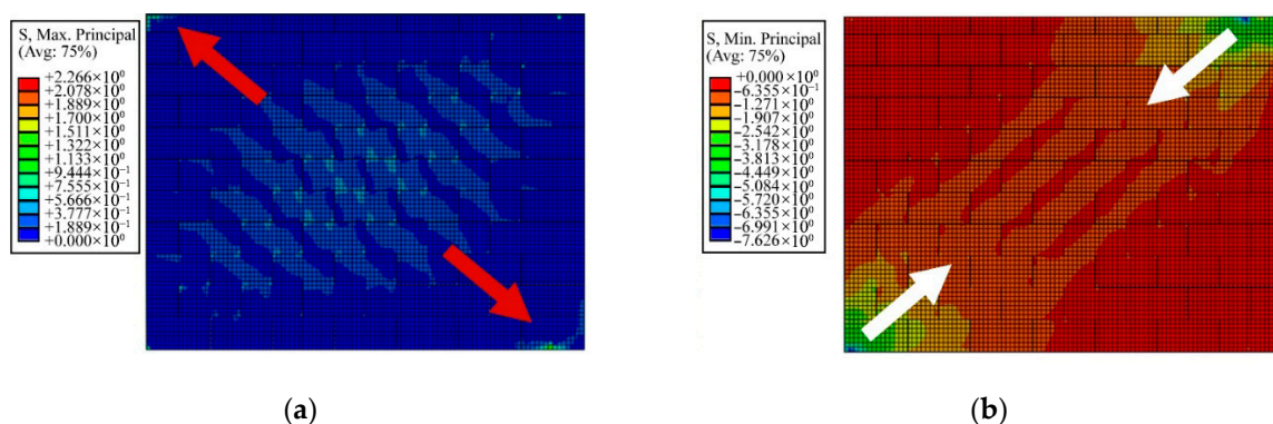
Figure 13. Displacement of the frame to the left with the formation of (a) tension struts ( \sigma_{max} ) and (b) compression struts ( \sigma_{min} ) (displacement magnification: 1 \times ).
