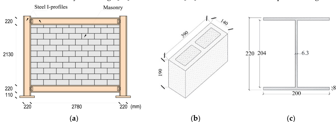
Figure 2. Geometric characteristics (a) of the studied steel frame, (b) the concrete blocks (in mm), and (c) of the steel I profile (in mm) adapted from Alvarenga [23].
