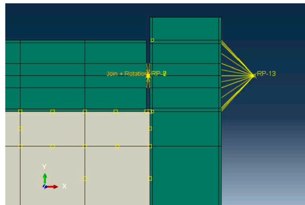
Figure 8. Kinematic coupling adopted for load application.
