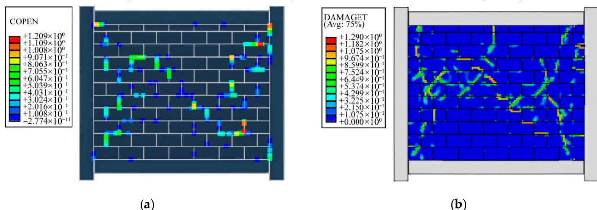
Figure 17. Results after all 70 kN cycles with (a) contact spacing (COPEN variable) and (b) damage to the blocks (displacement magnification: 1 \times ).
