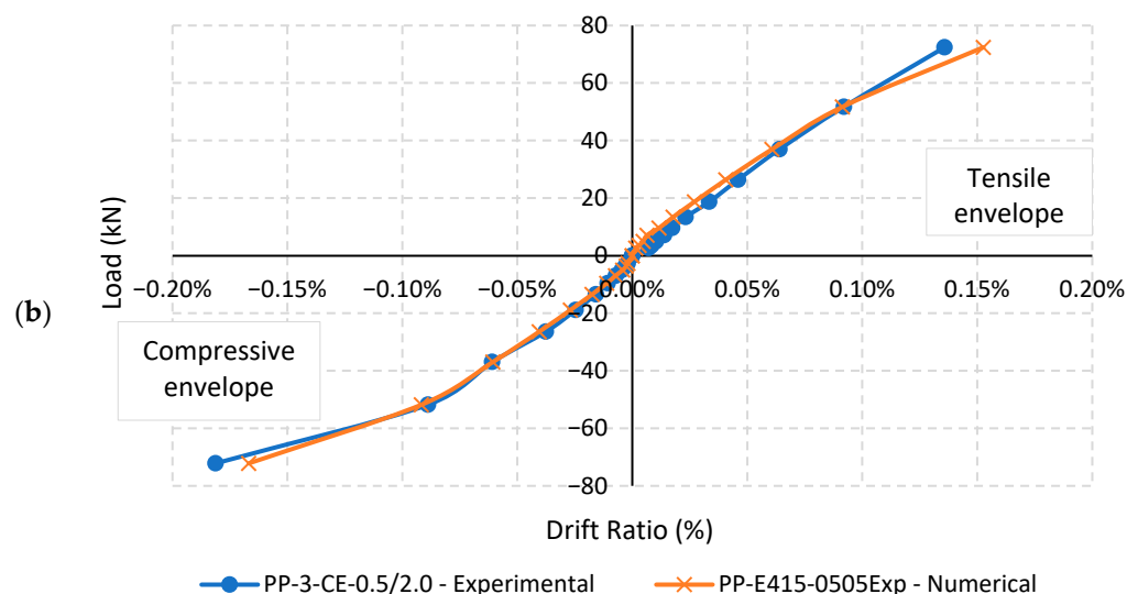
Figure 18. Load envelope obtained by the numerical model: (a) displacement (mm) and (b) drift ratio (%). Note: The abscissa (a) represents the displacements at the top of the frame (corresponding to point RP-13 in the numerical model), while the abscissa (b) corresponds to the drift ratio (%). Each ‘×’ and ‘•’ symbol represents the peak load–displacement point of the first cycle for each load step. The sign convention for force and displacement follows the scheme illustrated in Figure 12.
