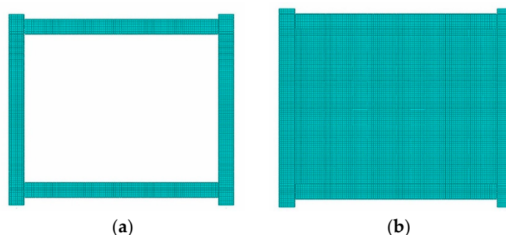
Figure 10. Finite element mesh of the models: (a) empty frame and (b) infilled frame.
