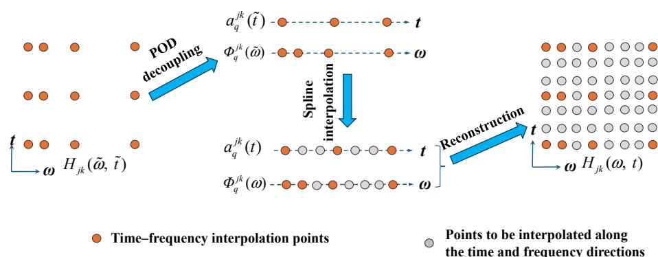
Figure 1. Schematic illustration of the decoupling, interpolation, and reconstruction procedure.
