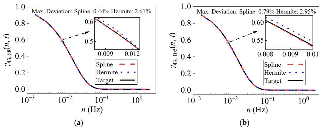
Figure 7. Comparison of coherence functions at t = 300 s: (a) Point 43 and Point 88; (b) Point 43 and Point 105.
