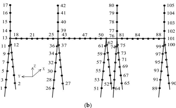
Figure 3. Three-span frame lightning-rod structure [36]: (a) Structural configuration; (b) Layout of simulation points.
