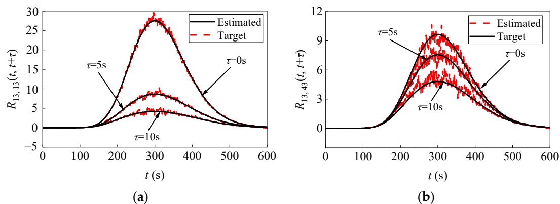
Figure 6. Validation of correlation functions: (a) Autocorrelation at Point 13; (b) Cross-correlation between Point 13 and Point 43.
