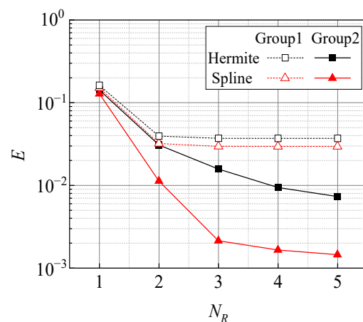
Figure 9. Comparison of simulation errors obtained by the two interpolation methods.
