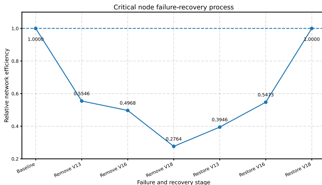
Figure 9. Critical-node failure–recovery resilience curve.
