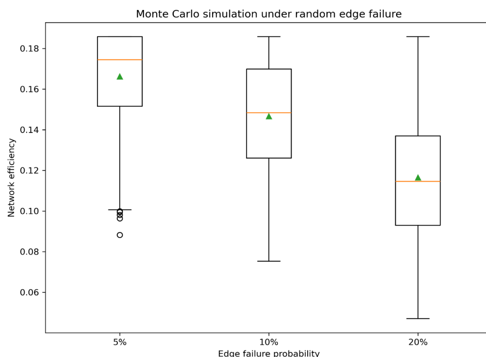
Figure 6. Network efficiency distribution under random edge failure.
