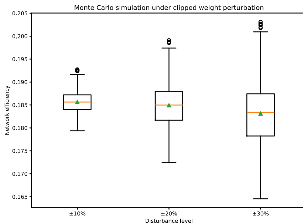
Figure 5. Network efficiency distribution under edge-weight perturbation.
