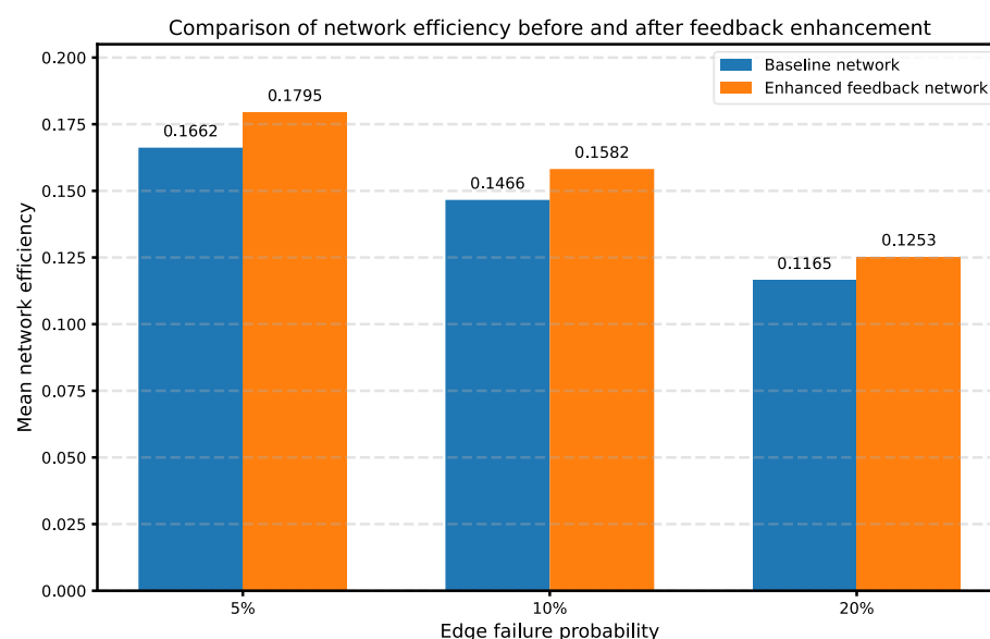
Figure 7. Comparison of network efficiency before and after feedback enhancement.
