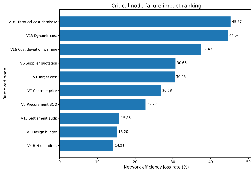
Figure 3. Ranking of critical node failure impacts.
