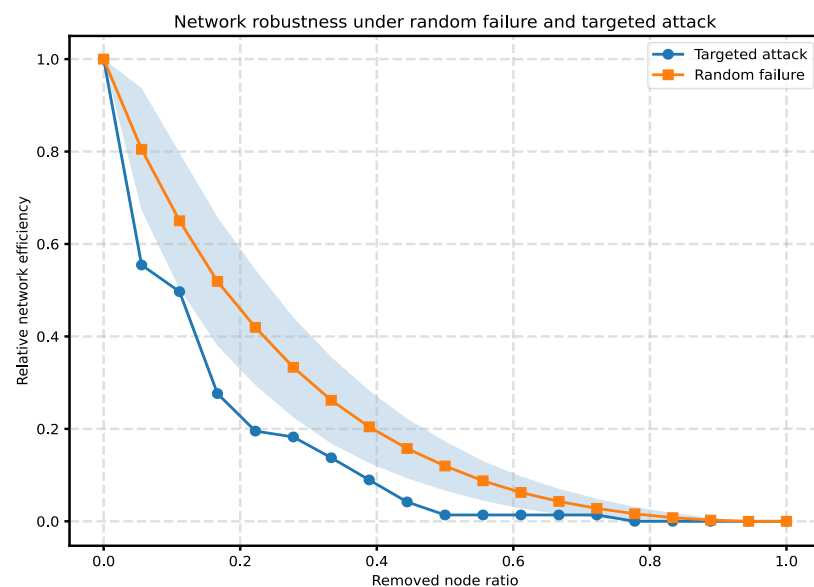
Figure 8. Network robustness under random failure and targeted attack.
