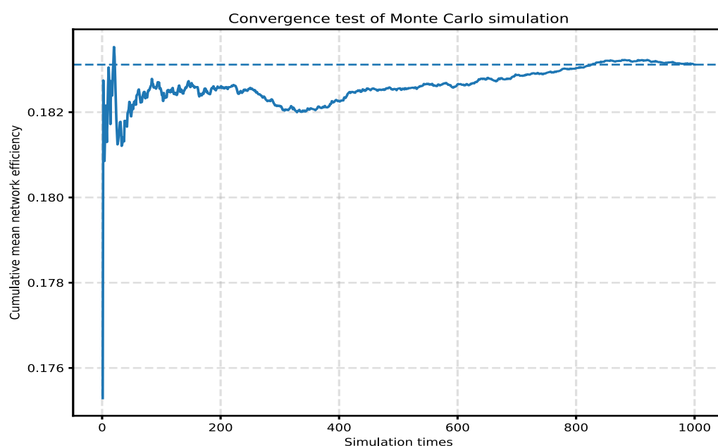
Figure 4. Convergence test of the Monte Carlo simulation.
