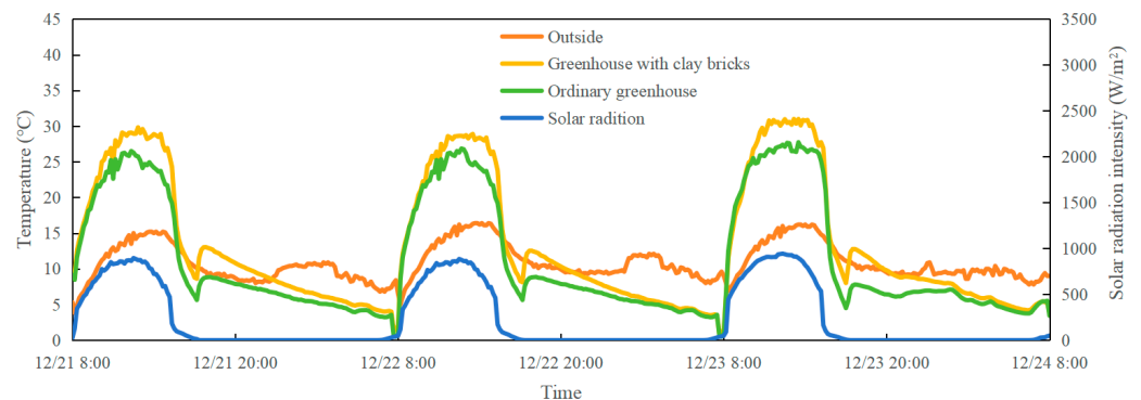
Figure 9. Temperature regulation performance: case 3.
