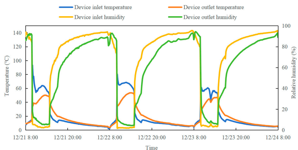
Figure 16. Device inlet and outlet air temperature and humidity regulation performance: case 3.
