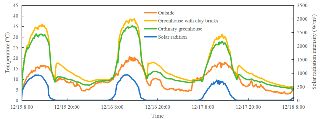
Figure 7. Temperature regulation performance: case 1.
