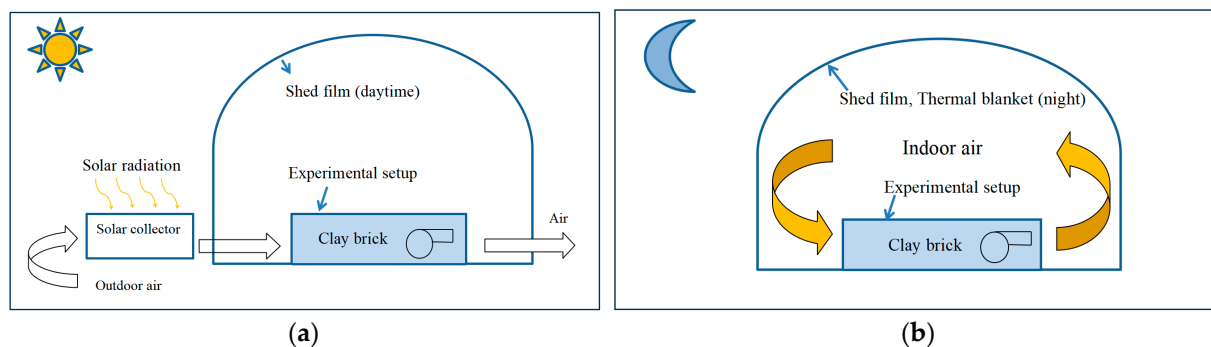
Figure 4. Experimental system's working principle: (a) Day; (b) Night.
