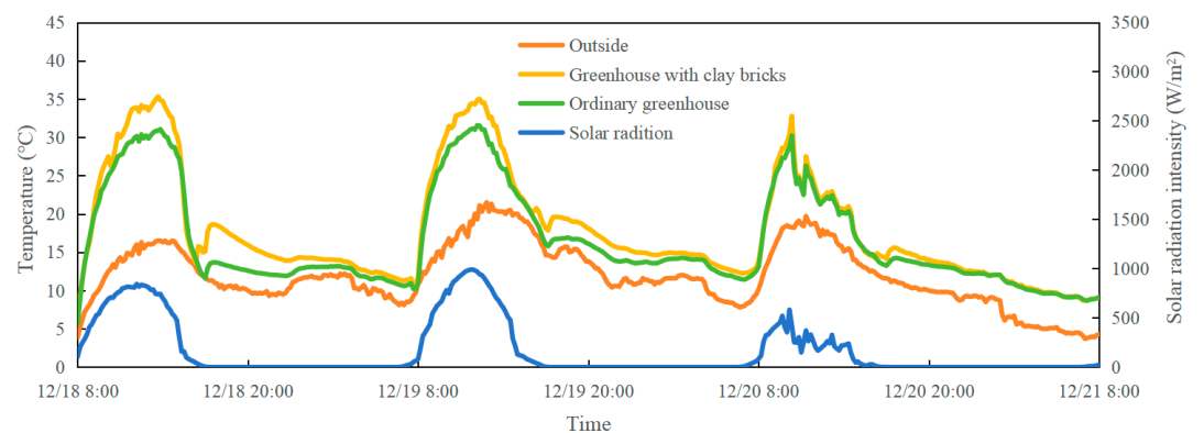
Figure 8. Temperature regulation performance: case 2.
