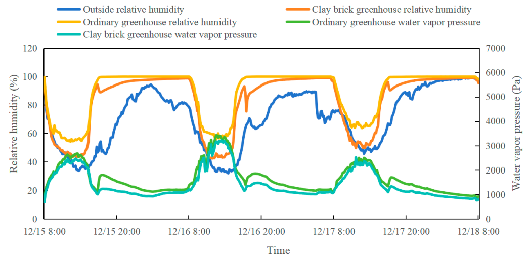
Figure 11. Humidity regulation performance: case 1.
