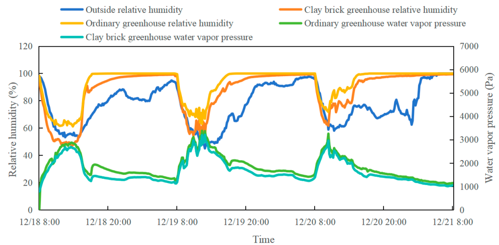
Figure 12. Humidity regulation performance: case 2.
