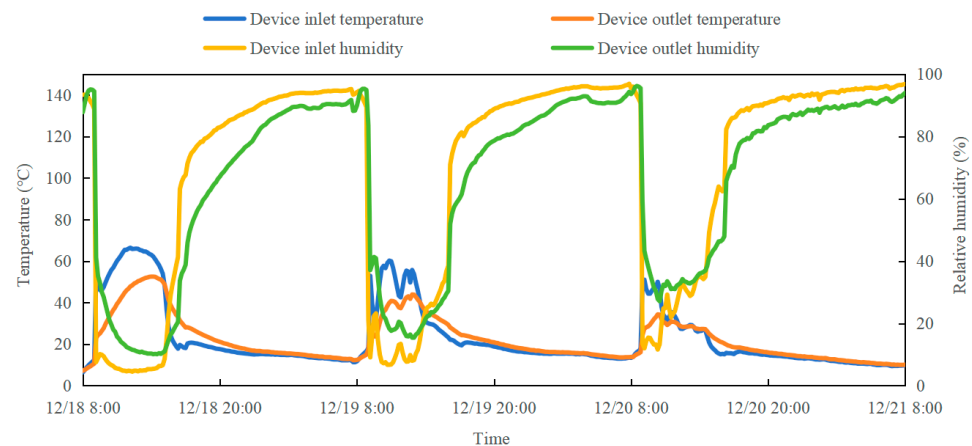
Figure 15. Device inlet and outlet air temperature and humidity regulation performance: case 2.
