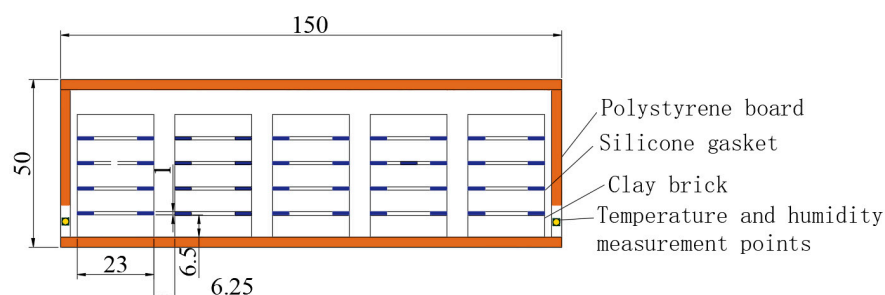
Figure 5. Temperature and humidity measurement point layout.
