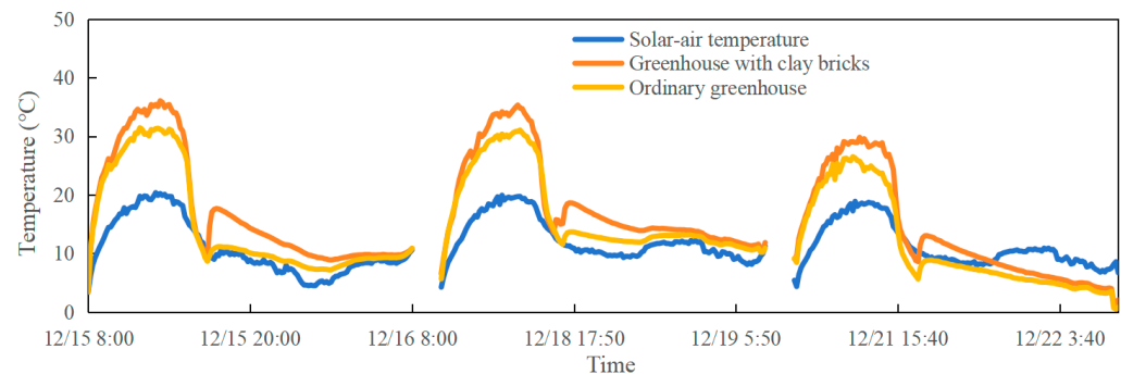
Figure 10. Heat storage duration performance.
