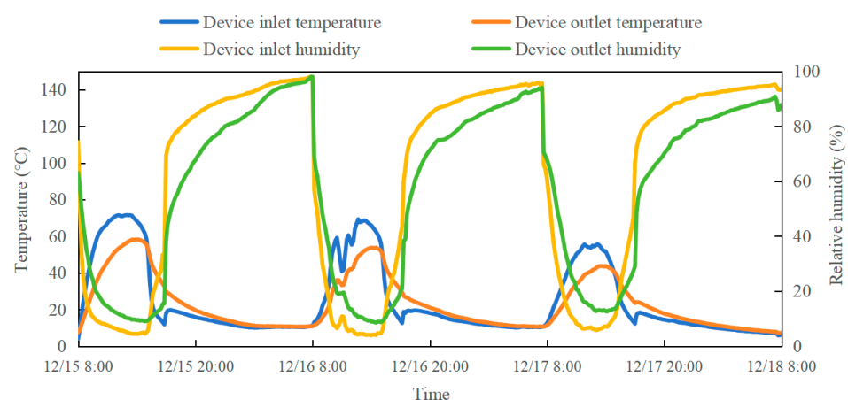
Figure 14. Device inlet and outlet air temperature and humidity regulation performance: case 1.
