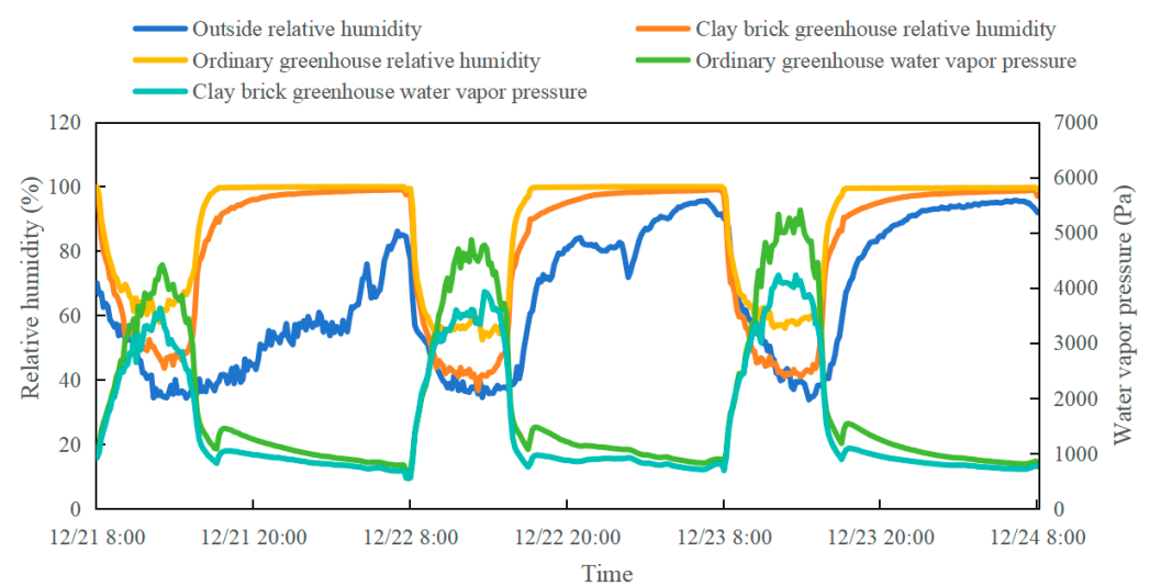
Figure 13. Humidity regulation performance: case 3.
