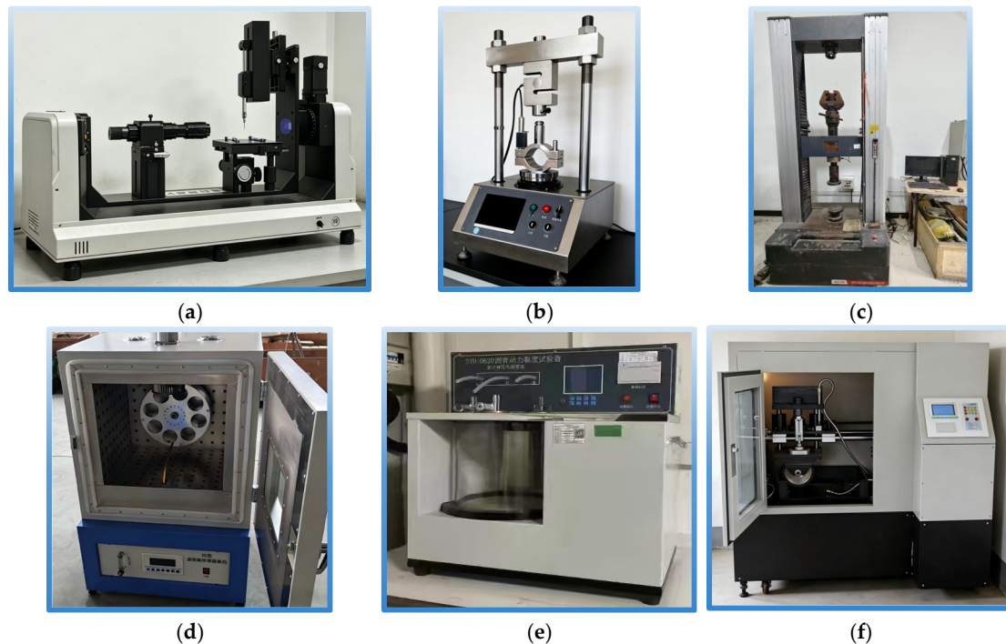
Figure 4. (a) Contact-angle meter; (b) Marshall stability tester; (c) electronic universal testing machine; (d) rolling thin-film oven; (e) asphalt dynamic viscosity tester; and (f) rutting tester.
