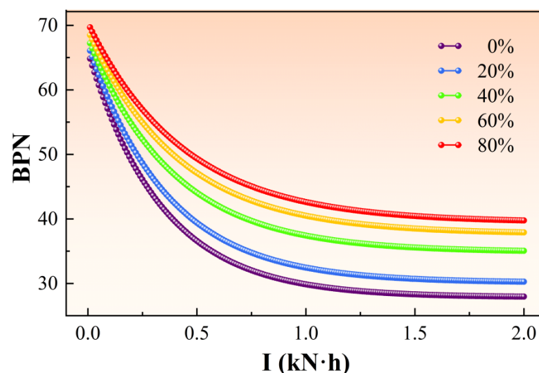
Figure 13. Fitted curves of the skid-resistance degradation model based on I .
