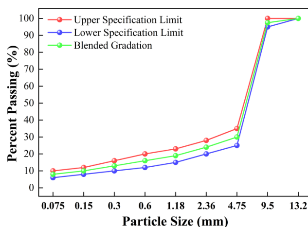
Figure 3. Gradation range of the SAC-10 ultra-thin wearing course.
