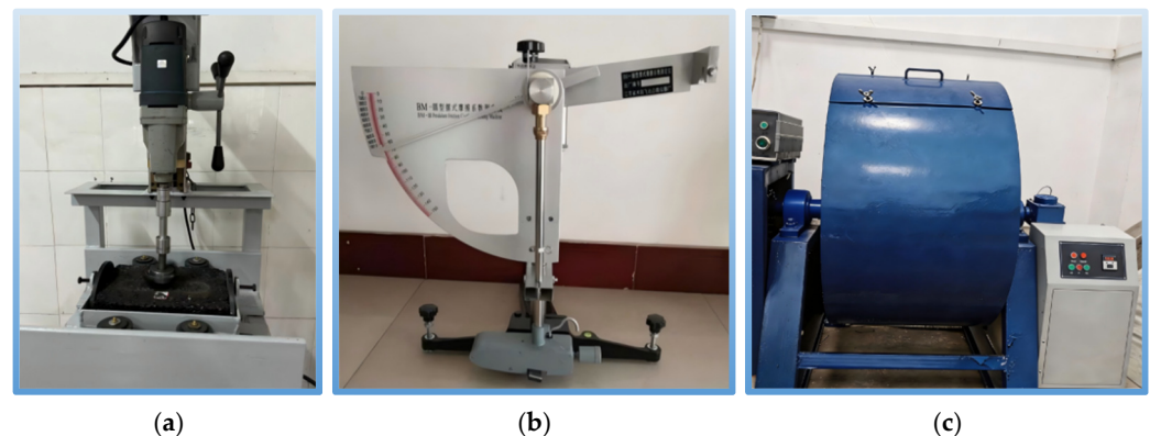
Figure 5. (a) Accelerated abrasion tester; (b) pendulum friction coefficient tester; and (c) Cantabro particle-loss tester.
