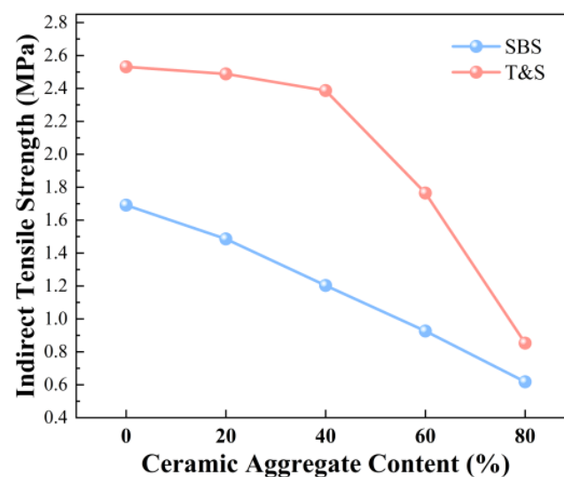
Figure 11. Effect of ceramic aggregate content on the indirect tensile strength of asphalt mixtures.
