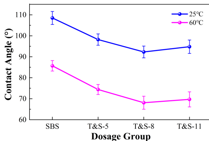
Figure 7. Contact angle between different asphalt binders and ceramic aggregates.
