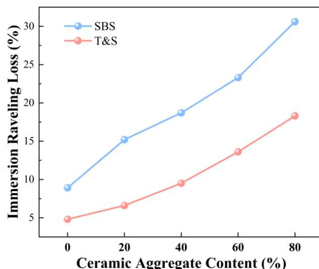
Figure 14. Immersion Cantabro particle-loss ratios of mixtures with different ceramic aggregate contents.
