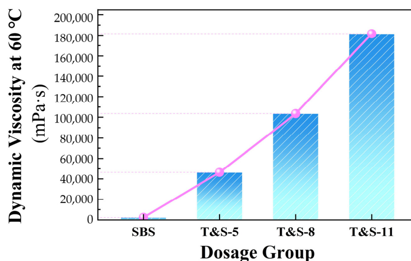
Figure 8. Test results of 60 °C dynamic viscosity.
