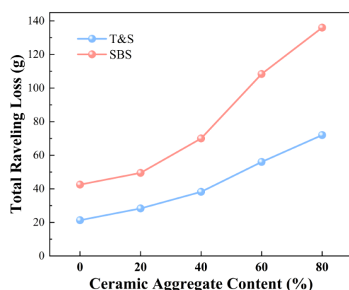
Figure 16. Total torsional particle loss of different modified asphalt mixtures at various ceramic aggregate contents.
