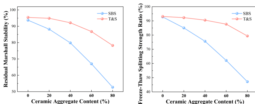
Figure 10. Effect of ceramic aggregate content on the moisture stability of asphalt mixtures.
