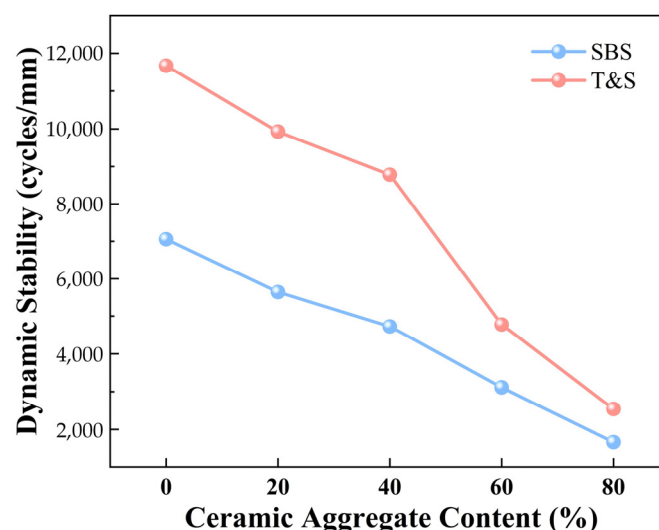
Figure 9. Effect of ceramic aggregate content on the dynamic stability of asphalt mixtures.
