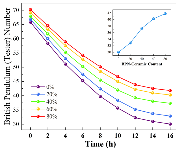
Figure 12. Variation in BPN of mixtures with different ceramic aggregate contents as a function of abrasion time.
