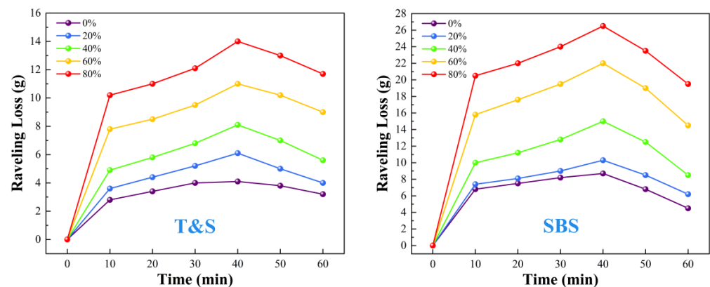
Figure 15. Time-history curves of torsional particle-loss mass for mixtures with different ceramic aggregate contents.
