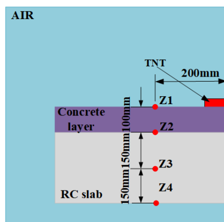
Figure 9. Layout of measuring points.
