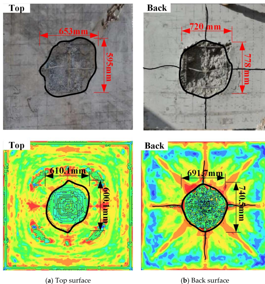
Figure 4. Comparison of experimental and numerical results.
