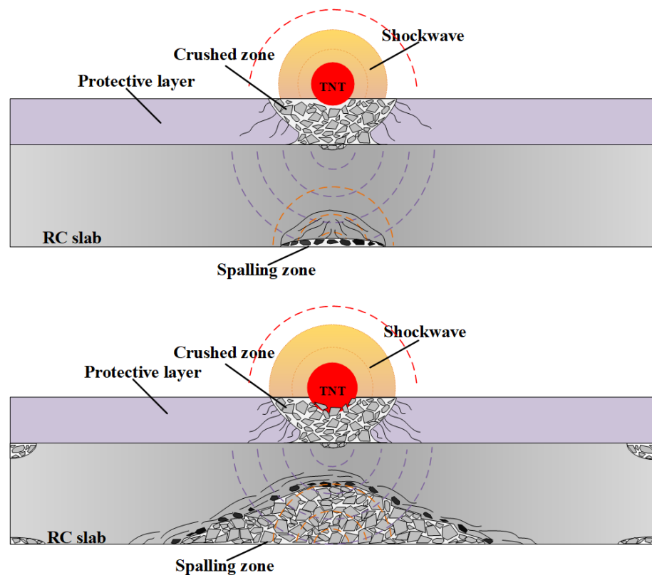
Figure 14. Damage evolution mechanism of different protection schemes.
