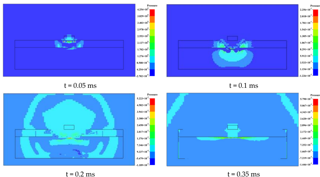
Figure 8. Pressure field distribution of T-1 scheme.
