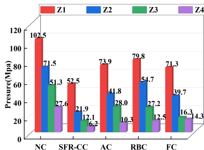
Figure 11. Peak pressure of various reinforcement schemes.
