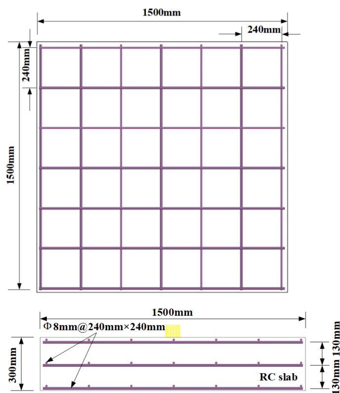
Figure 1. Arrangement of structural dimensions in the test.
