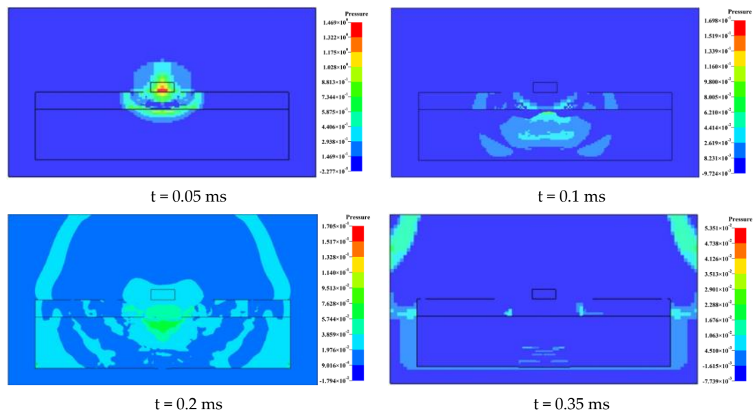
Figure 7. Pressure field distribution of NC scheme.
