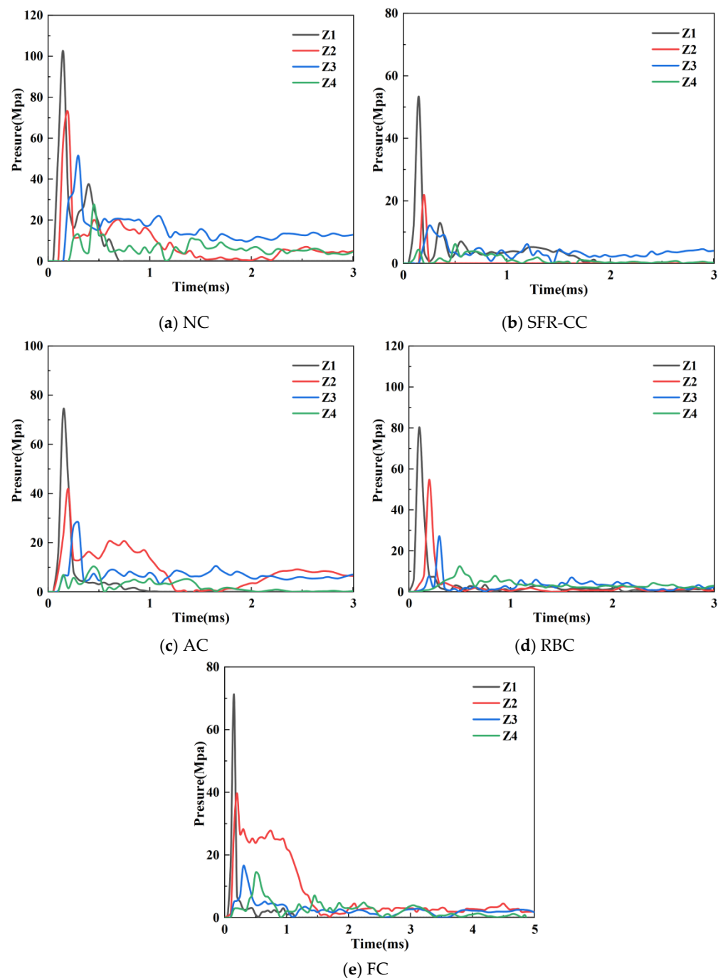
Figure 10. Pressure curves of various reinforcement schemes.
