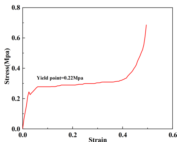
Figure 5. Stress–strain curve of FC.
