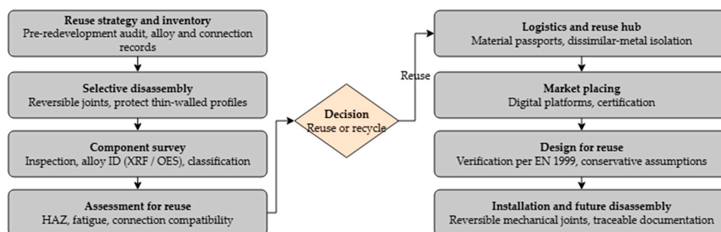
Figure 3. Proposed reuse pathway for structural aluminium members.
