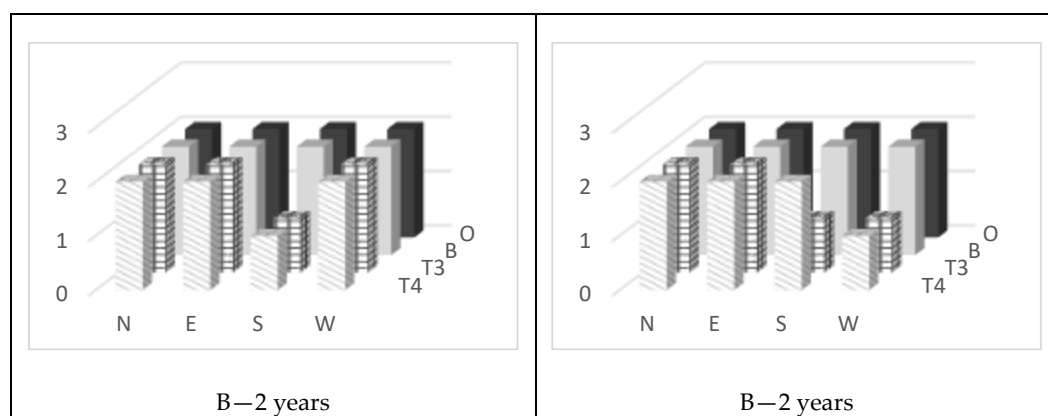
Figure 11. Visual classification results for wood degradation by biotic agents—Parameter B.
