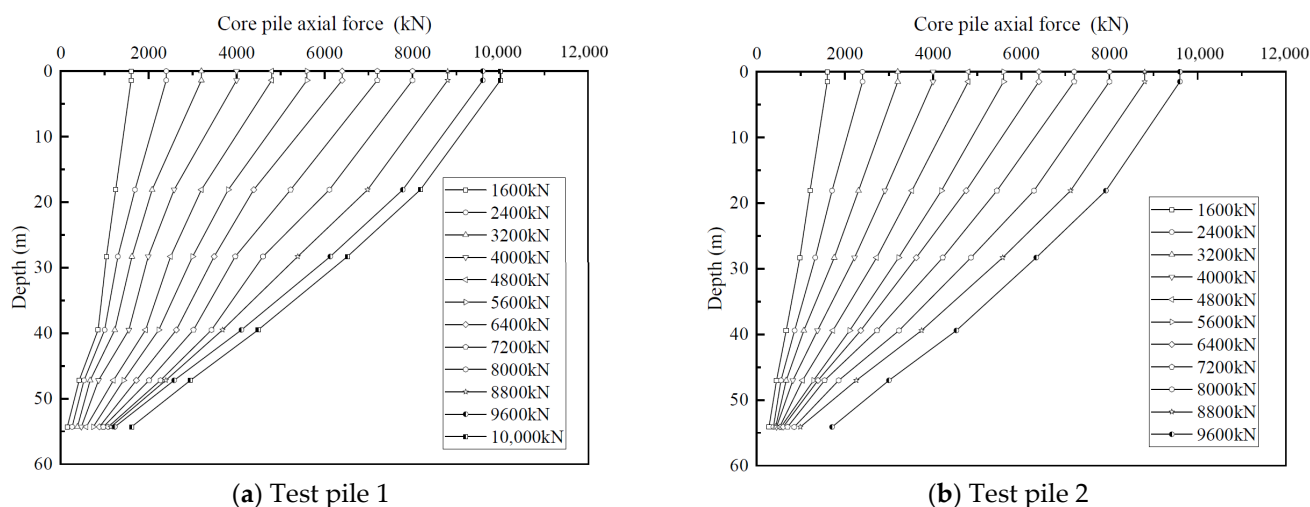
Figure 5. Core pile axial force.
