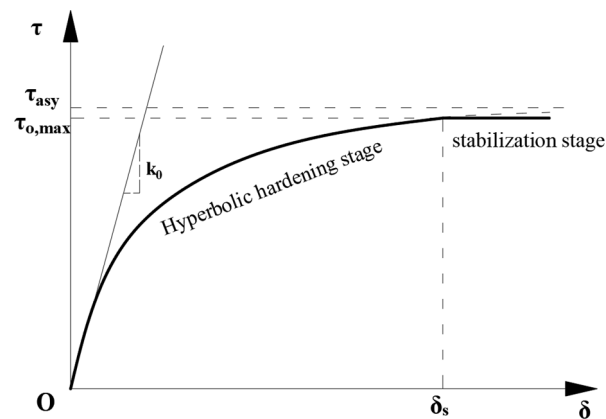
Figure 9. Constitutive model for shaft resistance of PGP pile.
