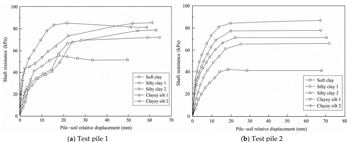
Figure 7. Curves of shaft resistance varying with pile–soil relative displacement.
