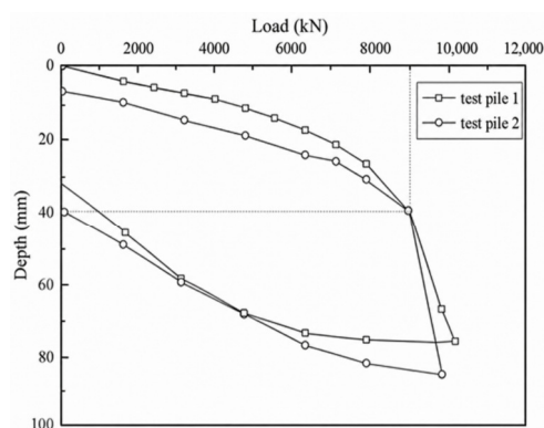
Figure 4. Load–displacement curves of the test piles.
