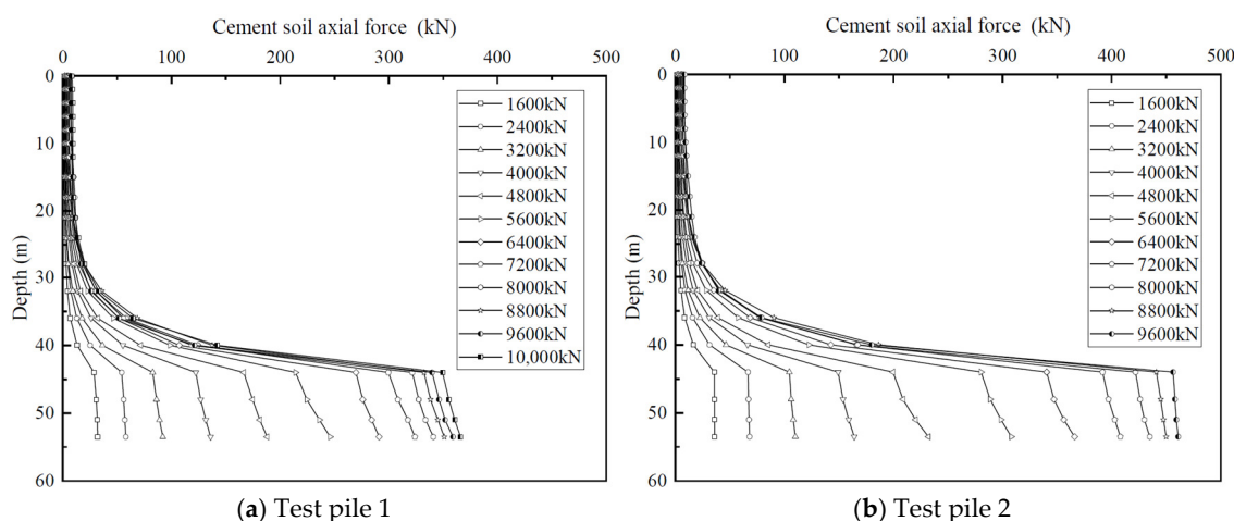
Figure 6. Cement soil axial force.
