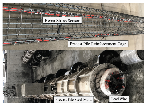
Figure 2. Precast pile fabrication and rebar stress sensor installation.
