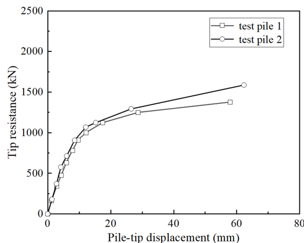
Figure 8. Tip resistance of the test piles.
