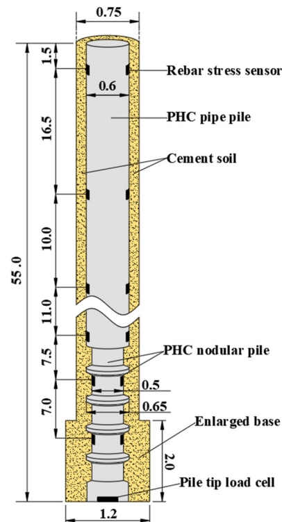
Figure 1. Schematic of the test pile (unit: m).
